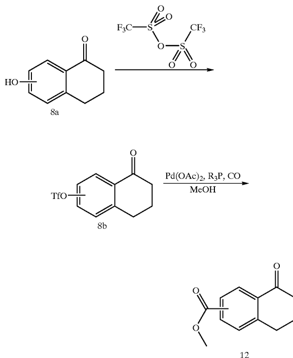
SCHEME VII
