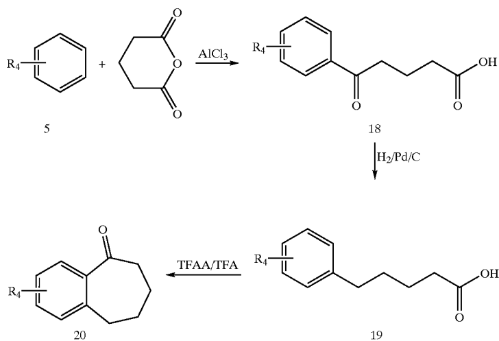
SCHEME X
