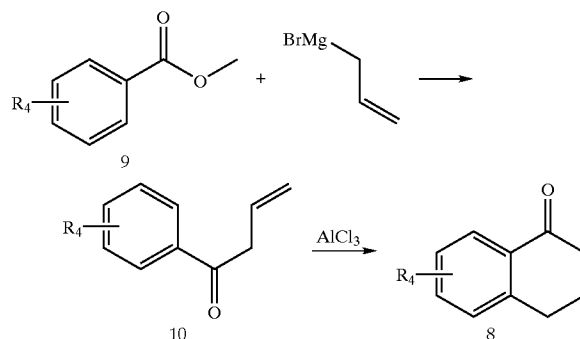
SCHEME IV
