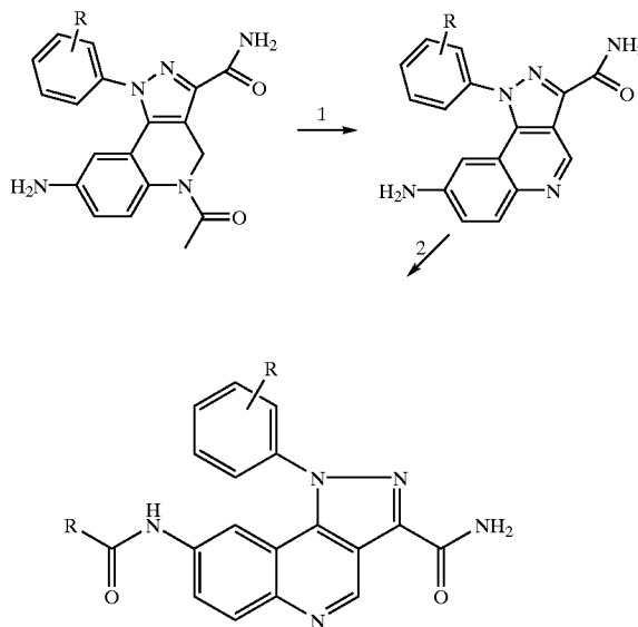
Scheme XII
