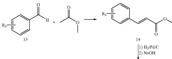
SCHEME VIII
