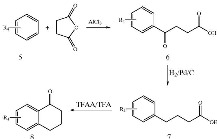
SCHEME III
