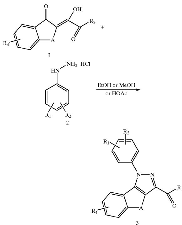
SCHEME I
