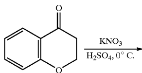
SCHEME XIII
