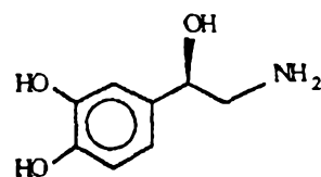
Norepinephrine
