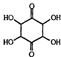
Tetrahydroxybenzoquinone
