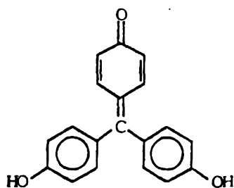
Aurin
