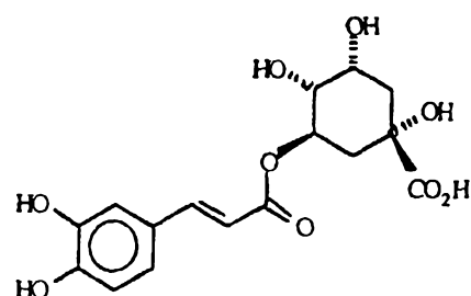
Chlorogenic Acid
