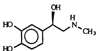
Epinephrine
