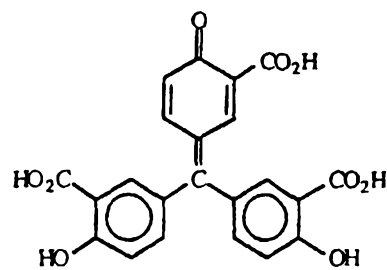
Aurintricarboxylic Acid
