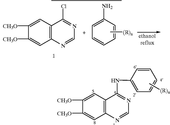
Scheme 2 Synthesis of JAK3 inhibitors.
