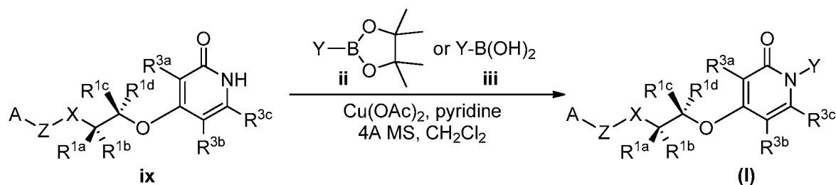
Scheme 11. Synthesis of the compound of formula (I)
