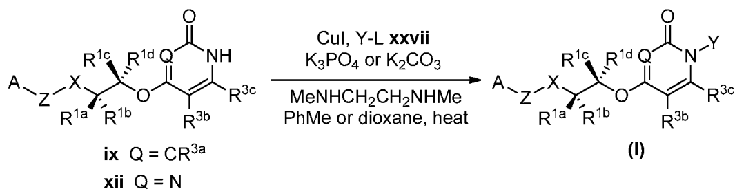
Scheme 9. Synthesis of the compound of formula (I)
