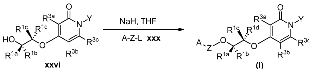
Scheme 15. Synthesis of the compound of formula (I)
