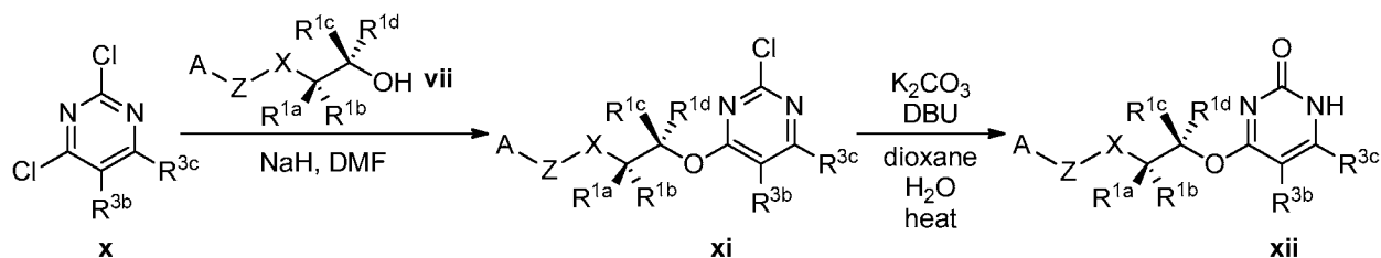
Scheme 3. Synthesis of intermediate xii
