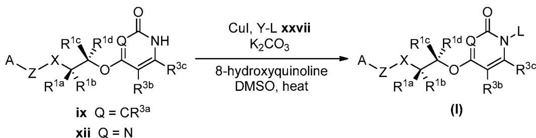
Scheme 10. Synthesis of the compound of formula (I)
