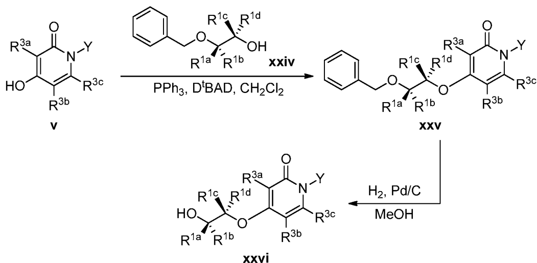
Scheme 7. Synthesis of intermediate xxvi
