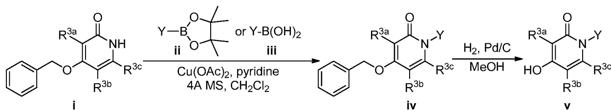
Scheme 1. Synthesis of intermediate v
