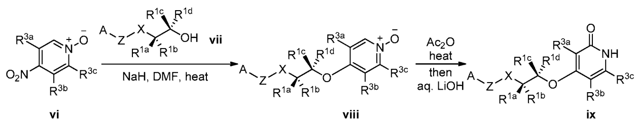
Scheme 2. Synthesis of intermediate ix
