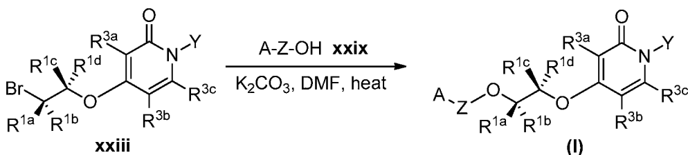
Scheme 14. Synthesis of the compound of formula (I)
