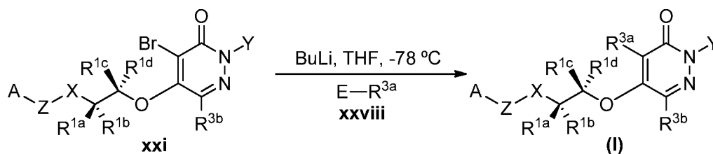
Scheme 13. Synthesis of the compound of formula (I)
