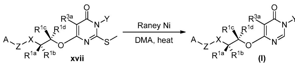
Scheme 12. Synthesis of the compound of formula (I)
