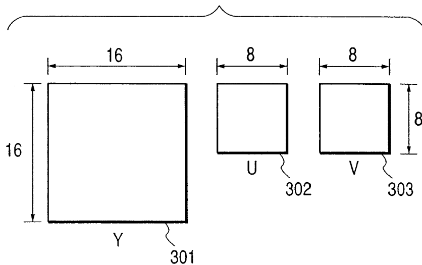
FIG. 3 (PRIOR ART)
