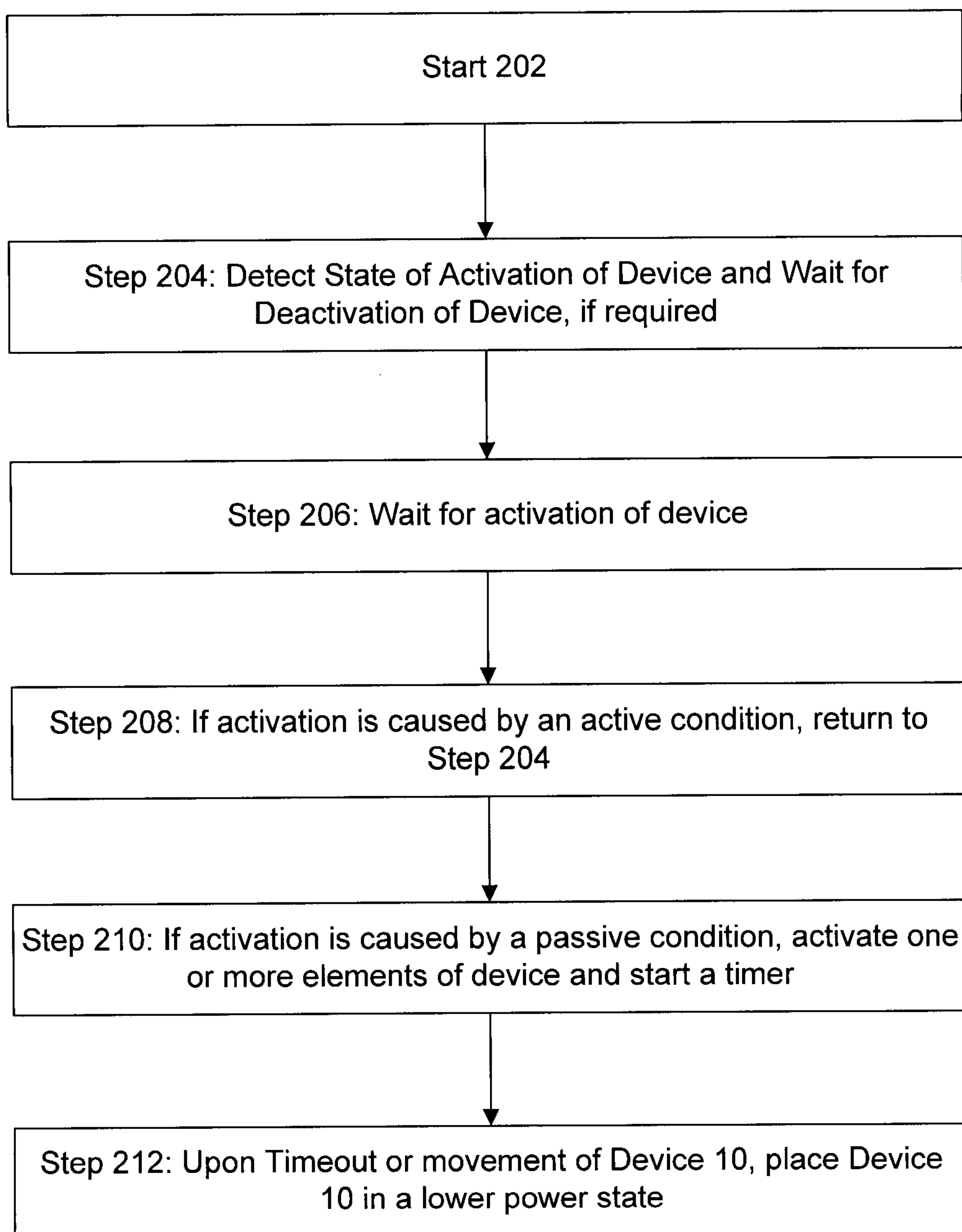
Algorithm 200
