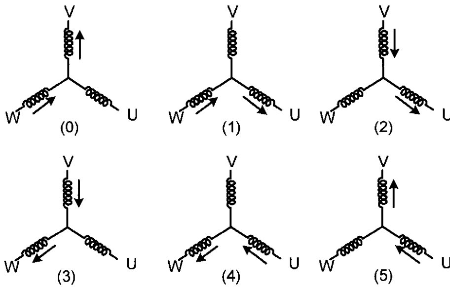
FIG. 3 PRIOR ART
