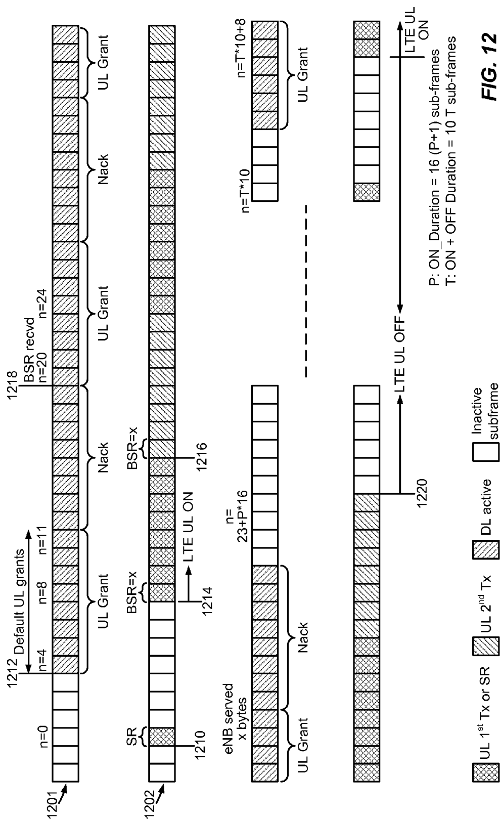
BSR Timeline example: FDD, one re-transmission
