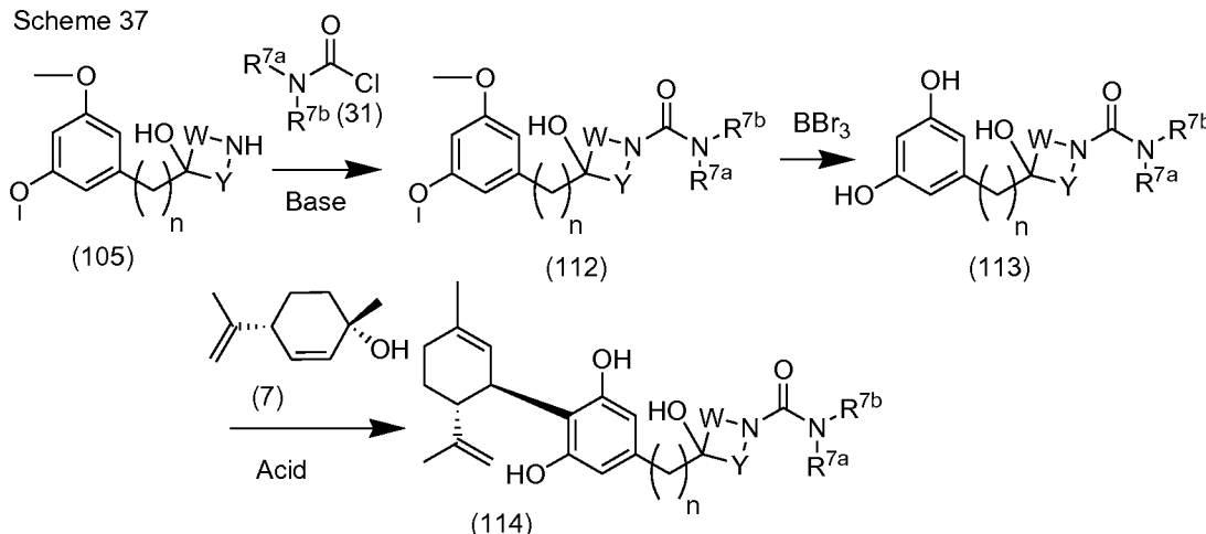
Scheme 37
