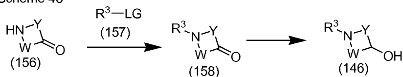
Scheme 48
