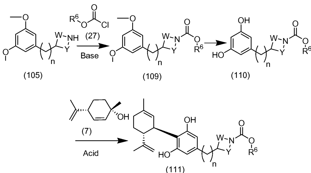
Scheme 36
