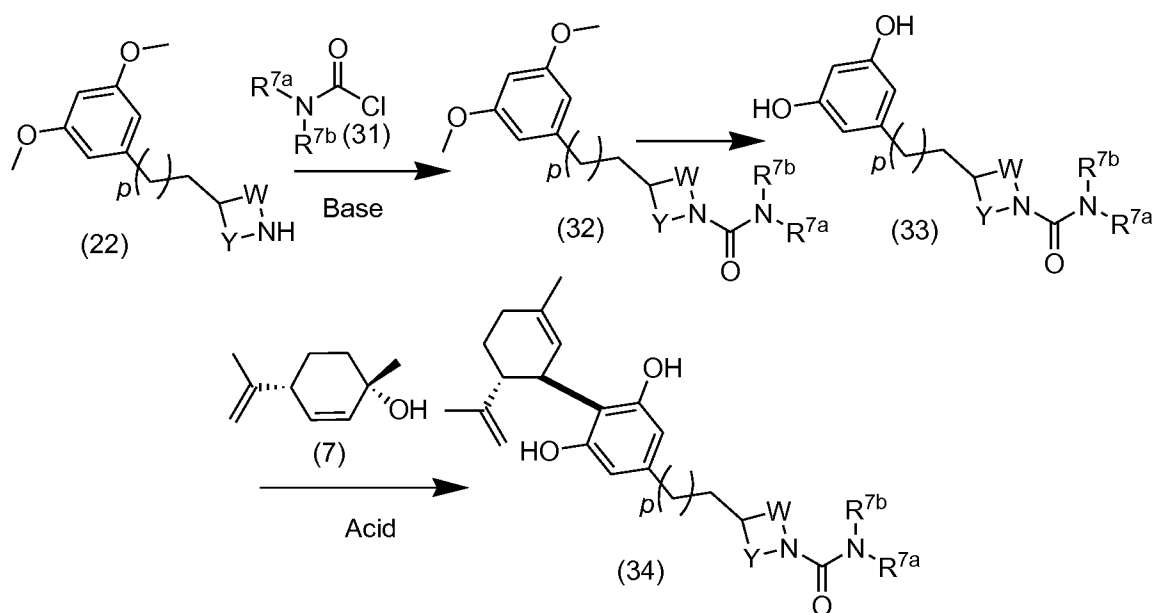
Scheme 12
