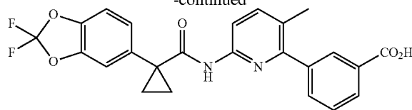
Compound 1
