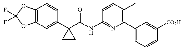
Compound 1
