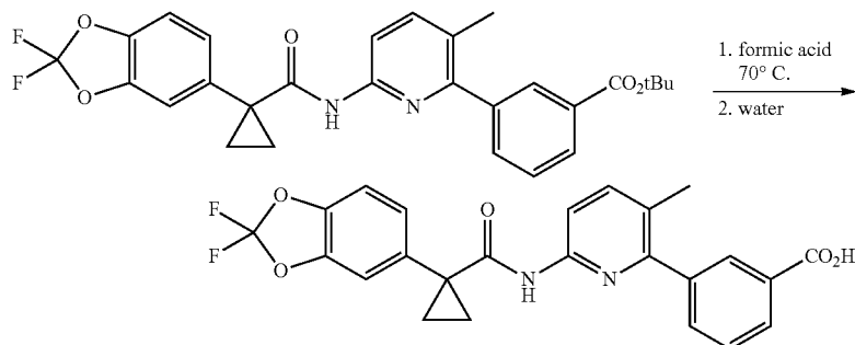
Compound 1
