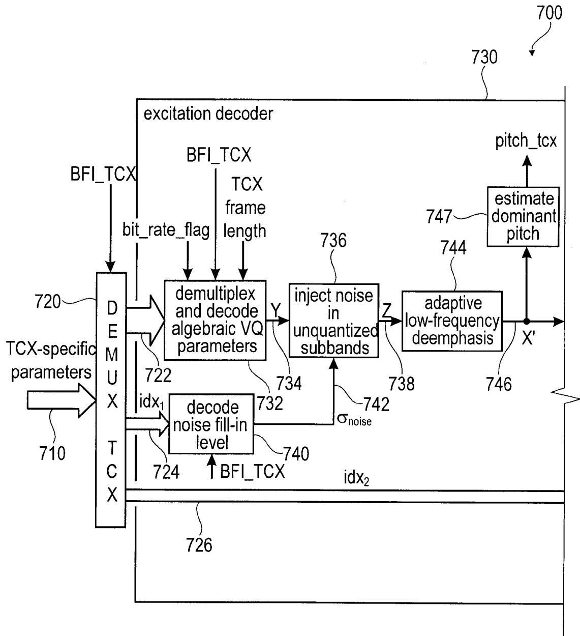
Block diagram of the TCX decoder
