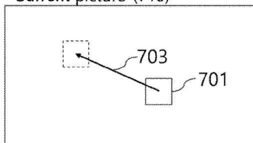
Current picture (710)
