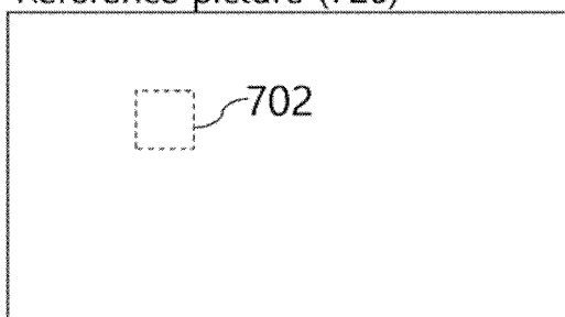
Reference picture (720)
