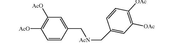
N-acetyl-bis-(3,4-diacetoxybenzyl)-amine
