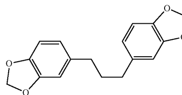
1,3-bis(3,4-methylenedioxyphenyl)propane
