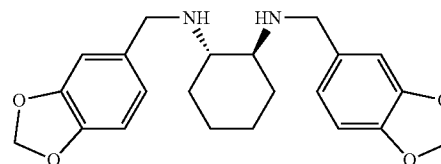
N,N'-bis(3,4-methylenedioxybenzyl)-trans-1,2-diaminocyclohexane
