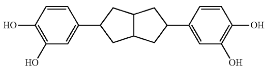
2,5-bis(3,4-dihydroxybenzoyl)bicyclo[3.3.0]octane
