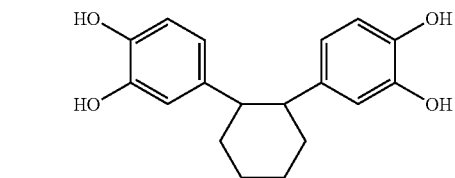
1,2-bis(3,4-dihydroxyphenyl)cyclohexane
