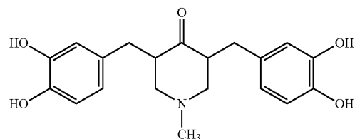
3,5-bis(3,4-dihydroxybenzyl)-1-methyl-4-piperidinone
