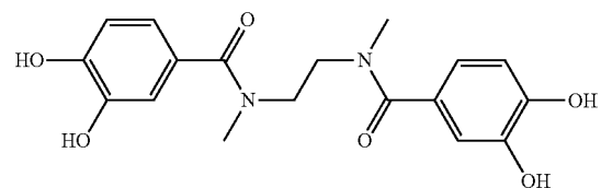
N,N'-bis(3,4-dihydroxybenzoyl)-N,N'-dimethyl (-)ethylenediamine
