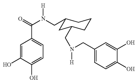
N,N'-bis(3,4-dihydroxybenzoyl)-cis-1,3-bis-aminomethylcyclohexane
