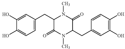
3,6-bis(3,4-dihydroxybenzylidene)-1,4-dimethyl-2,5-diketopiperazine
