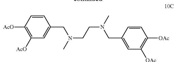
N,N'-bis(3,4-diacetoxybenzyl)-N,N'-dimethylethylenediamine
