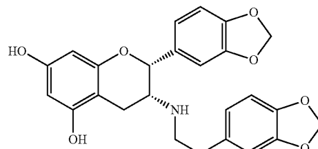
3-deoxy-3-(3,4-methylenedioxyphenethyl)-aminoepicatechin
