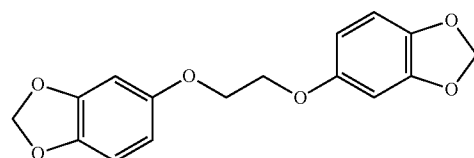
1,2-bis(3,4-methylenedioxyphenoxy) ethane
