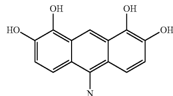
10-Amino-anthracene-1,2,7,8-tetraol
