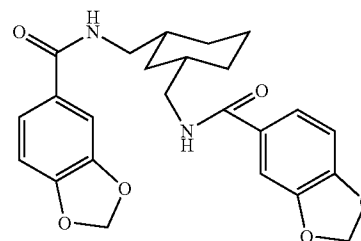
N,N'-bis(3,4-methylenedioxybenzoyl)-cis-1,3-bis-aminomethylcyclohexane
