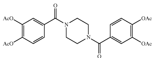
1,4-bis(3,4-diacetoxybenzoyl) piperazine
