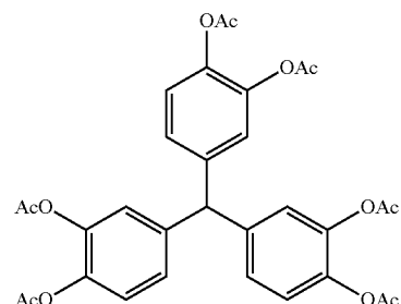
Tris-(3,4-diacetoxyphenyl)methane
