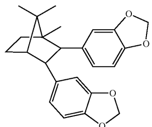
2,3-bis(3,4-methylenedioxyphenyl)-1,7,7- trimethyl-bicyclo[2,2,1]heptane
