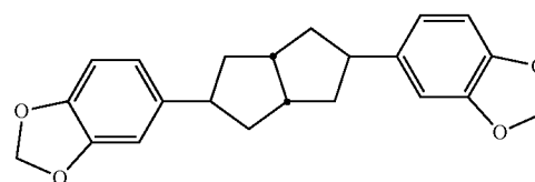
3,7-bis(3,4-methylenedioxyphenyl) bicyclo[3,3,0]octane
