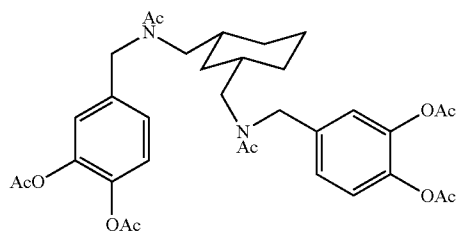
N,N'-bis(acetyl)-bis(3,4-diacetoxybenzyl)-cis-1,3-bis-aminomethylcyclohexane
