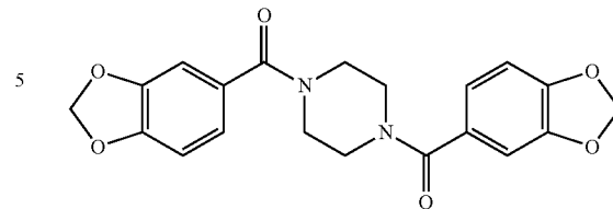
1,4-bis(3,4-methylenedioxybenzoyl) piperazine
