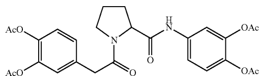
N-(3,4-diacetoxyphenylacetyl)-proline-3,4- diacetoxyanilide
