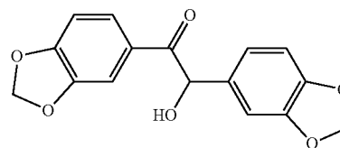
bis(3,4-methylenedioxy)benzoin
