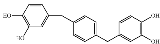
1,4-bis(3,4-dihydroxybenzyl)-benzene
