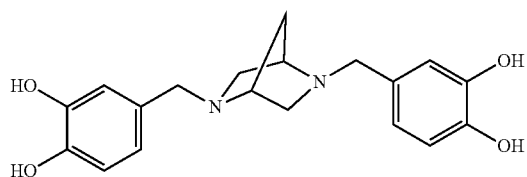
2,5-bis(3,4-dihydroxybenzyl)-2,5-diaza-[2.2.1]- bicycloheptane
