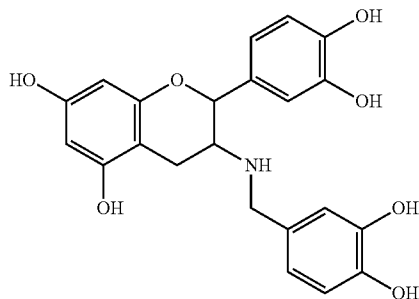
3-deoxy-3-(3,4-dihydroxybenzyl)(-)-amino- epicatechin
