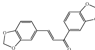
bis(3,4-methylenedioxy)chalcone
