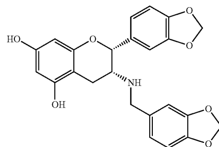
3-deoxy-3-(3,4-methylenedioxybenzyl)-aminoepicatechin
