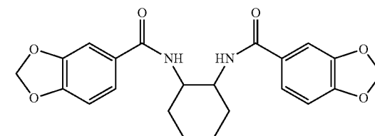
N,N'-bis(3,4-methylenedioxybenzoyl)-trans-diaminocyclohexane
