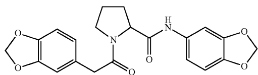
N-(3,4-methylenedioxyphenylacetyl)-proline-3,4- methylenedioxyanilide
