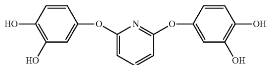
2,6-bis(3,4-dihydroxyphenoxy)pyridine
