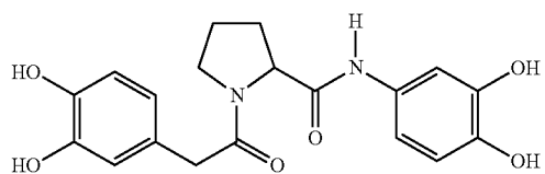
N-(3,4-hydroxyphenylacetyl)proline-3,4-dihydroxyanilide
