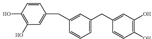
1,3-bis(3,4-dihydroxybenzyl)-benzene
