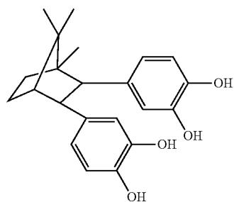
2,3-bis(3,4-dihydroxyphenyl)-1,7,7-trimethylbicyclo[2.2.1]heptane
