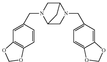
2,5-bis(3,4-methylenedioxybenzyl)-2,5-diaza[2,2,1]-bicycloheptane
