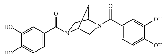
2,5-bis(3,4-dihydroxybenzoyl)-2,5-diaza- [2.2.1]-bicycloheptane
