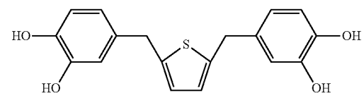
2,5-bis(3,4-dihydroxybenzyl)thiophene
