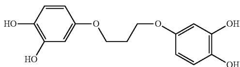
1,3-bis(3,4-dihydroxyphenoxy)propane
