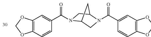
2,5-bis(3,4-methylenedioxybenzoyl)-2,5-diaza[2,2,1]-bicycloheptane
