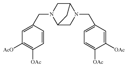
2,5-bis(3,4-diacetoxybenzyl)-2,5-diaza[2,2,1]-bicycloheptane
