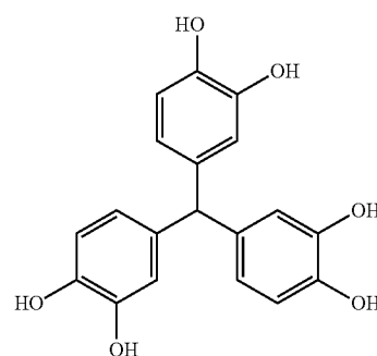
Tris-(3,4-dihydroxybenzyl)methane
