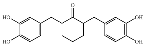
2,6-bis(3,4-dihydroxybenzyl)cyclohexanone
