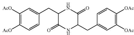
3,6-bis(3,4-diacetoxybenzyl)-2,5- diketopiperazine
