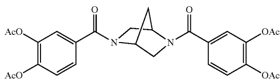
2,5-bis(3,4-diacetoxybenzoyl)-2,5- diaza[2,2,1]-bicycloheptane
