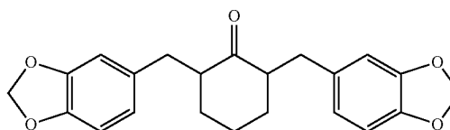
2,6-bis(3,4-methylenedioxybenzyl) cyclohexanone
