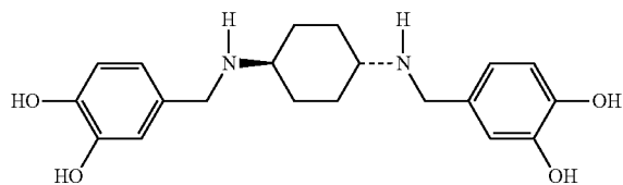
N,N'-bis(3,4-dihydroxybenzyl)-trans-1,4-diaminocyclohexane
