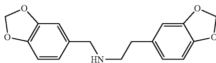
N-(3,4-methylenedioxybenzyl)-3,4-methylenedioxyphenethylamine
