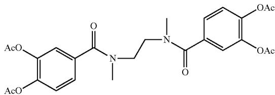
N,N'-bis(3,4-diacetoxybenzoyl)-N,N'- dimethyl(-)ethylenediamine
