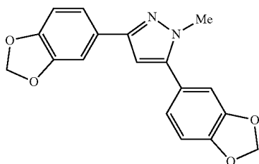
3,5-bis(3,4-methylenedioxyphenyl)-1-methyl-1H-pyrazoline
