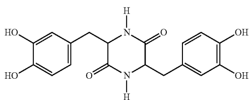
3,6-bis(3,4-dihydroxybenzyl)-1-methyl-2,5-diketopiperazine
