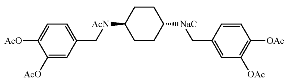
N,N'-bis(acetyl)-bis(3,4-diacetoxybenzyl)-trans-1,4-diaminocyclohexane
