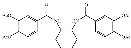
N,N'-bis(3,4-diacetoxybenzoyl)-trans- diaminocyclohexane
