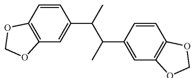
2,3-bis(3,4-methylenedioxyphenyl) butane
