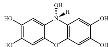
Phenoxazine-2,3,7,8,10-pentaol
