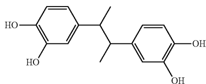
2,3-bis(3,4-dihydroxyphenyl)butane
