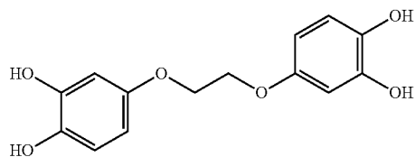
1,2-bis(3,4-dihydroxyphenoxy)ethane
