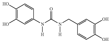
1-(3,4-dihydroxyphenyl)-3-(3,4-dihydroxybenzyl) urea
