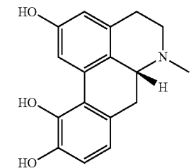
6-Methyl-5,6,6a,7-tetrahydro-4H-dibenzo[de,g]quinoline-2,10,11-triol
