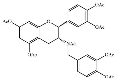
N-acetyl-3-deoxy-3-(3,4-diacetoxybenzyl)-amino-5,7,3',4'-tetraacetyl-epicatechin
