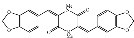
3,6-bis(3,4-methylenedioxybenzylidene)- 1,4-dimethyl-2,5-diketopiperazine
