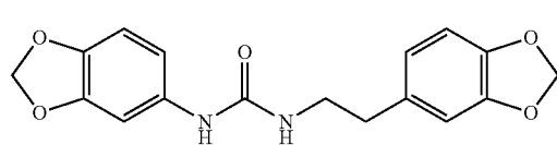
1-(3,4-methylenedioxyphenyl)-3-(3,4-methylenedioxyphenethyl) urea
