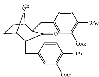
2,4-bis(3,4-diacetoxybenzyl)-3-tropinone
