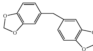
1,1-bis(3,4-methylenedioxyphenyl)methane
