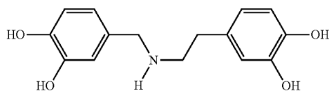
N-(3,4-dihydroxybenzyl)-3,4-dihydroxy(-) phenethylamine
