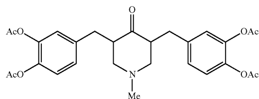
3,5-bis(3,4-diacetoxybenzyl)-1-methyl-4-piperidinone
