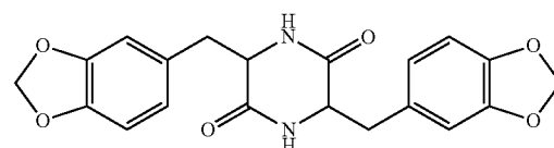
3,6-bis(3,4-methylenedioxybenzyl)-2,5-diketopiperazine
