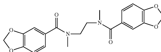
N,N'-bis(3,4-methylenedioxybenzoyl)-N,N'-dimethyl(-)ethylenediamine
