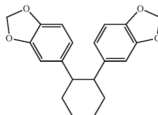
1,2-bis(3,4-methylenedioxyphenyl) cyclohexane
