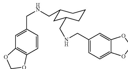
N,N'-bis(3,4-methylenedioxybenzyl)-cis-1,3-bis-aminomethylcyclohexane
