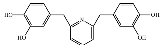
2,6-bis(3,4-dihydroxybenzyl)pyridine
