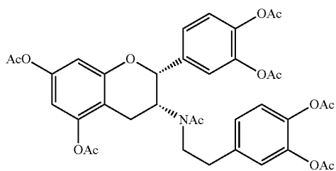
N-acetyl-3-deoxy-3-(3,4-diacetoxyphenethyl)-amino-5,7,3',4'-tetraacetyl-epicatechin
