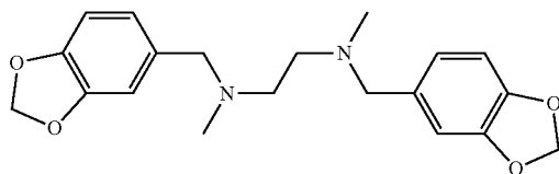
N,N'-bis(3,4-methylenedioxybenzyl)-N,N'-dimethyl-ethylenediamine
