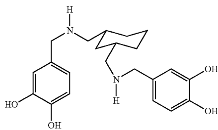
N,N'-bis(3,4-dihydroxybenzyl)-cis-1,3-bis- aminomethylcyclohexane
