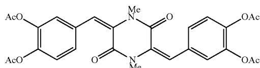
3,6-bis(3,4-diacetoxybenzylidene)- 1,4-dimethyl-2,5-diketopiperazine
