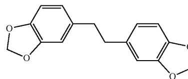
1,2-bis(3,4-methylenedioxyphenyl)ethane
