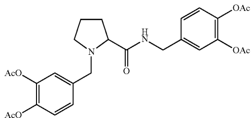
N-(3,4-diacetoxybenzyl)proline 3,4-diacetoxybenzylamide
