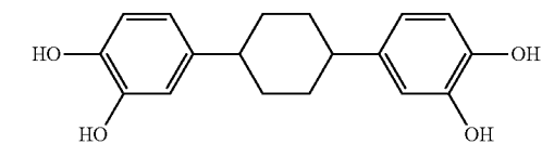
3,7-bis(3,4-dihydroxyphenyl)cyclohexane
