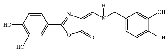
4-(3,4-dihydroxybenzylaminomethylene)-2- (3,4-dihydroxyphenyl)oxazolin-5-one
