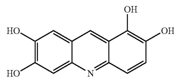
Acridine-1,2,6,7-tetraol
