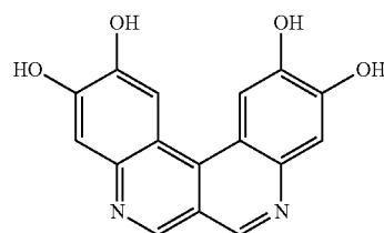
Dibenzo[c,f][2,7]naphthyridine-2,3,10,11-tetraol
