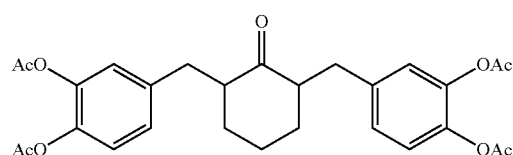
2,6-bis(3,4-diacetoxybenzyl) cyclohexanone
