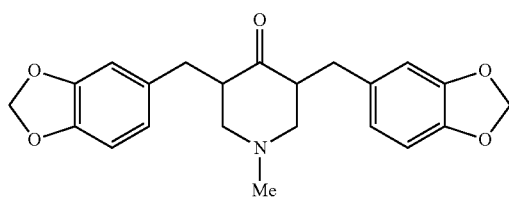
3,5-bis(3,4-methylenedioxybenzyl)-1-methyl-4-piperidinone
