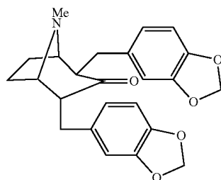
2,4-bis(3,4-methylenedioxybenzyl)-3-tropinone
