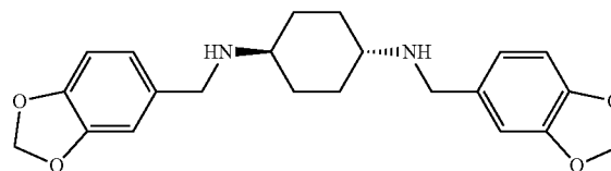
N,N'-bis(3,4-methylenedioxybenzyl)-trans-1,4-diaminocyclohexane
