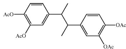
2,3-bis(3,4-diacetoxyphenyl) butane
