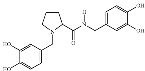
N-(3,4-dihydroxybenzyl)proline 3,4-dihydroxy-benzylamide
