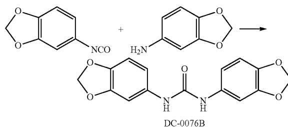
DC-0076B
