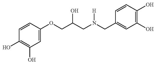
N-(3,4-dihydroxybenzyl)-3-(3,4-dihydroxypropyl)amine
