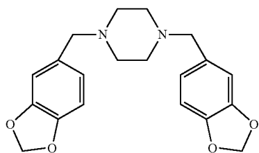
1,4-bis(3,4-methylenedioxybenzyl)piperazine
