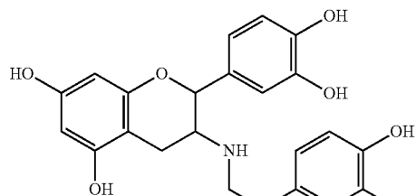
3-deoxy-3-(3,4-dihydroxyphenethyl)(-)-amino- epicatechin
