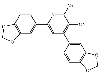
4,6-bis(3,4-methylenedioxyphenyl)-3-cyano-2-methylpyridine
