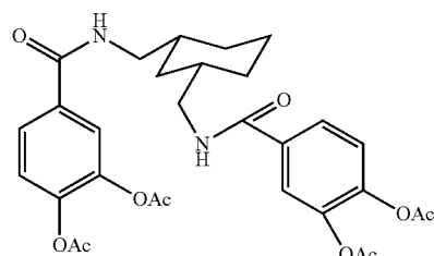
N,N'-bis(3,4-diacetoxybenzoyl)-cis-1,3- bis-aminomethylcyclohexane
