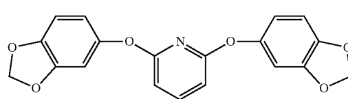
2,6-bis(3,4-methylenedioxyphenoxy) pyridine
