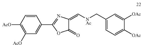
N-acetyl-4-(3,4-diacetoxybenzylamino-methylene)-2- (3,4-diacetoxyphenyl)-oxazolin-5-one
