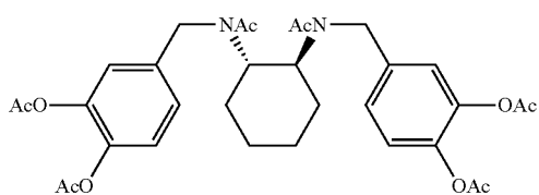
N,N'-bis(acetyl)-bis(3,4-diacetoxybenzyl)-trans-1,2-diaminocyclohexane
