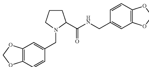
N-(3,4-methylenedioxybenzyl)proline 3,4-methylenedioxybenzylamide
