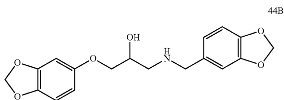
N-(3,4-methylenedioxybenzyl)-3-(3,4-methylenedioxyphenoxy)-2-hydroxypropylamine
