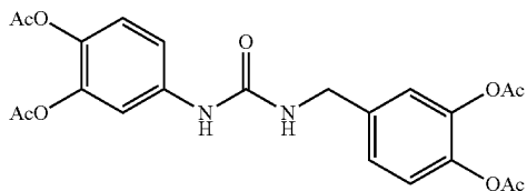
1-(3,4-diacetoxyphenyl)-3-(3,4-diacetoxybenzyl) urea
