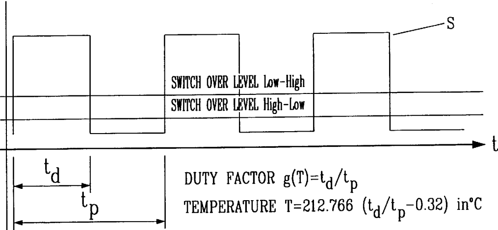
ORIGINAL SIGNAL AT SENSOR OUTPUT
