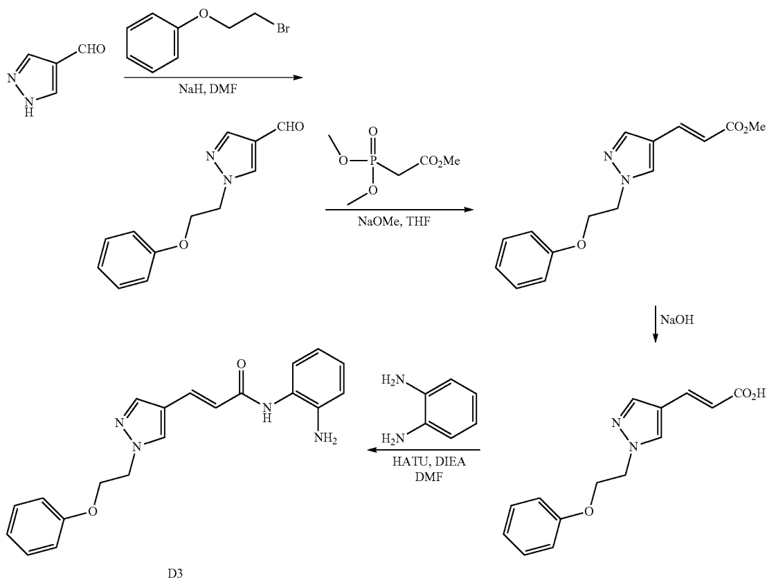
(E)-ethyl 3-(1-(2-phenoxyethyl)-1H-pyrazol-4-yl)acrylate
