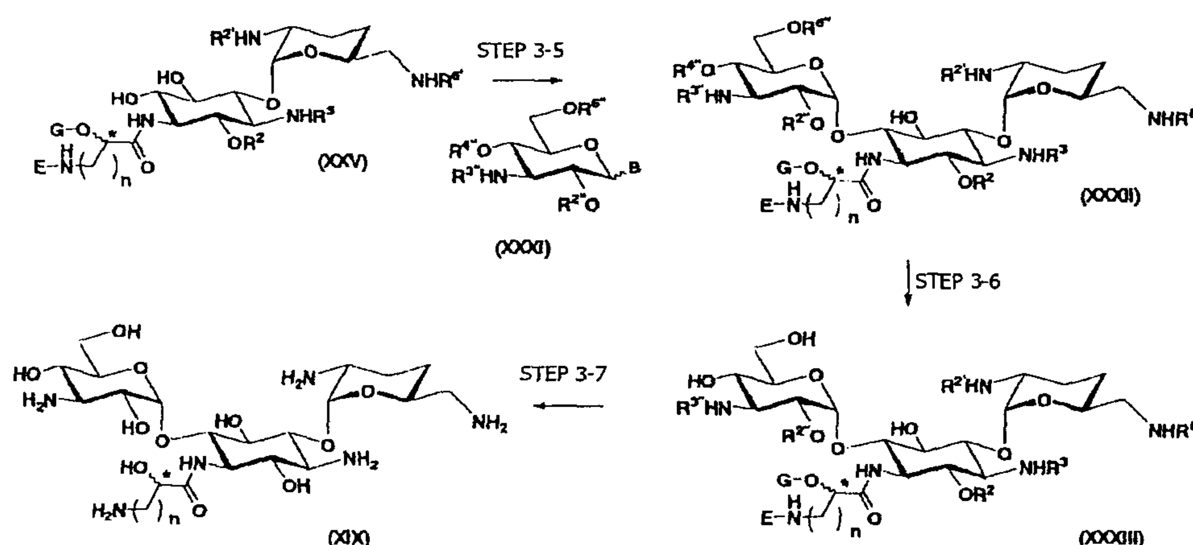
Scheme 7
