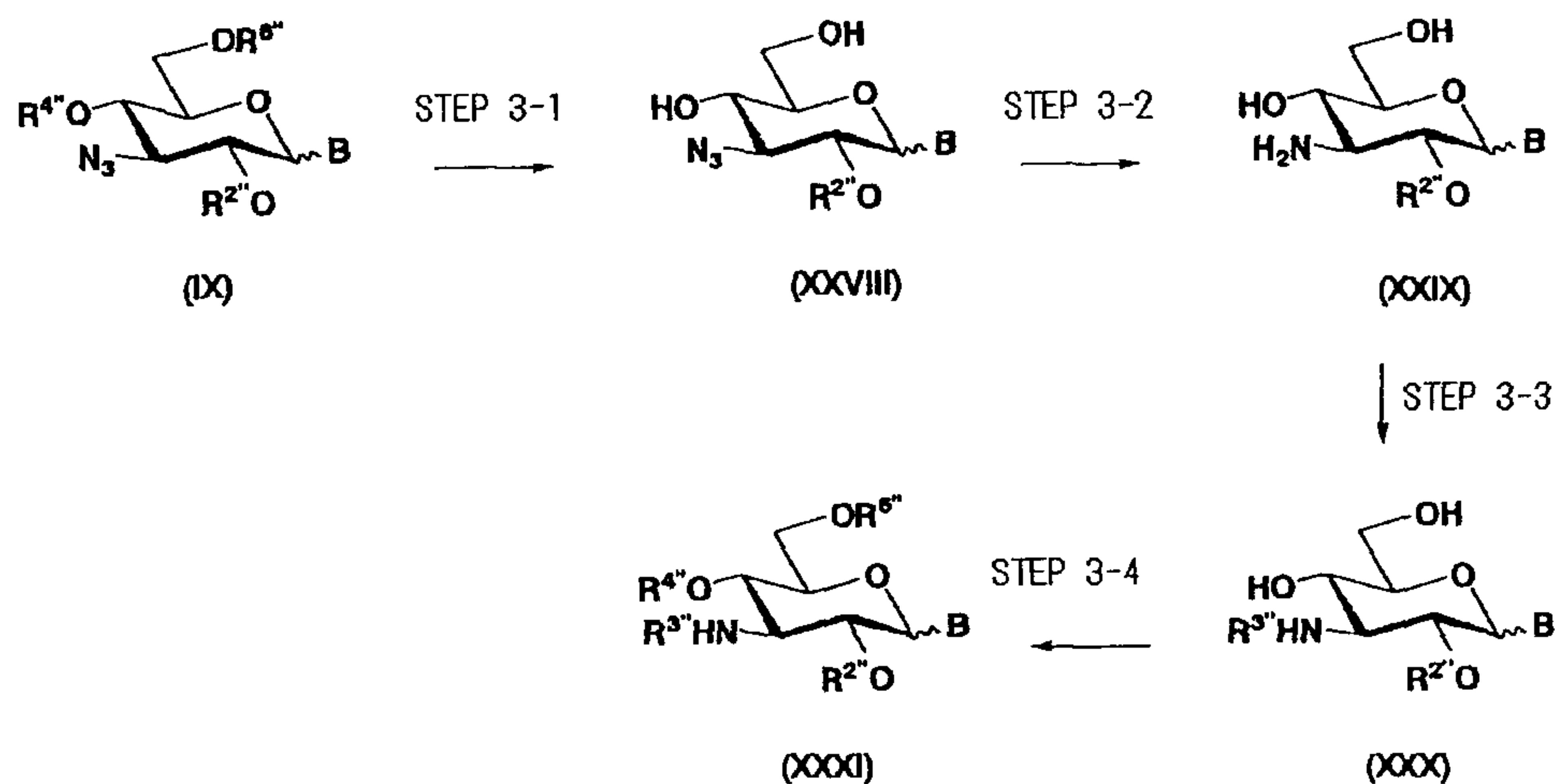
Scheme 6
