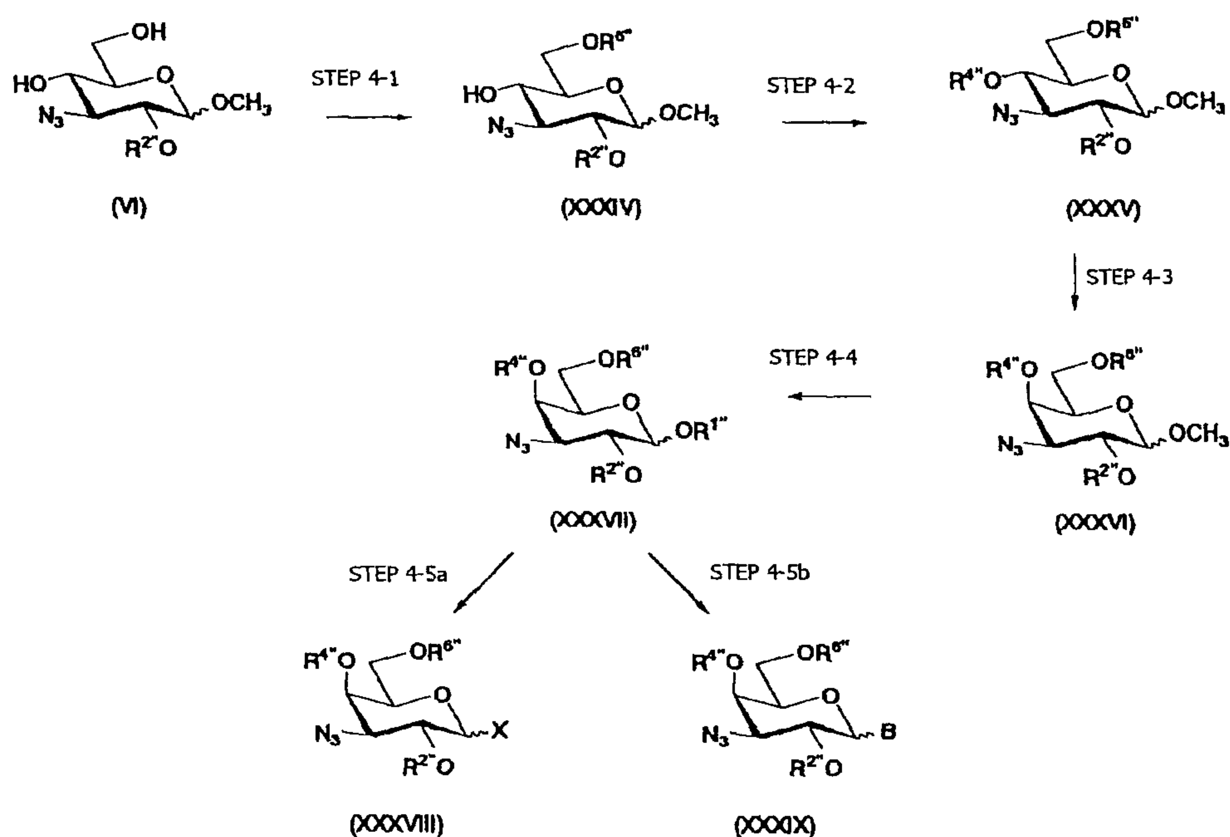
Scheme 8
