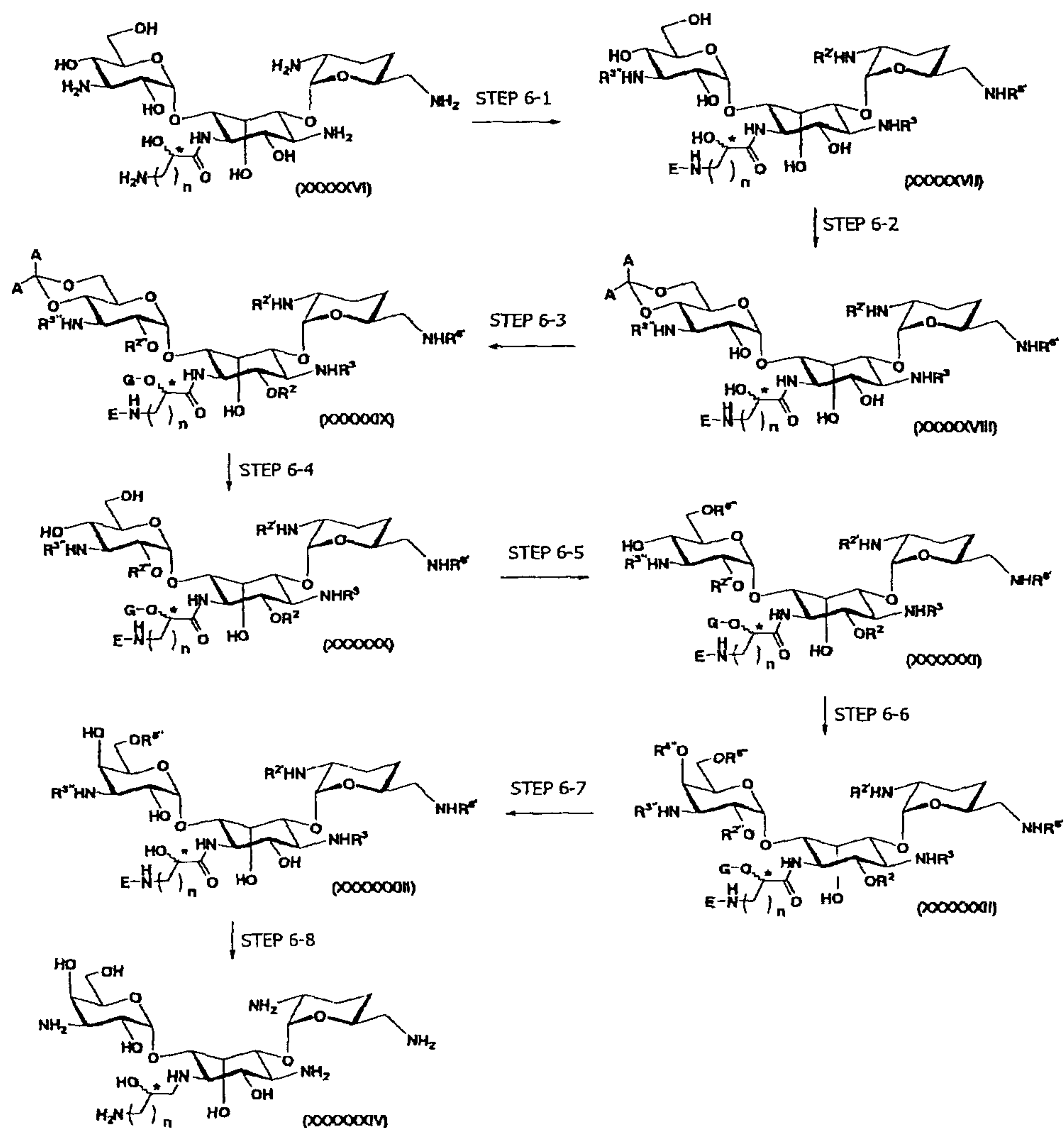
Scheme 12
