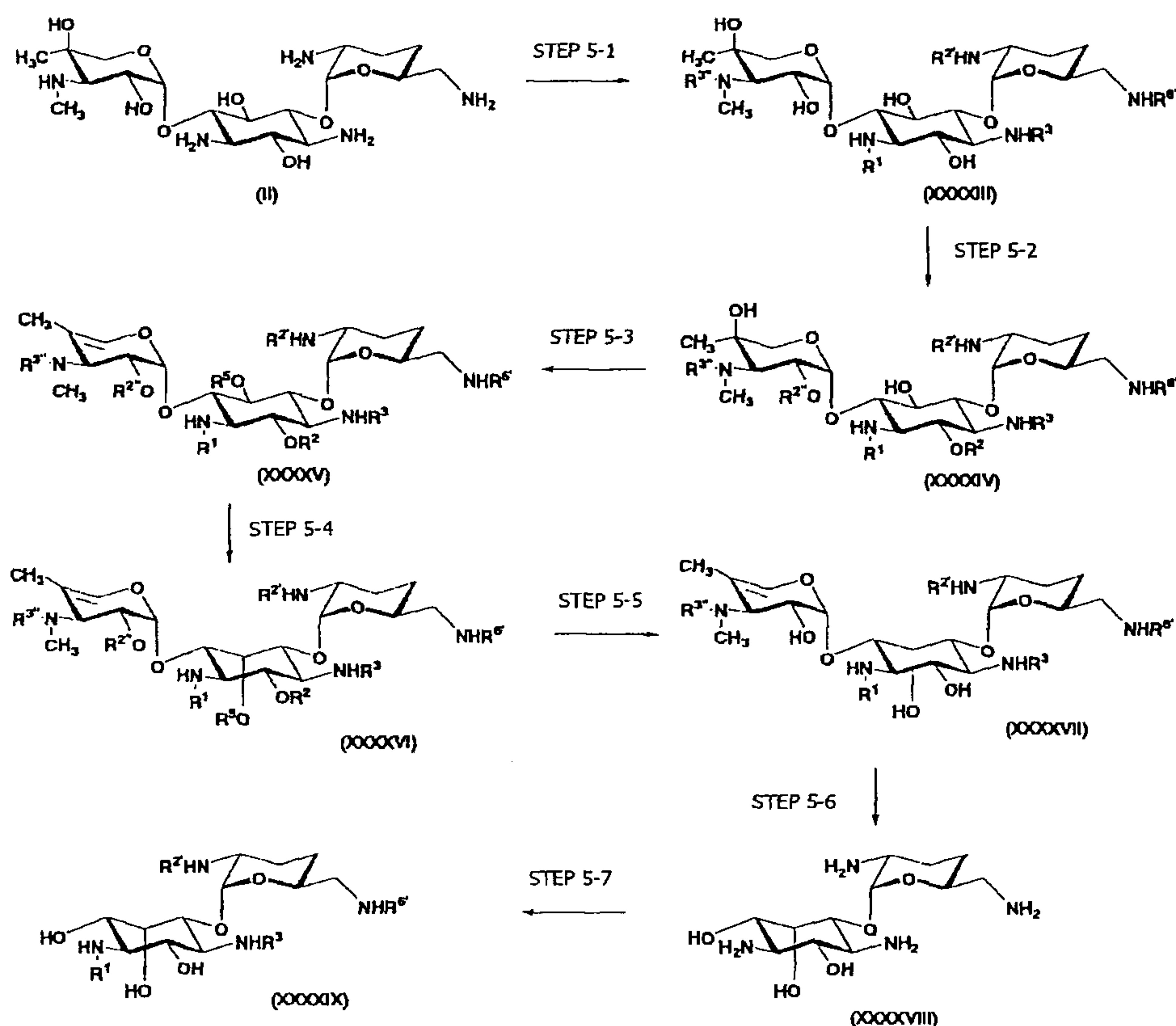
Scheme 10
