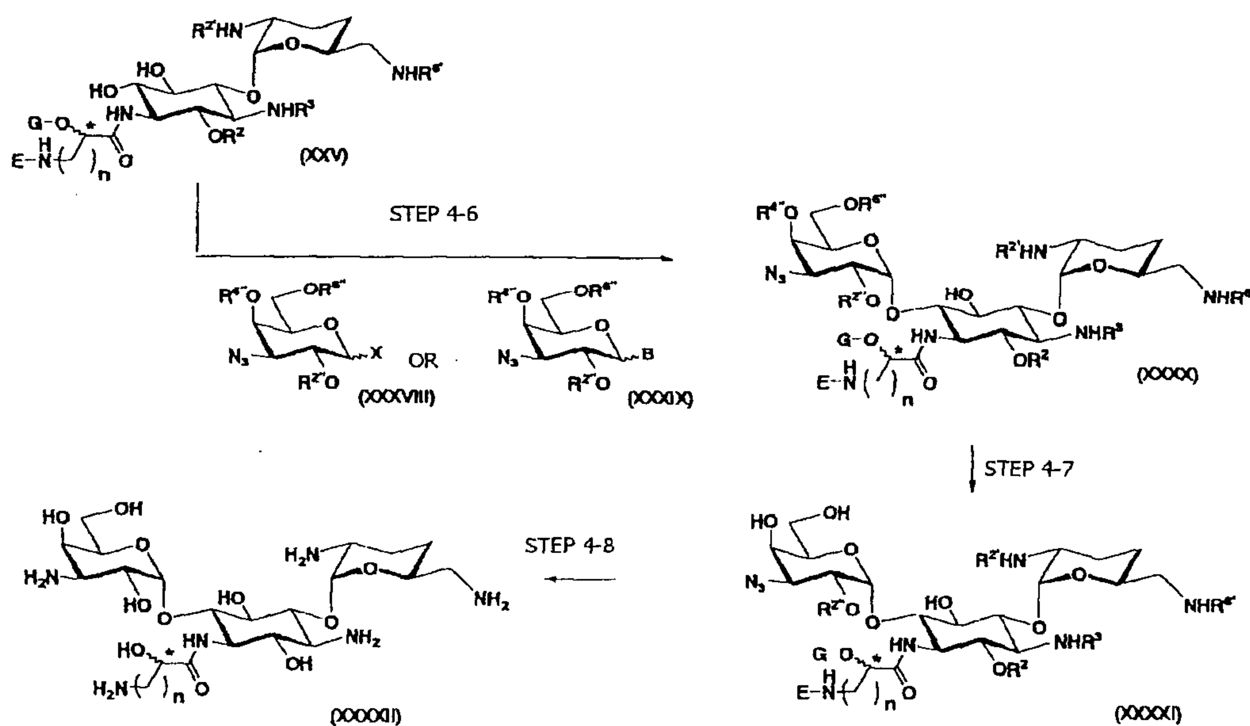
Scheme 9
