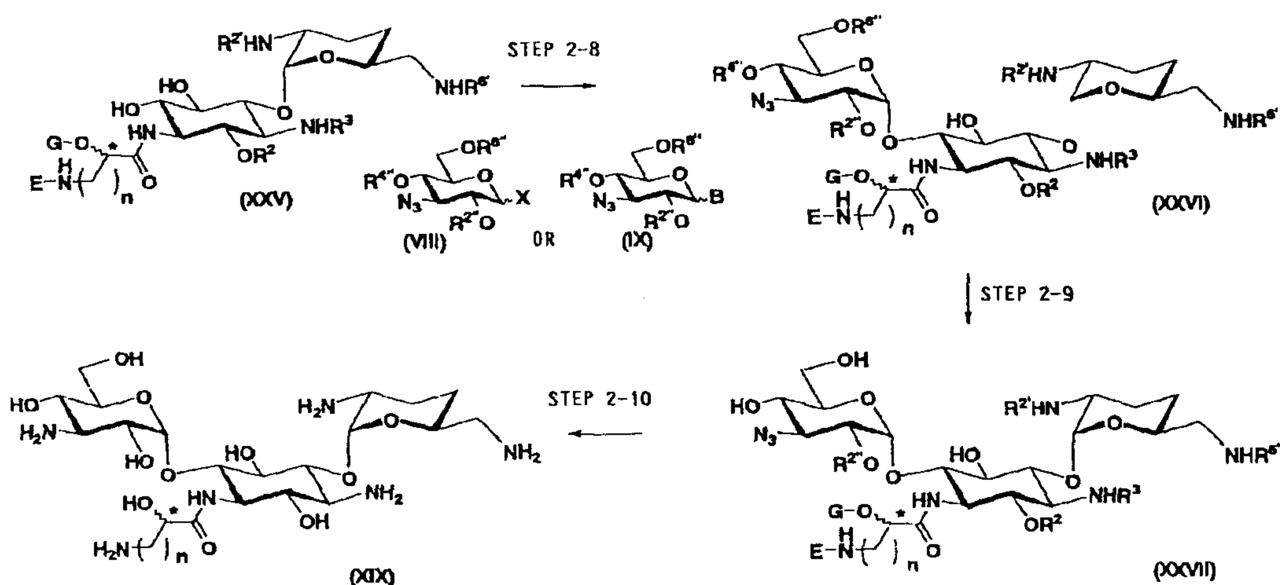
Scheme 5
