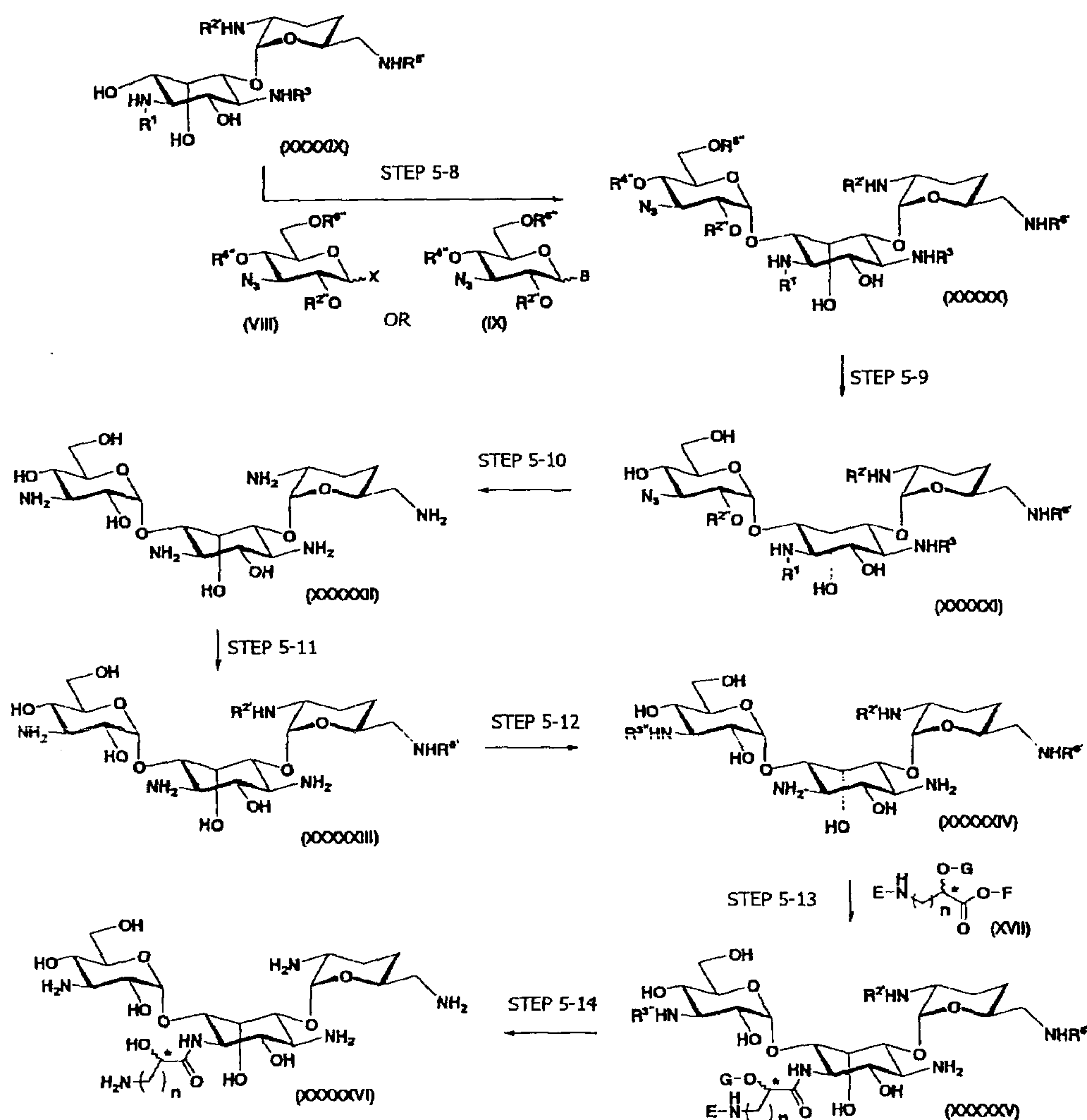
Scheme 11
