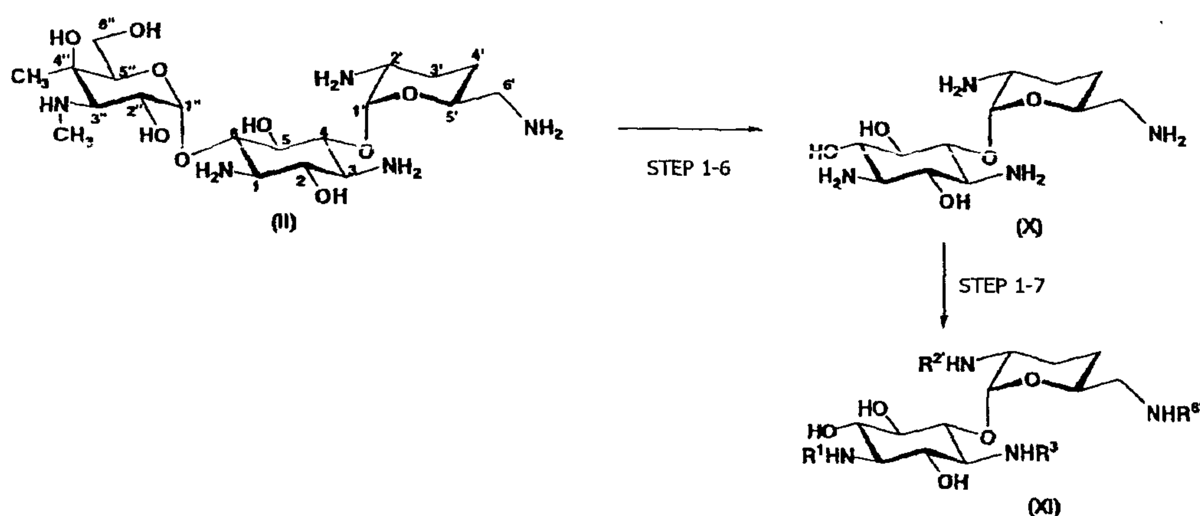
Scheme 2
