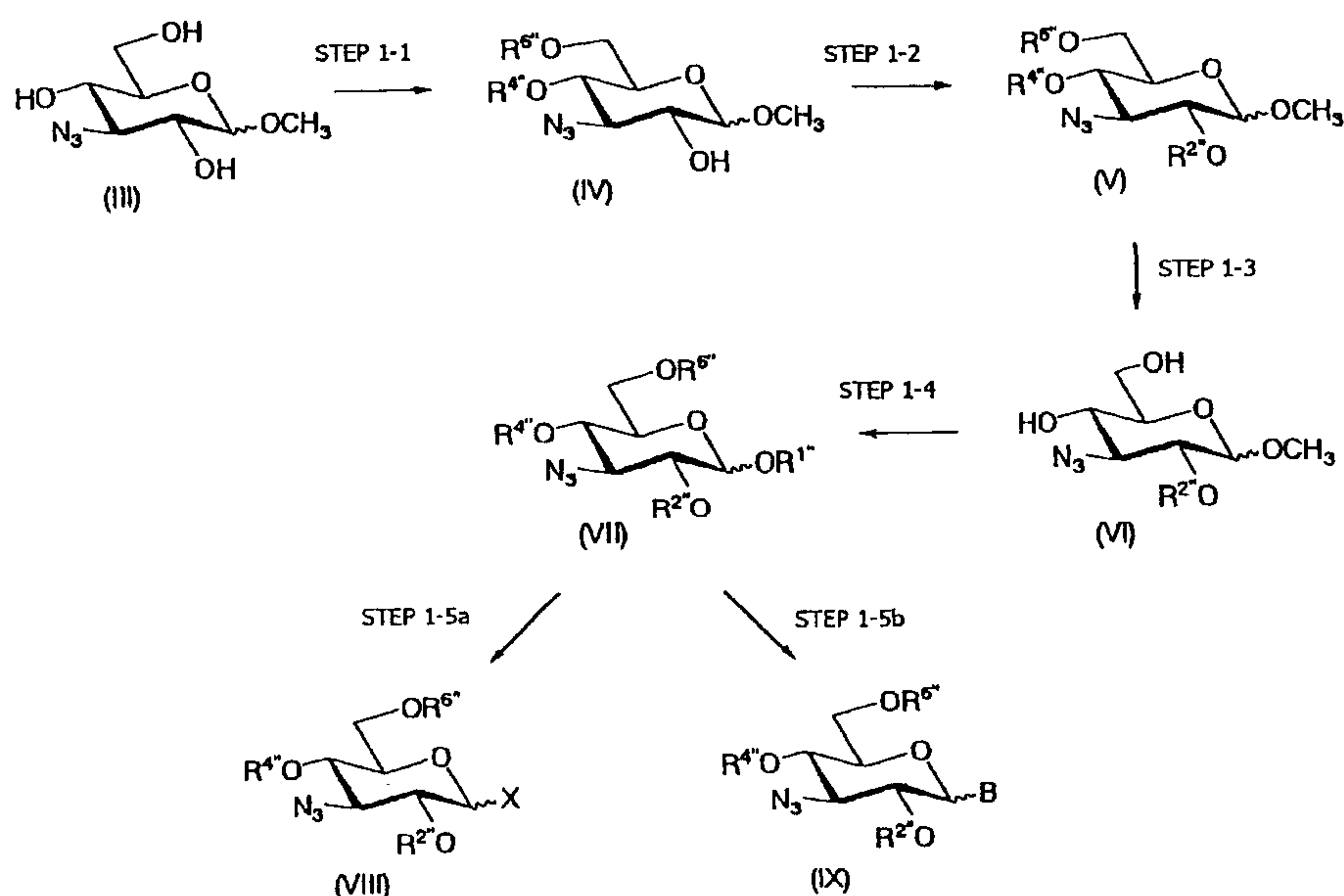
Scheme 1
