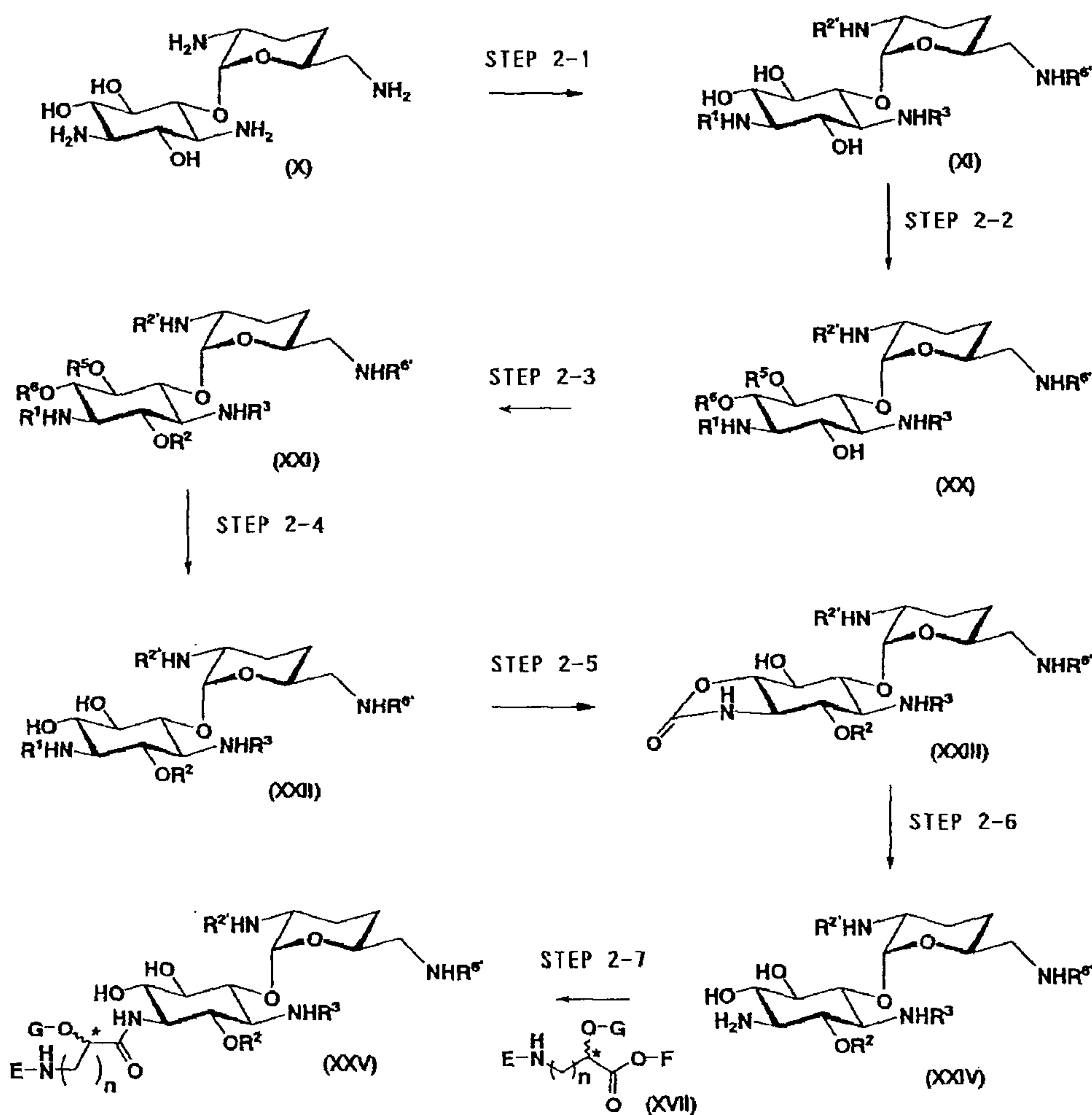
Scheme 4
