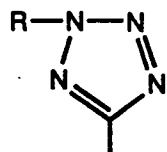
Tetrazole
