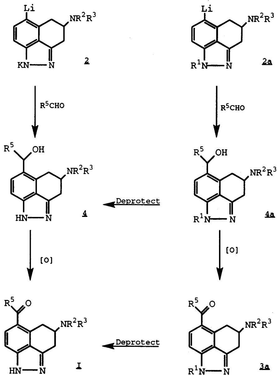
Scheme 3
