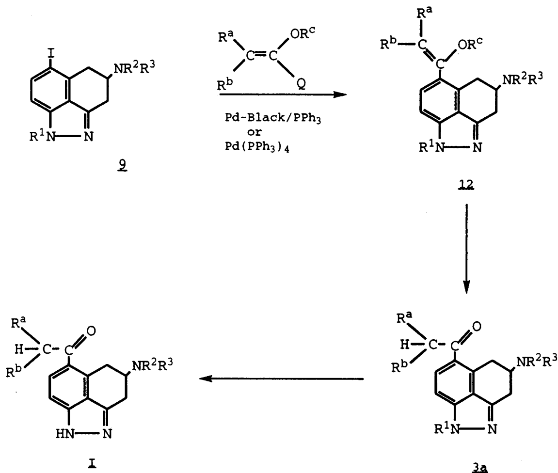
Scheme 9
