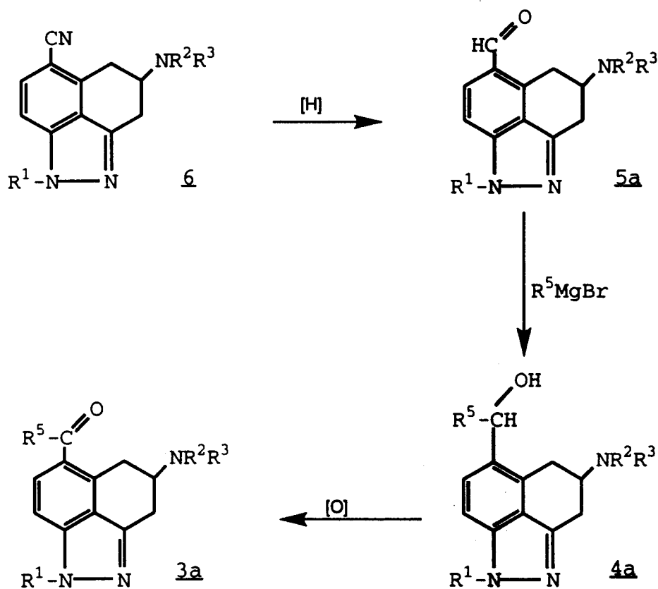
Scheme 6
