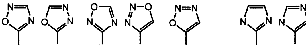
Oxadiazoles
