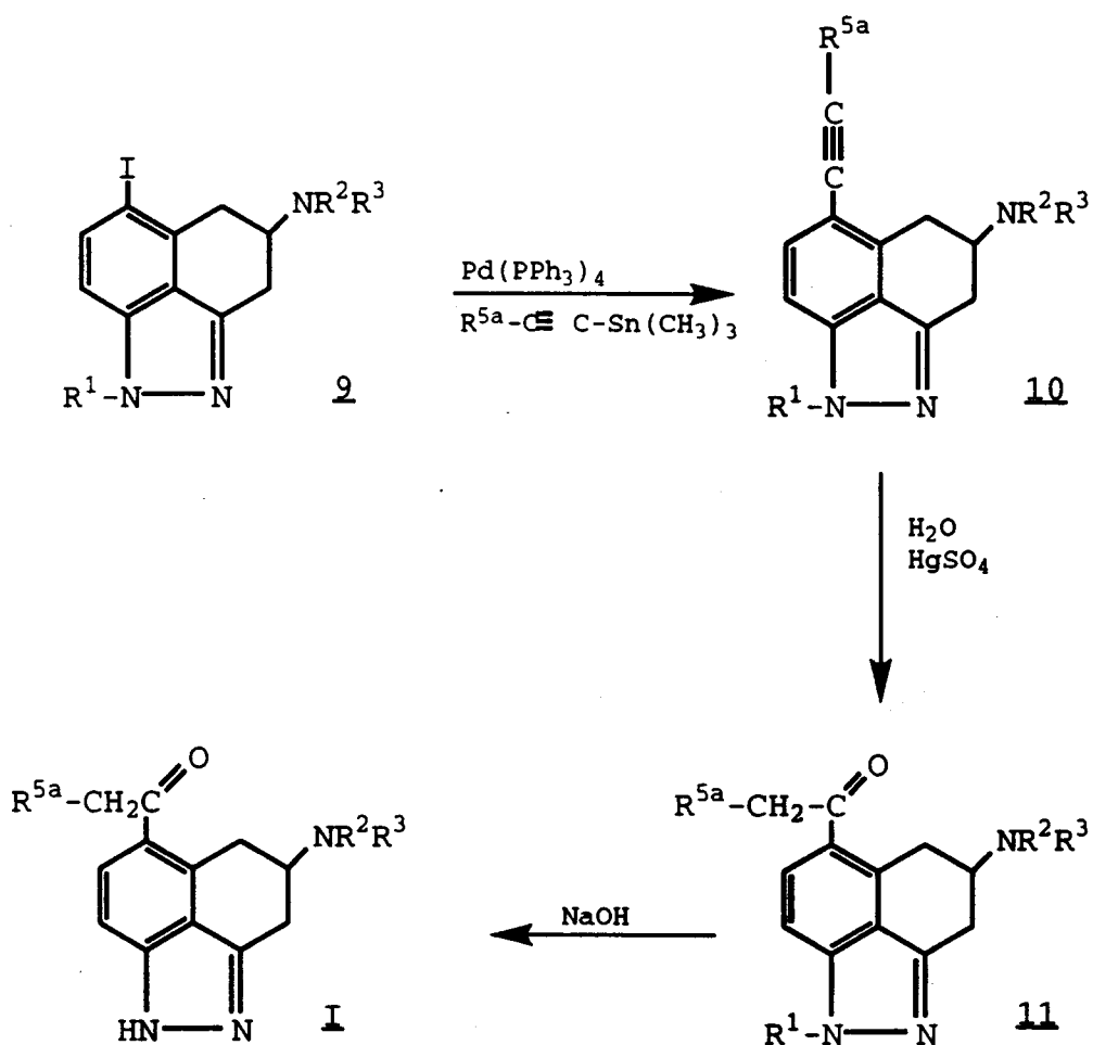
Scheme 7
