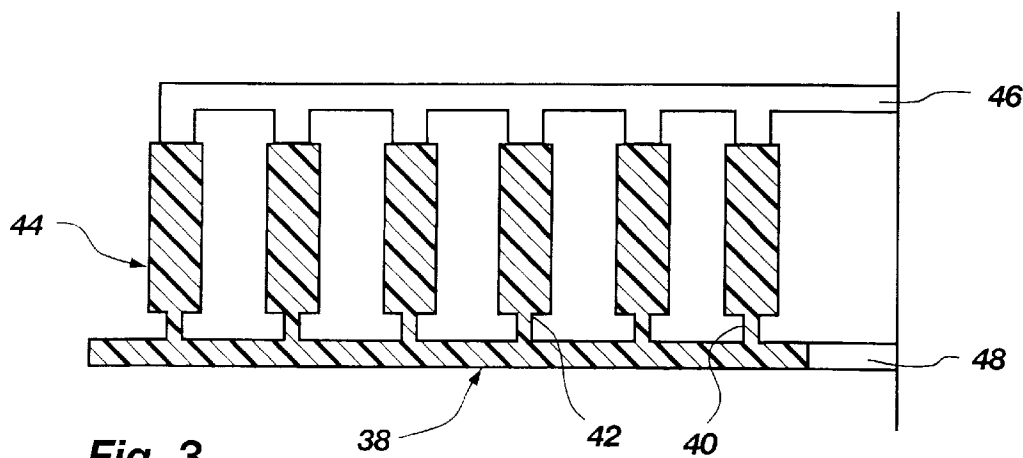
Fig. 3 (PRIOR ART)
