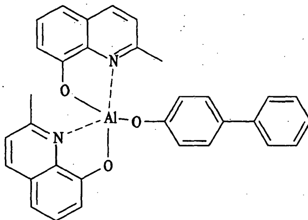
Balq [aluminum(III) bis(2-methyl-8-quinolinato) 4-phenylphenolate]
