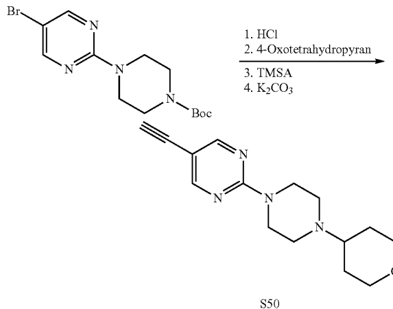
Synthesis of 5-ethynyl-2-(4-(tetrahydro-2H-pyran-4-yl)piperazin-1-yl)pyrimidine (S50)
