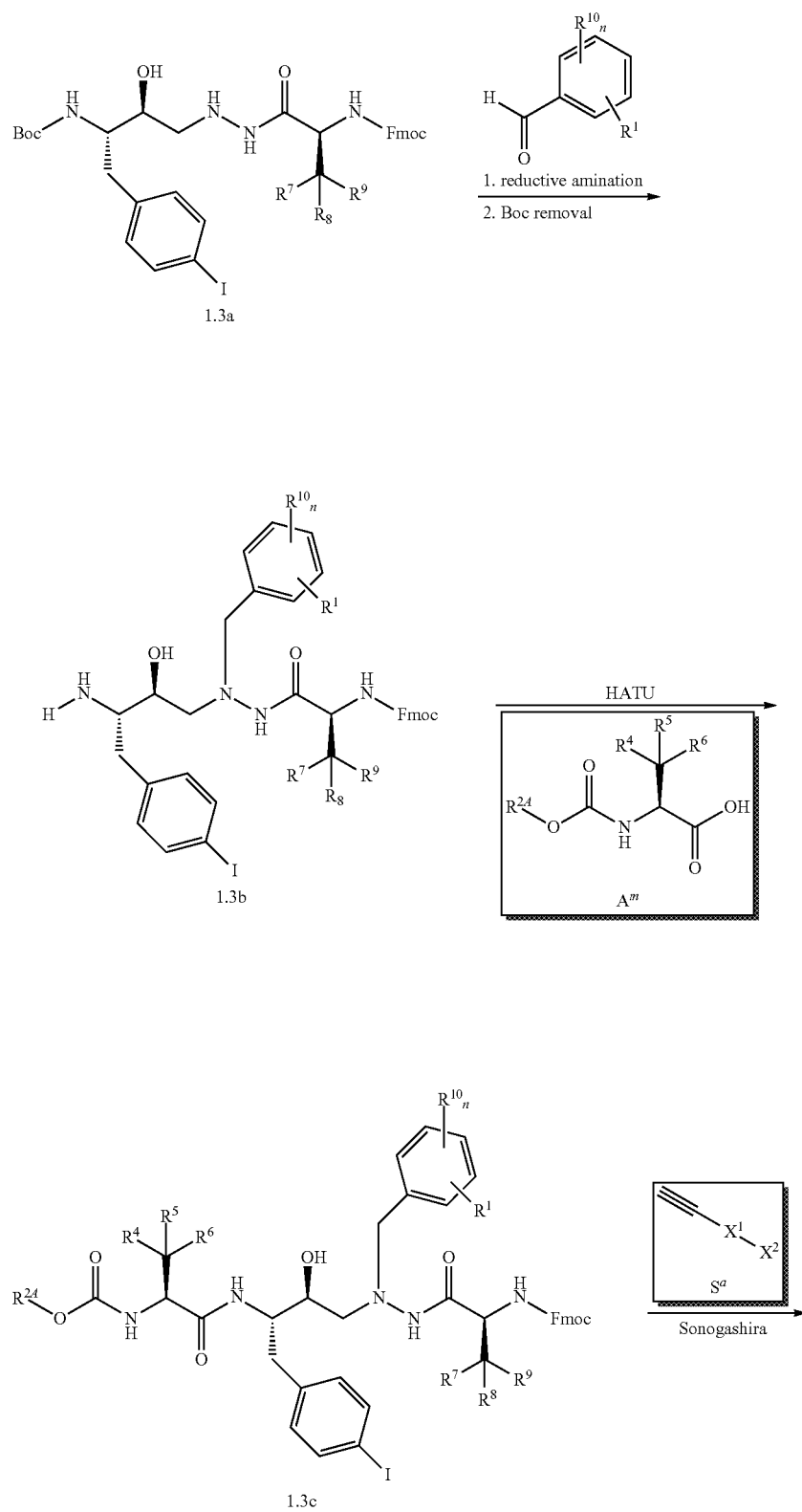
SCHEME 1.3
