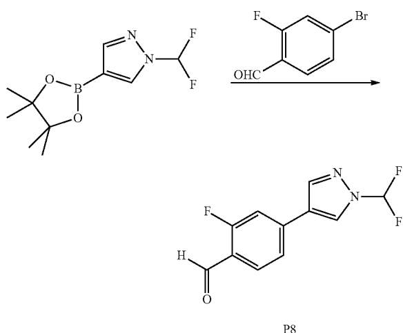
Synthesis of 4-(1-(difluoromethyl)-1H-pyrazol-4-yl)-2-fluorobenzaldehyde (P8)
