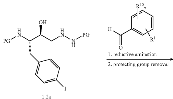
SCHEME 1.2
