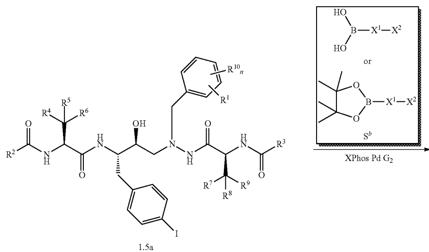
SCHEME 1.5
