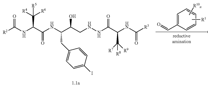
SCHEME 1.1
