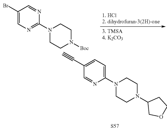
Synthesis of 1-(5-ethynylpyridin-2-yl)-4-(tetrahydrofuran-3-yl)piperazine (S57)
