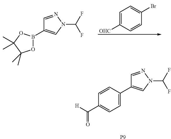
Synthesis of 4-(1-(difluoromethyl)-1H-pyrazol-4-yl)benzaldehyde (P9)
