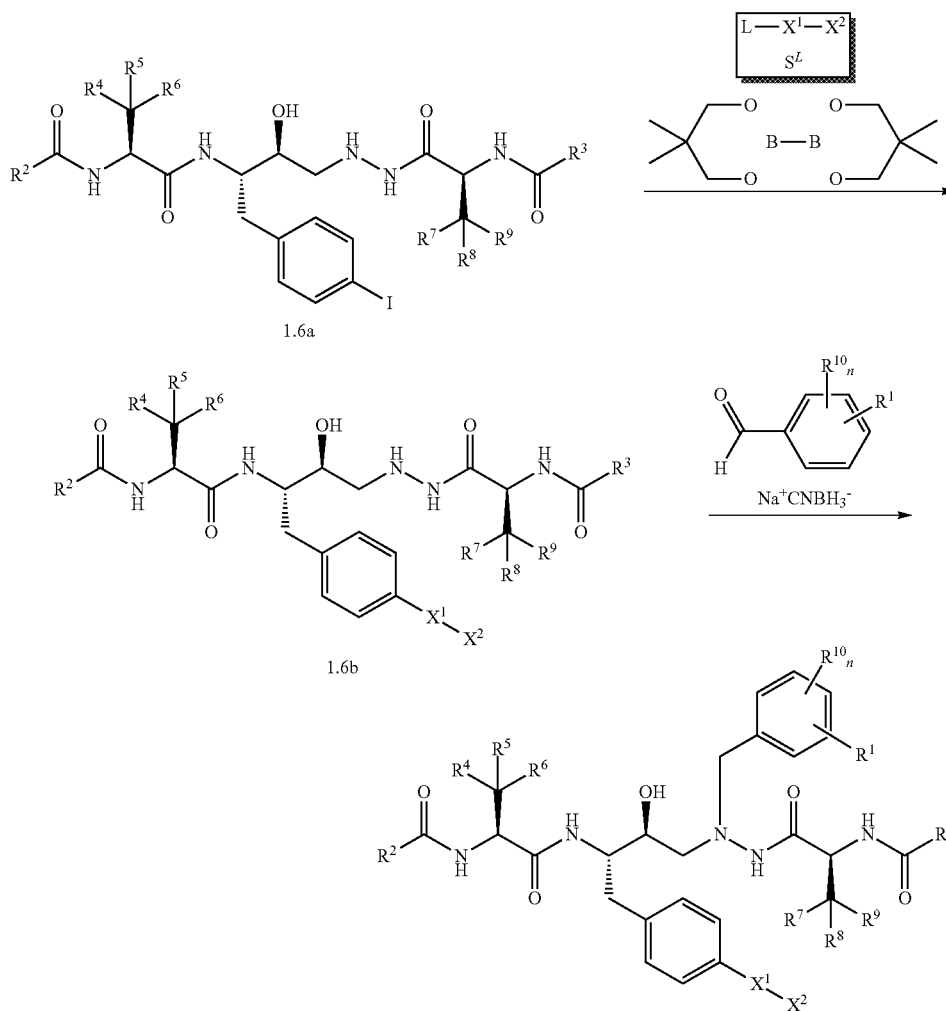
SCHEME 1.6
