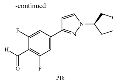
(R)-2,6-difluoro-4-(1-(tetrahydrofuran-3-yl)-1H-pyrazol-3-yl)benzaldehyde (P18)
