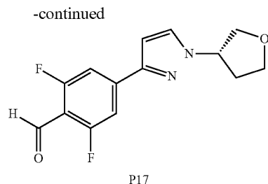
(S)-2,6-difluoro-4-(1-(tetrahydrofuran-3-yl)-1H-pyrazol-3-yl)benzaldehyde (P17)
