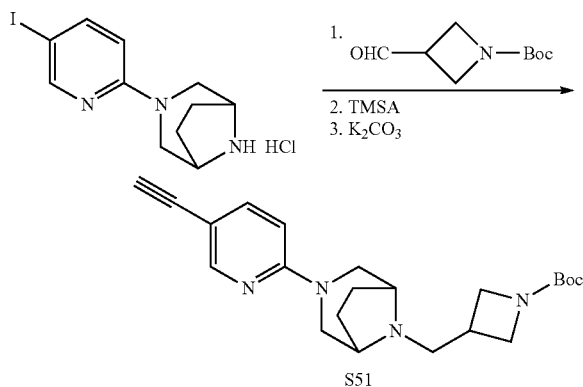
Synthesis of tert-butyl 3-((3-(5-ethynylpyridin-2-yl)-3,8-diazabicyclo[3.2.1]octan-8-yl)methyl)azetidine-1-carboxylate (S51)
