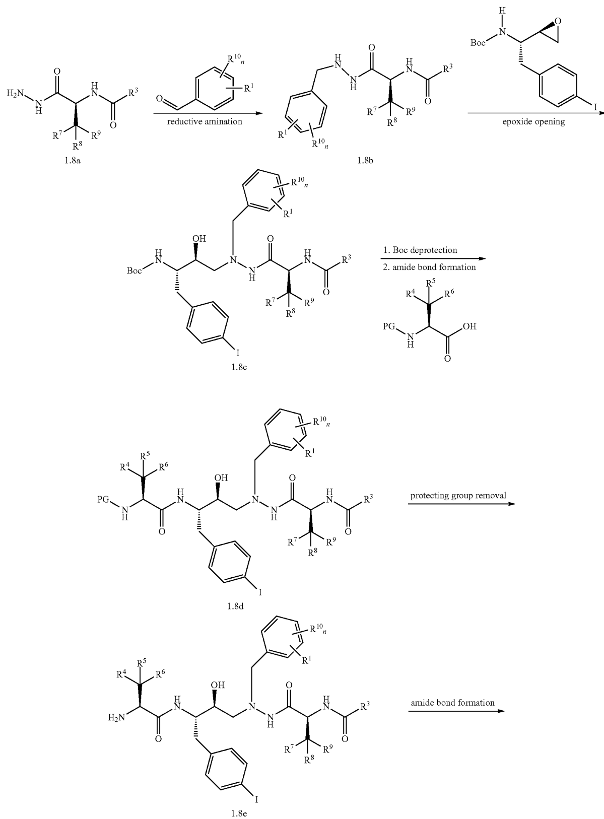
SCHEME 1.8
