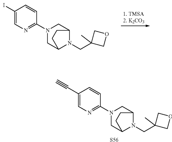
Synthesis of 3-(5-ethynylpyridin-2-yl)-8-((3-methyloxetan-3-yl)methyl)-3,8-diazabicyclo[3.2.1]octane (S56)
