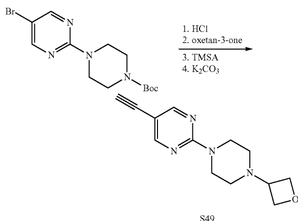
Synthesis of 5-ethynyl-2-(4-(oxetan-3-yl)piperazin-1-yl)pyrimidine (S49)
