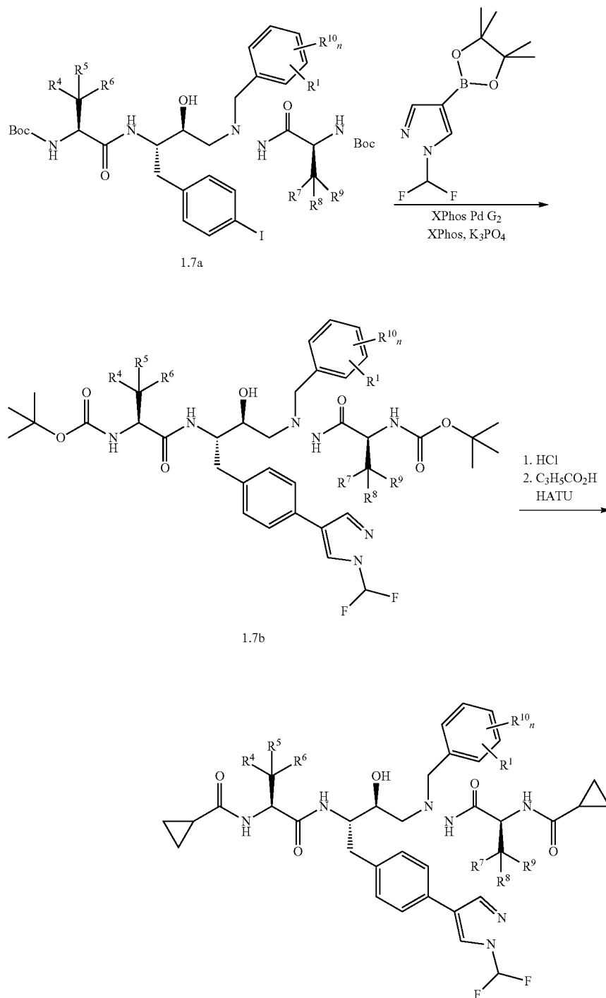
SCHEME 1.7
