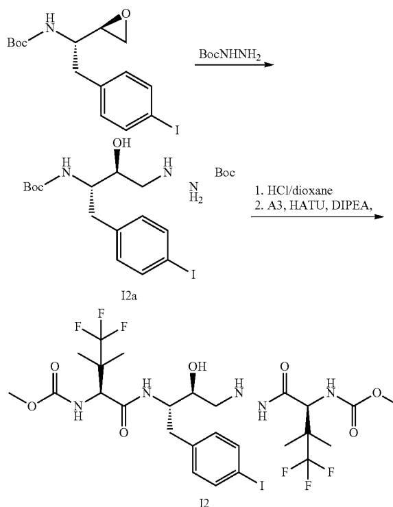
Synthesis of tert-butyl 2-((2S,3S)-3-((tert-butoxycarbonyl)amino)-2-hydroxy-4-(4-iodophenyl)butyl)hydrazine-1-carboxylate (12a)
