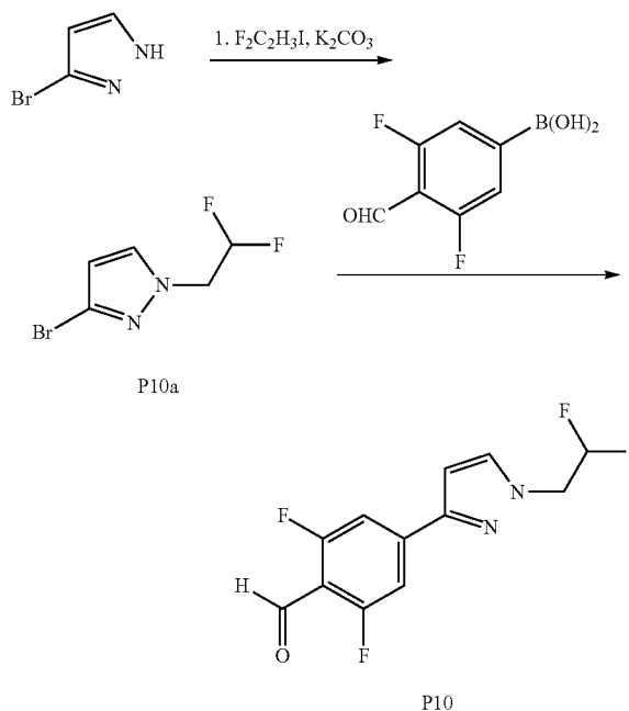
Synthesis of 3-bromo-1-(2,2-difluoroethyl)-1H-pyrazole (P10a)
