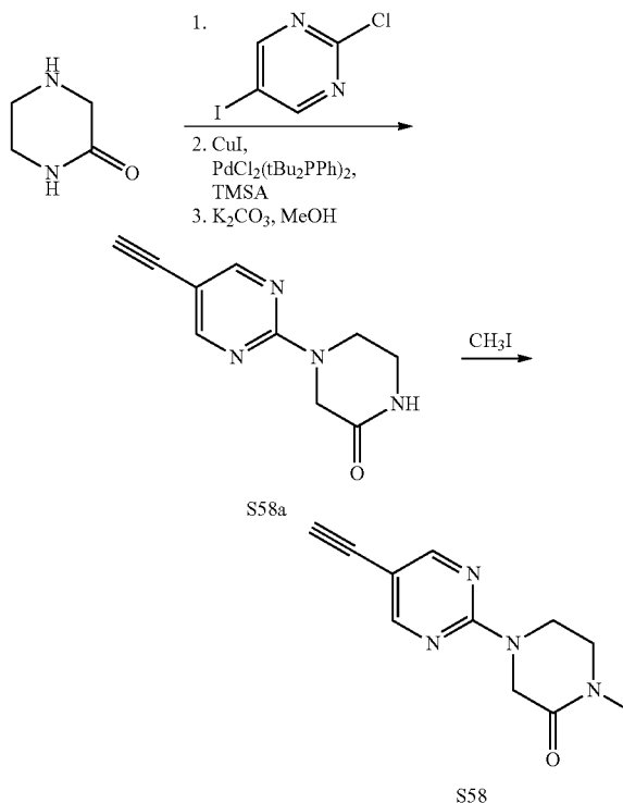
Synthesis of 4-(5-ethynylpyrimidin-2-yl)piperazin-2-one (S58a)
