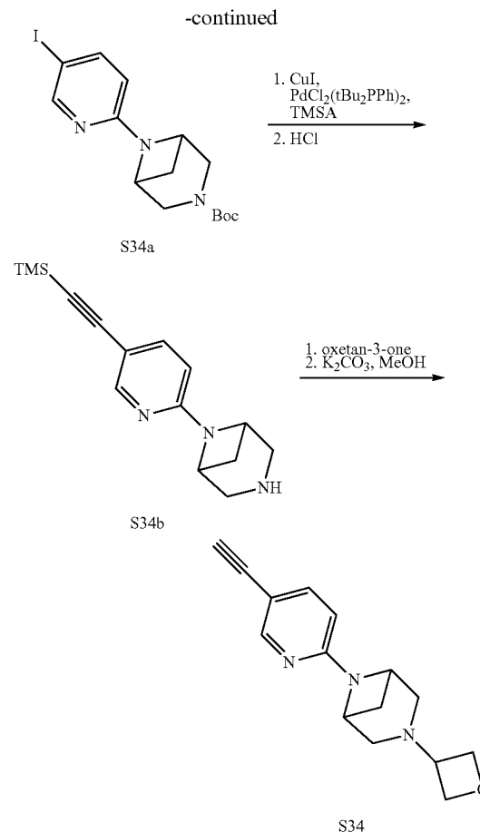
Synthesis of tert-butyl 6-(5-iodopyridin-2-yl)-3,6-diazabicyclo[3.1.1]heptane-3-carboxylate (S34a)
