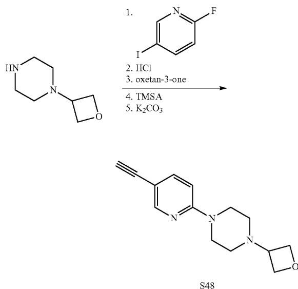
Synthesis of 1-(5-ethynylpyridin-2-yl)-4-(oxetan-3-yl)piperazine (S48)
