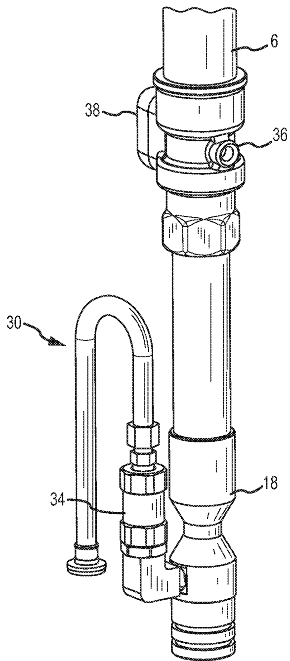
FIG.4 (PRIOR ART)
