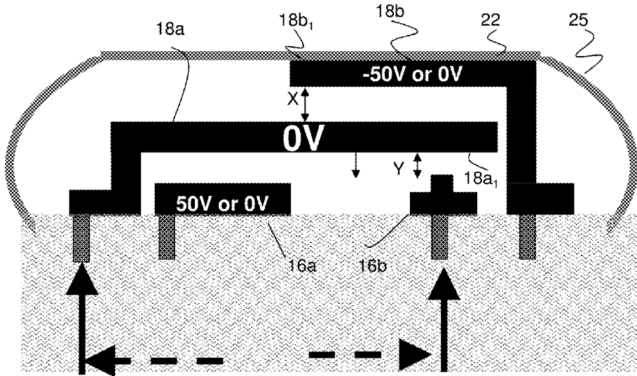
Sense open or closed switch
