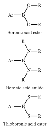
Scheme 1: Structures of some boronic acid and borinic acid derivatives
