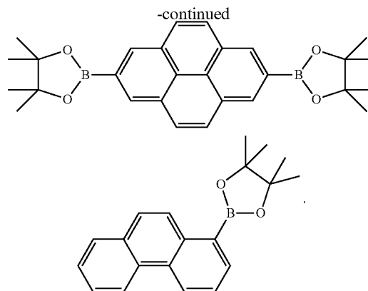
38. A compound of formulae (27), (27a), and (28)
