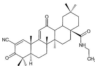
CDDO-EA
