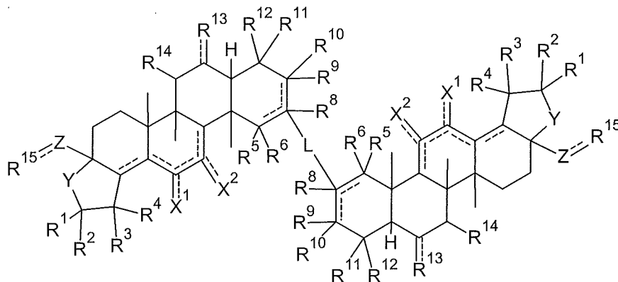
Formula II
