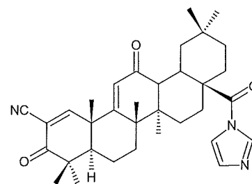
CDDO-Im
