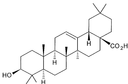
Oleanolic Acid
