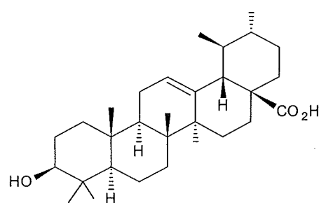
Ursolic Acid
