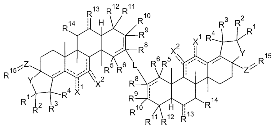
Formula II
