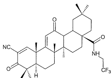
CDDO-TFEA
