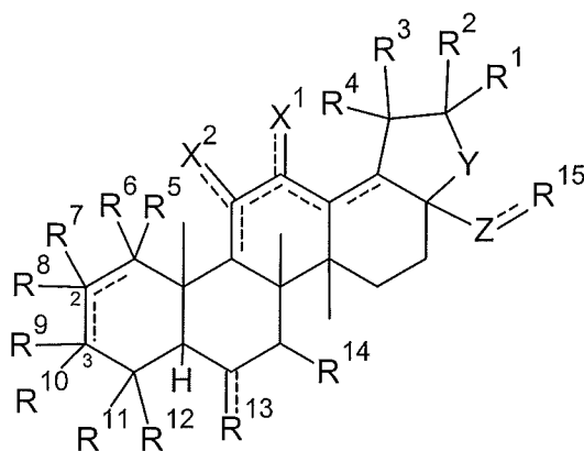
Formula I
