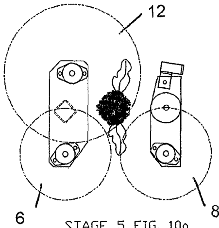
STAGE 5 FIG. 10a PLAN VIEW
