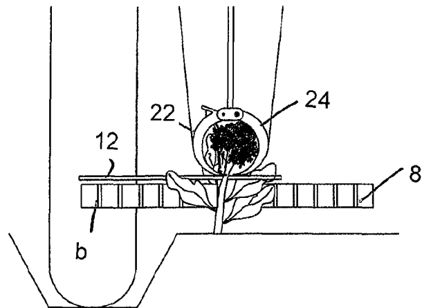
STAGE 4 - FIG. 9b FRONT VIEW
