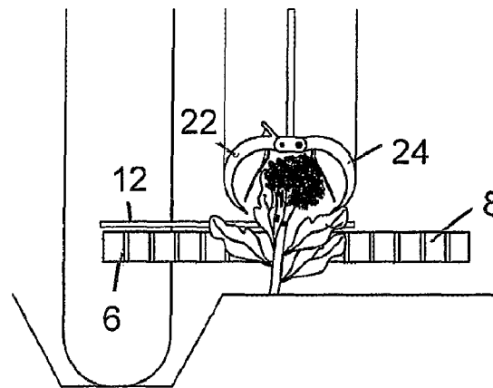
STAGE 1 - FIG. 6b FRONT VIEW
