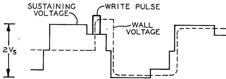
FIG. 1 (PRIOR ART)
