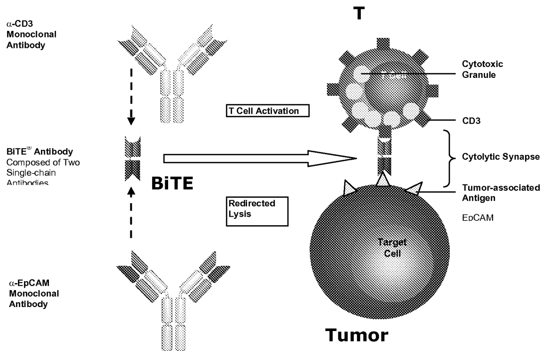
Fig. 3: Generation of MT110 and Mode of Action
