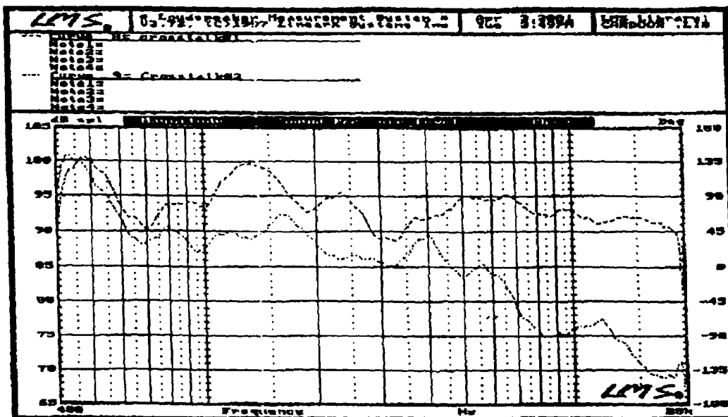
Figure 8 Cross Talk comparison of standard speaker vs directional transducer mounted in orientation described by invention
