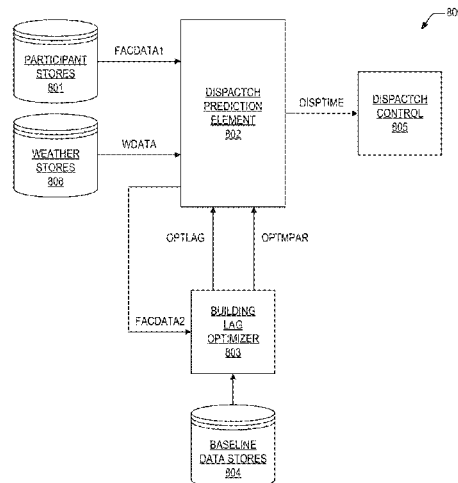
DEMAND RESPONSE DISPATCH PREDICTION SYSTEM
