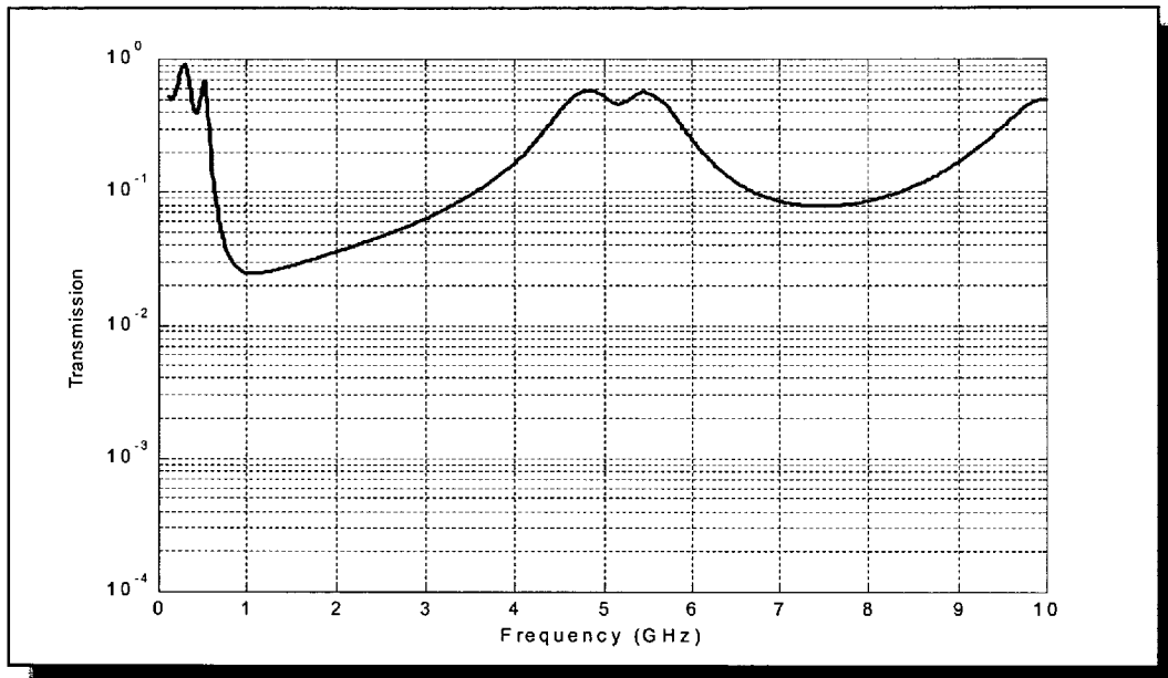
Figure 15(b) Rinner1 = 0.01 mm Rinner2 = 0.11 mm Router=0.12 mm
