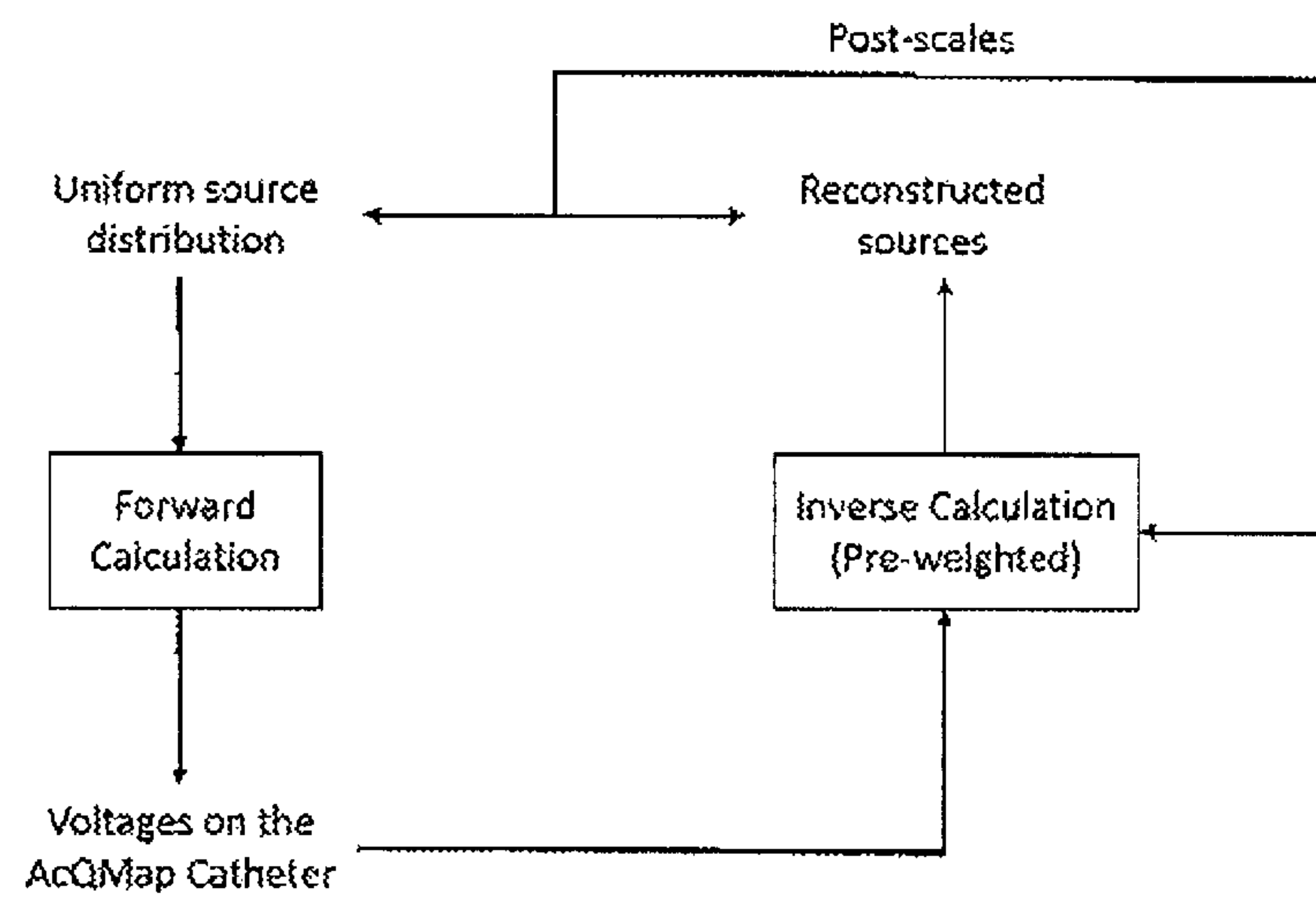
Block Diagram of a scaling algorithm.
