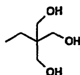
Trimethylolpropane
