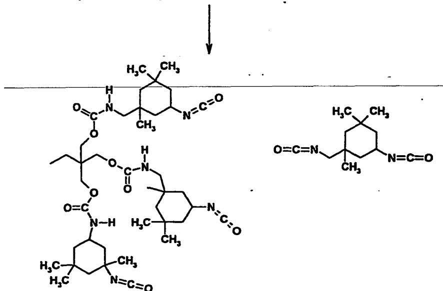
Isophorone diisocyanate
