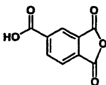
Trimellitic anhydride
