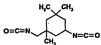
Isophorone diisocyanate
