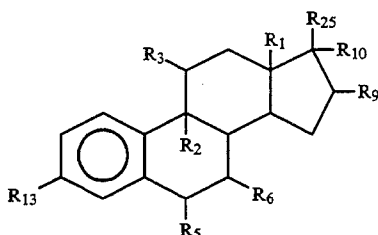
Structure [B]
