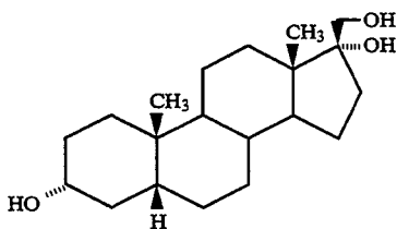
5β-ANDROSTAN-3α,17α,20-TRIOIOL
