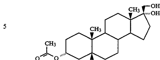
3α-ACETOXY-5β-ANDROSTAN-17α,20-DIOL
