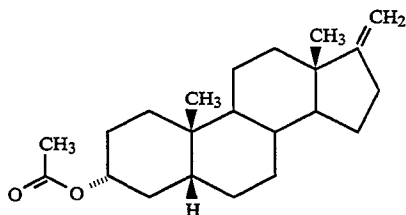
3α-ACETOXY-5β-ANDROST-17(20)-ENE
