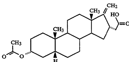
3α-ACETOXY-5β-ANDROST-17(20)-EN-16-ACETIC ACID
