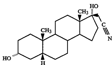
17β-(CYANOMETHYL)-5β-ANDROSTAN-3α,17α-DIOL
