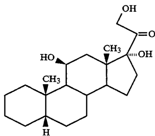
5β-PREGNAN-11β,17α,21-TRIOL-20-ONE
