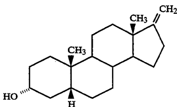
5β-ANDROST-17(20)-EN-3α-OL
