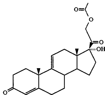
4,9(11)-PREGNADIEN-17α,21-DIOL-3,20-DIONE-21-ACETATE
