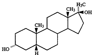
17α-METHYL-5β-ANDROSTAN-3α,17β-DIOL
