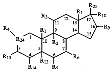
Structure [A]
