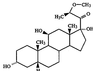
21-METHYL-5β-PREGNAN-3α,11β,17α, 21-TETROL-20-ONE 21-METHYL ETHER
