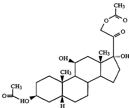
3β-ACETAMIDO-21-ACETOXY-5β- PREGNAN-11β,17α-DIOL-20-ONE
