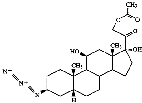
3β-AZIDO-21-ACETOXY-5β-PREGNAN- 11β,17α-DIOL-20-ONE
