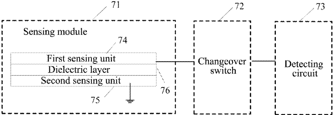
Capacitance detection module 70
