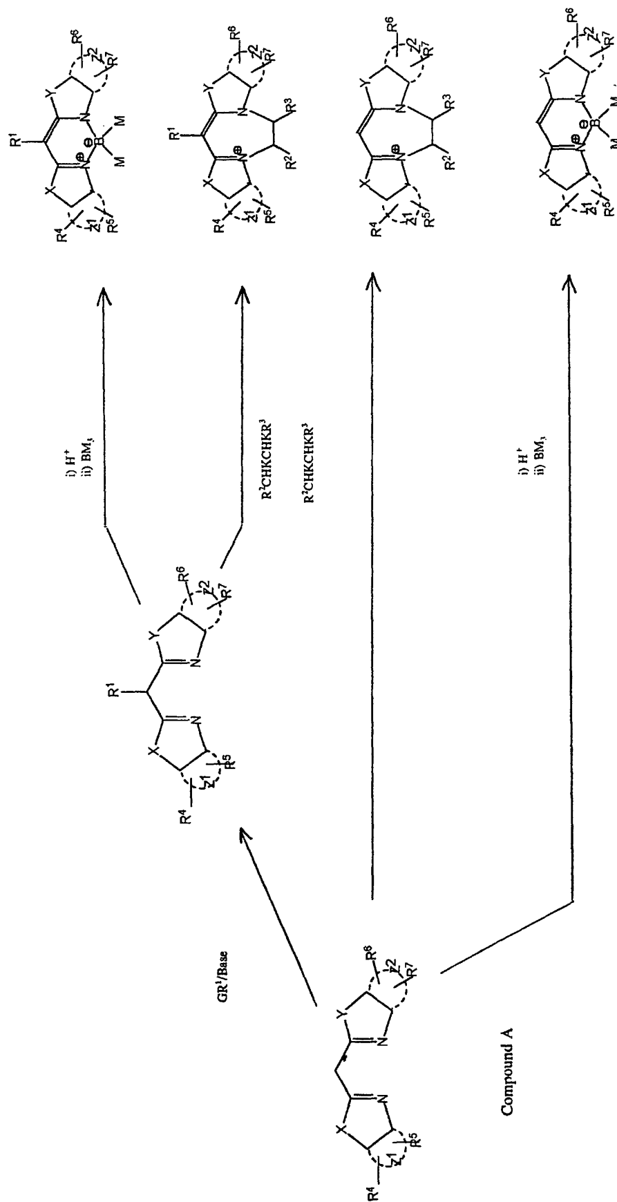
Reaction Scheme 1(c): Asymmetric Compounds
