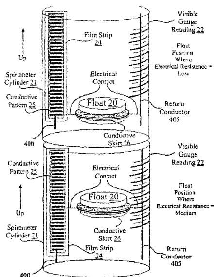
Performed Embodiment of Spirometer Gauge 2
