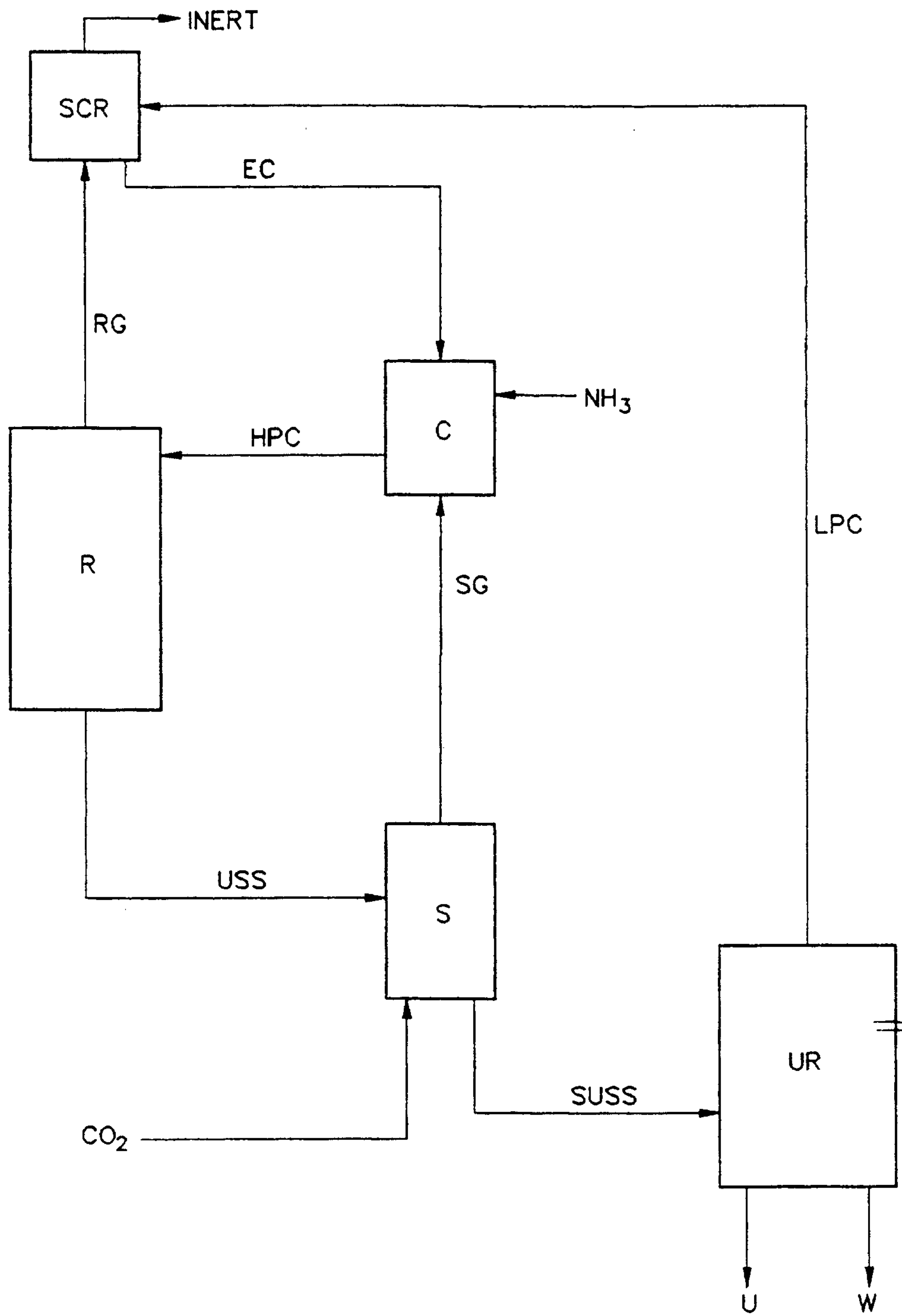
FIG. 1 (PRIOR ART)
