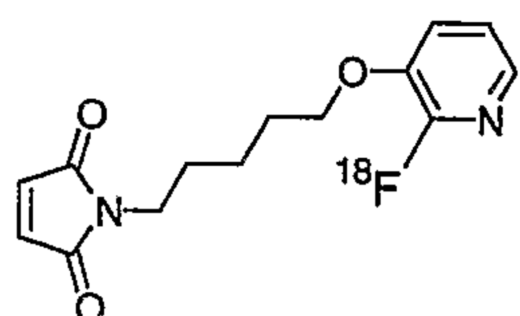
1-[5-(2-[ 18 F]fluoro-pyridin-3-yloxy)-pentyl]-pyrrole-2,5-dione
