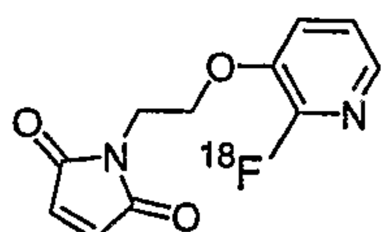
1-[2-(2-[ 18 F]fluoro-pyridin-3-yloxy)-ethyl]-pyrrole-2,5-dione
