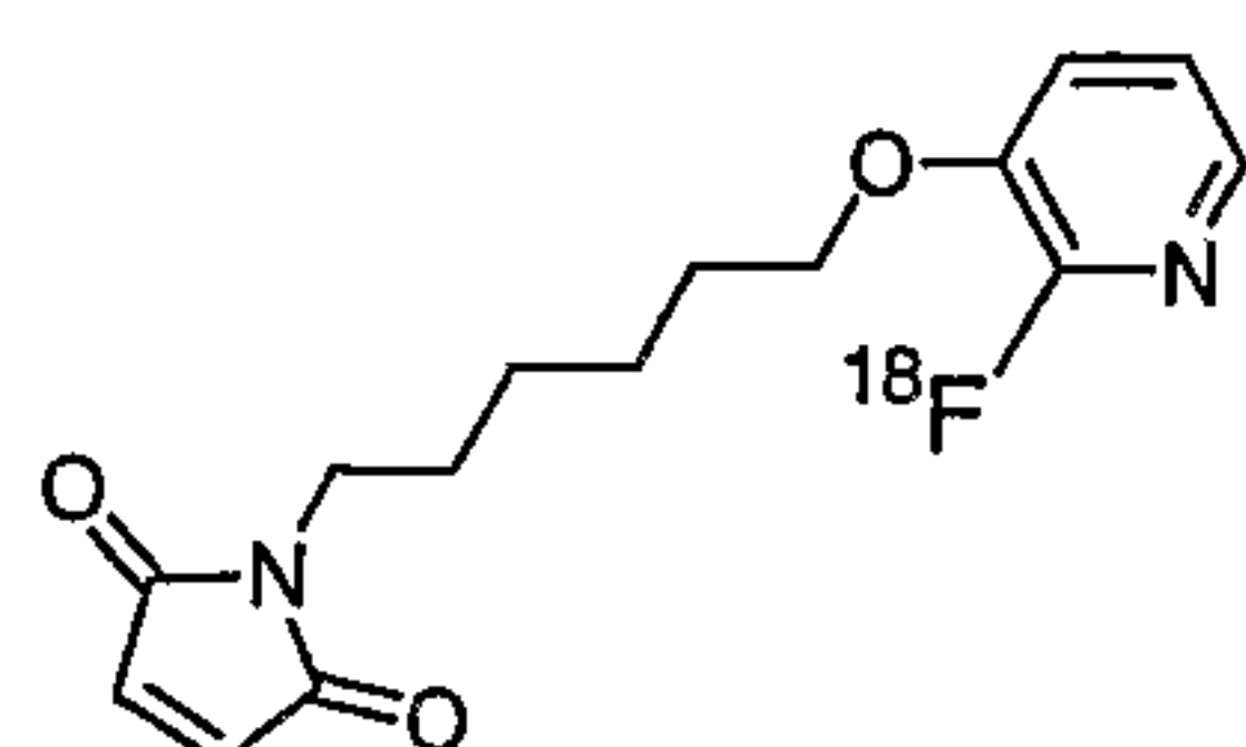
1-[6-(2-[ 18 F]fluoro-pyridin-3-yloxy)-hexyl]-pyrrole-2,5-dione
