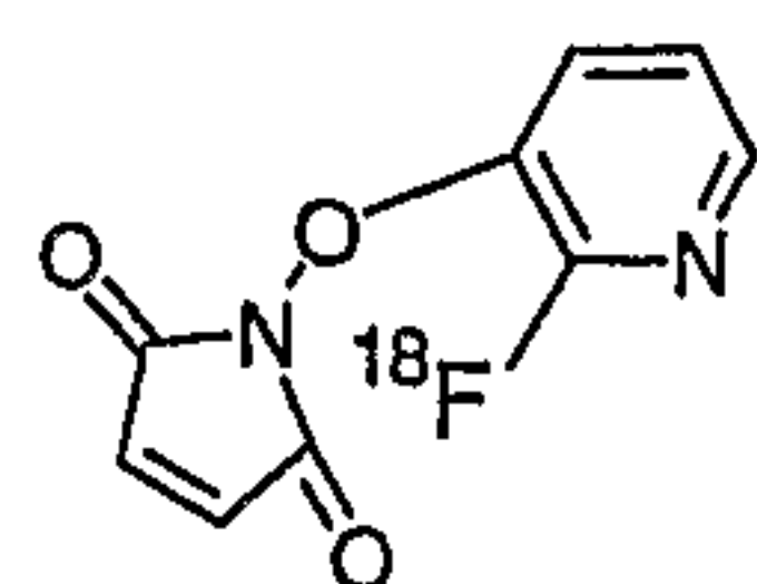
1-[(2-[ 18 F]fluoro-pyridin-3-yloxy)-methyl]-pyrrole-2,5-dione
