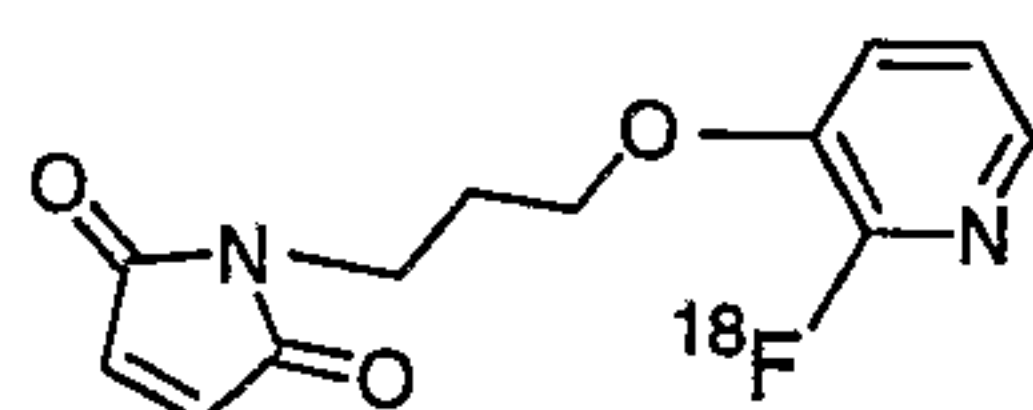
1-[3-(2-[ 18 F]fluoro-pyridin-3-yloxy)-propyl]-pyrrole-2,5-dione
