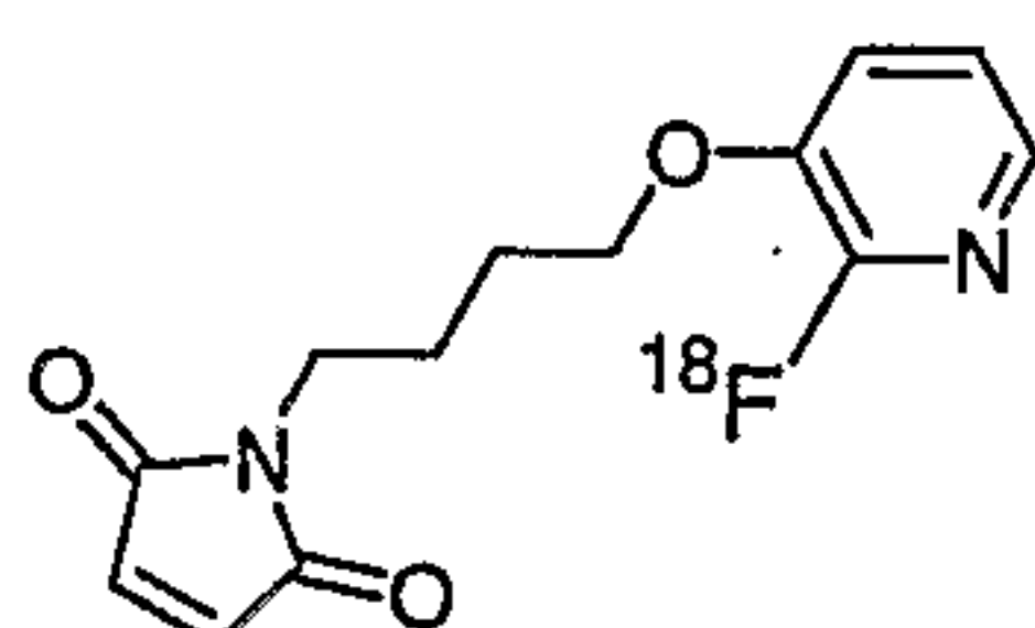
1-[4-(2-[ 18 F]fluoro-pyridin-3-yloxy)-butyl]-pyrrole-2,5-dione
