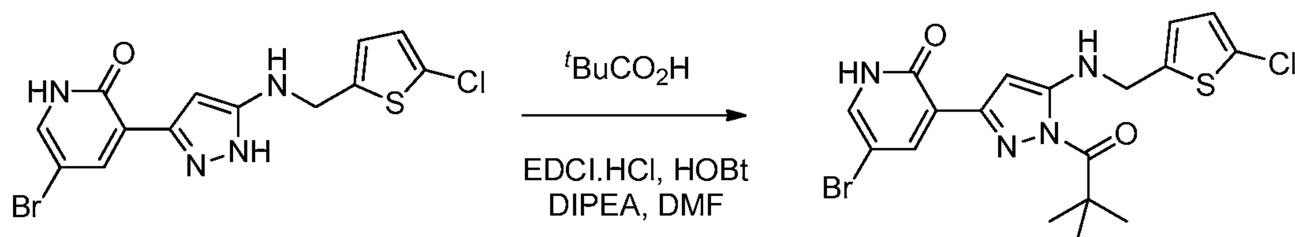
Compound 23
