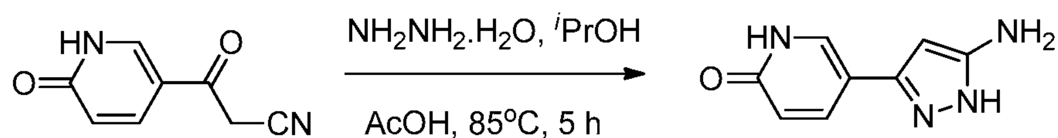
Intermediate 32
