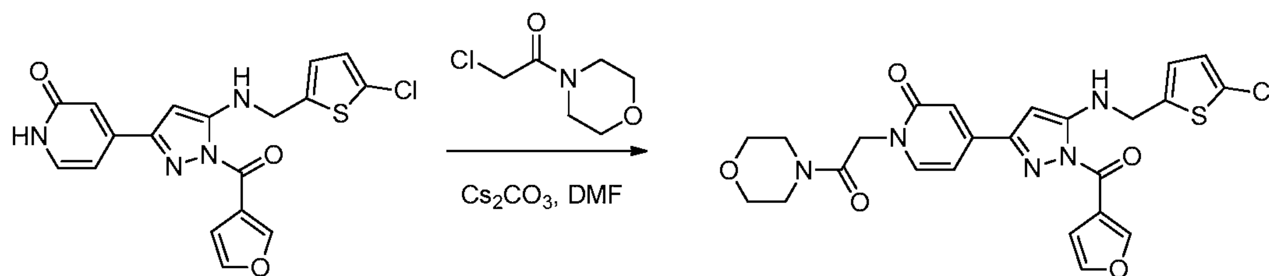
Compound 9
