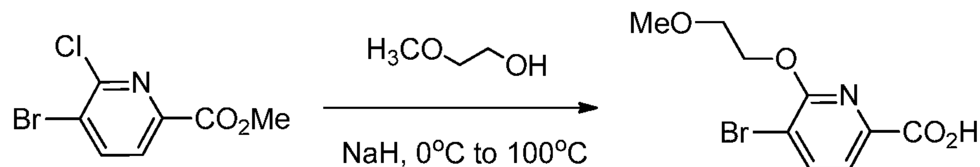
Intermediate 27
