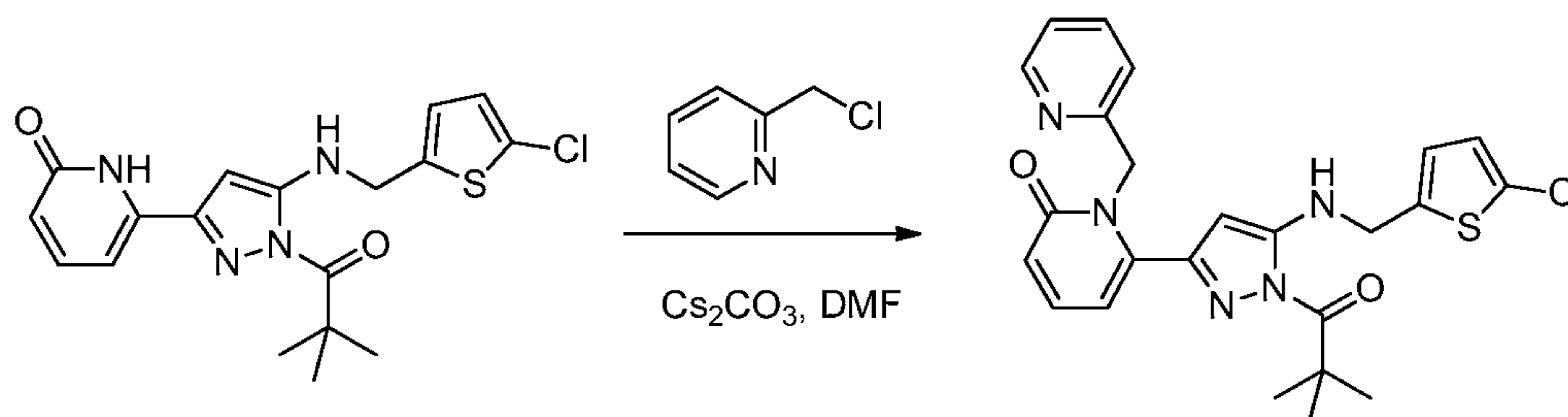
Compound 75
