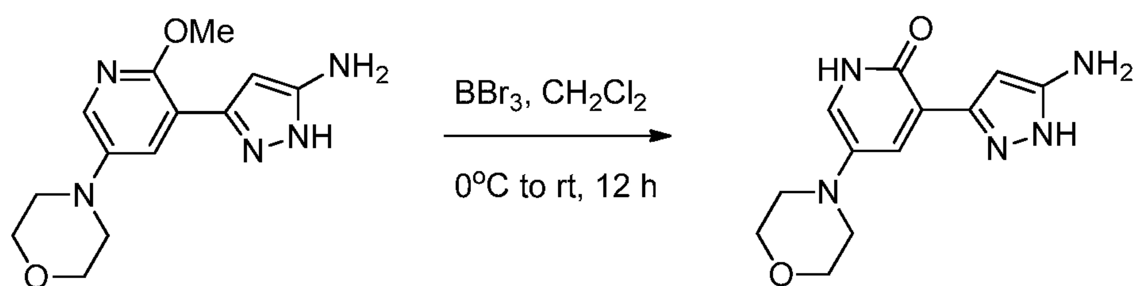
Compound 28
