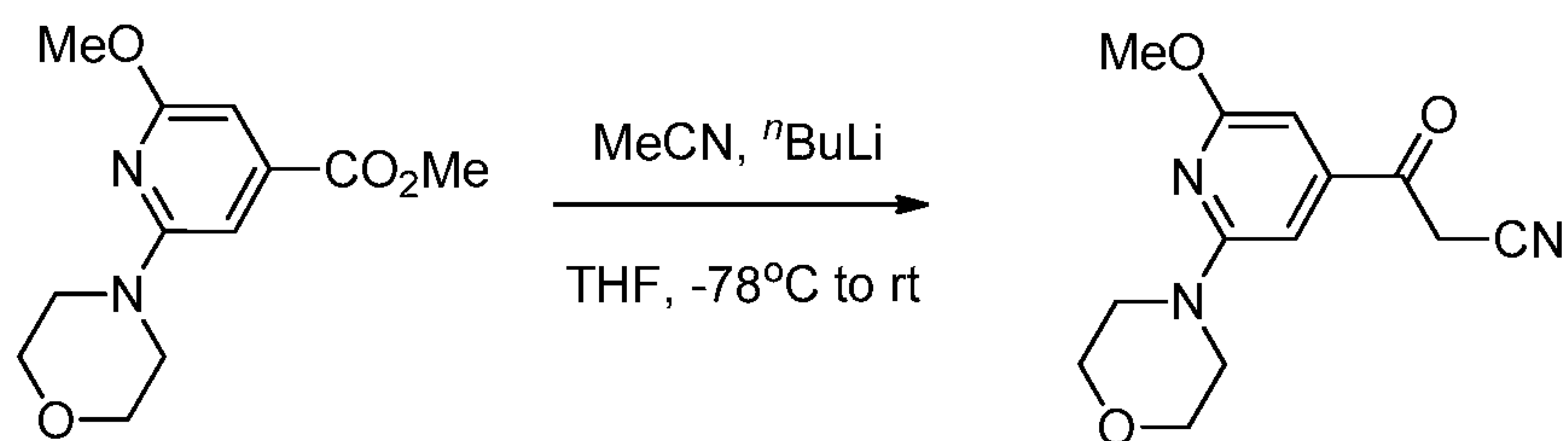
Intermediate 19
