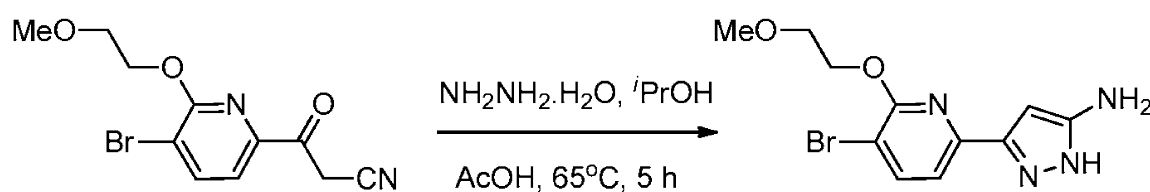
Intermediate 30
