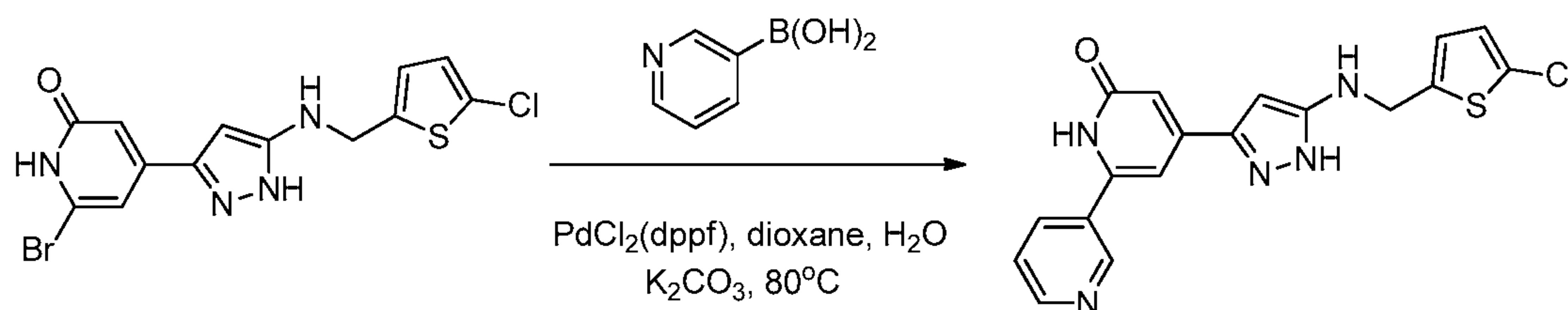
Compound 58
