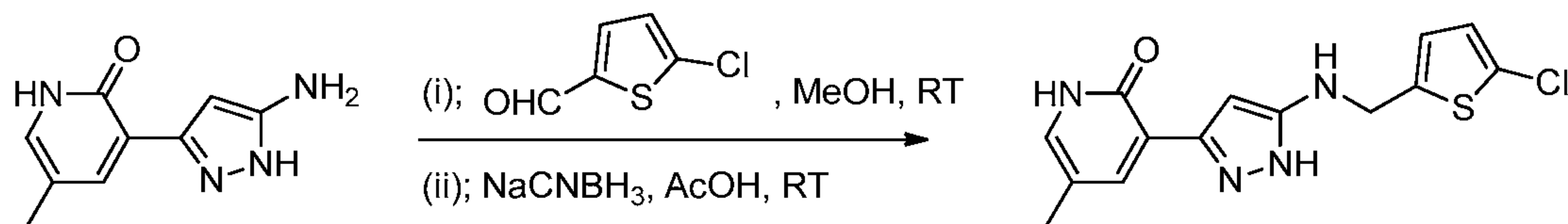
Compound 38
