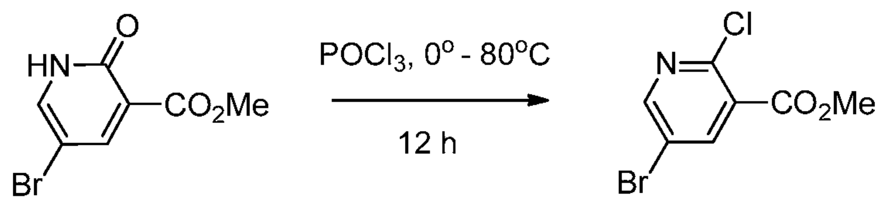
Intermediate 5
