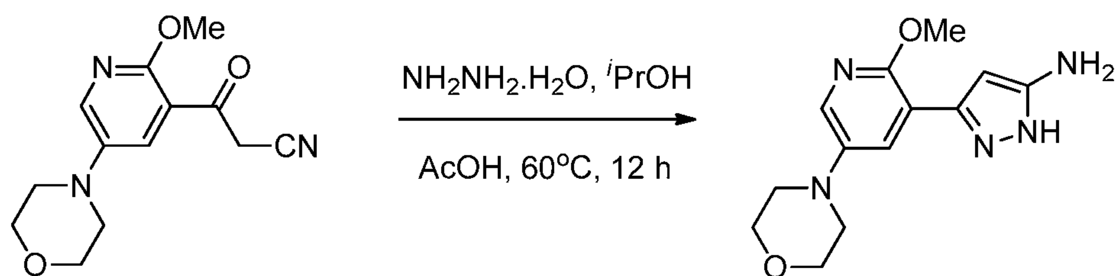
Intermediate 16
