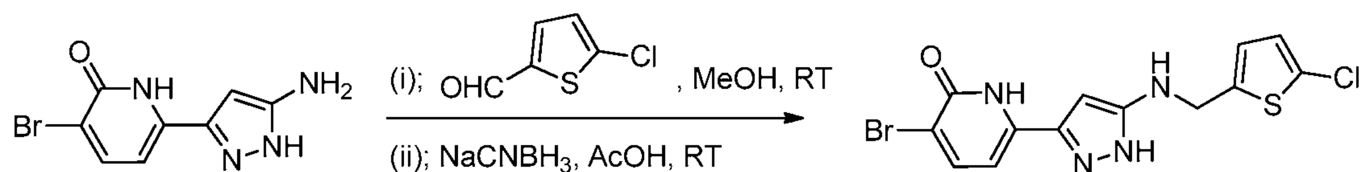
Compound 65
