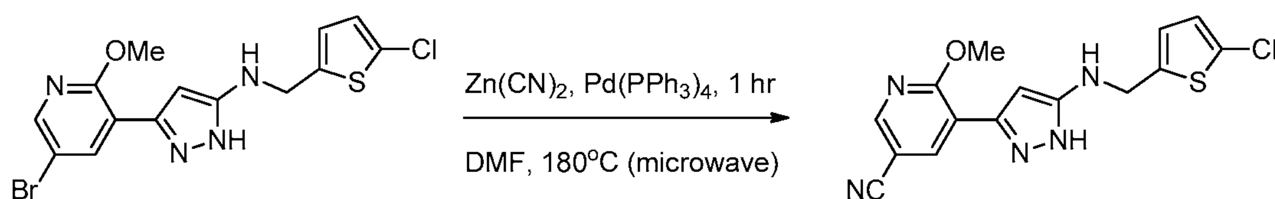
Compound 25
