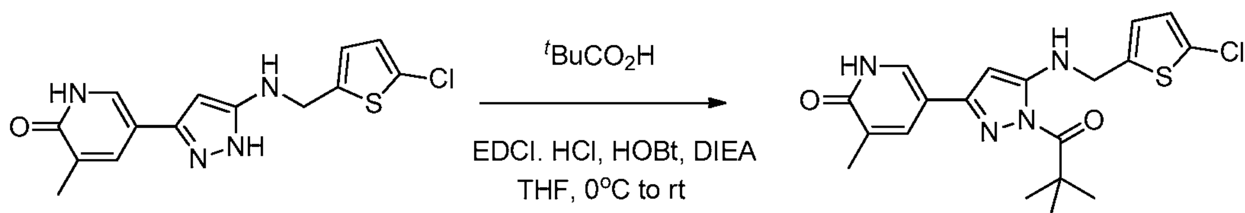
Compound 47
