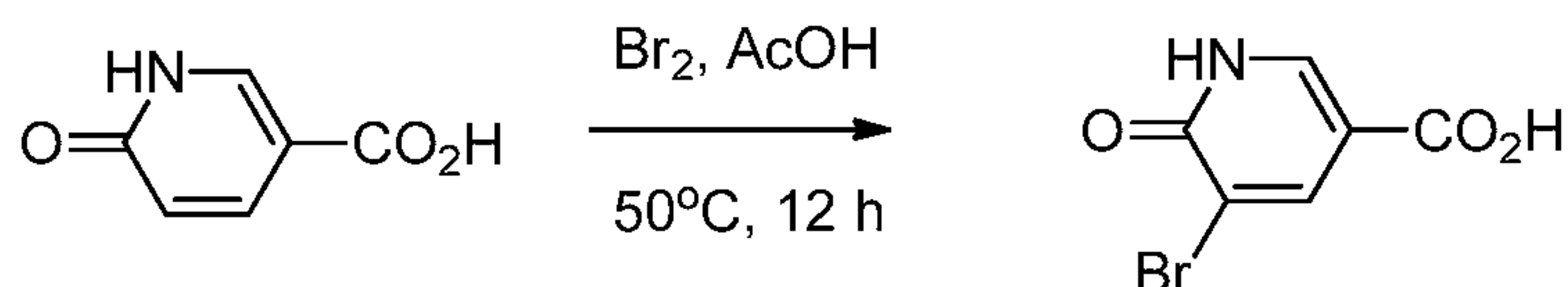
Intermediate 10
