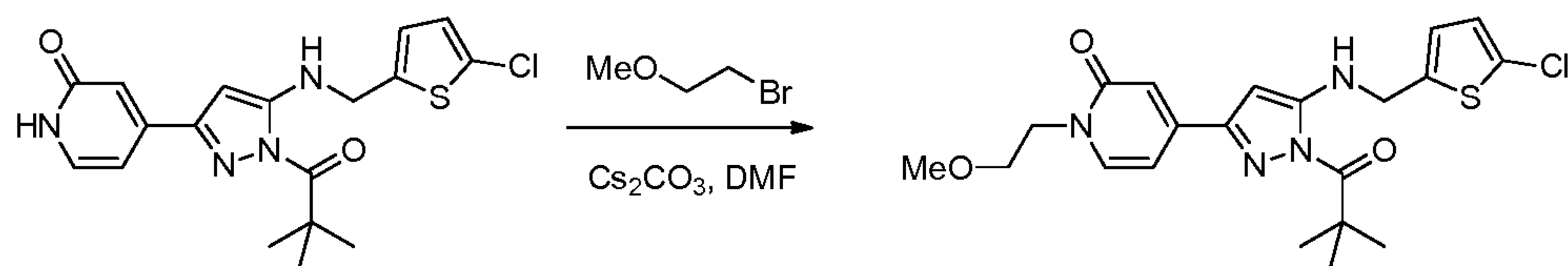
Compound 13
