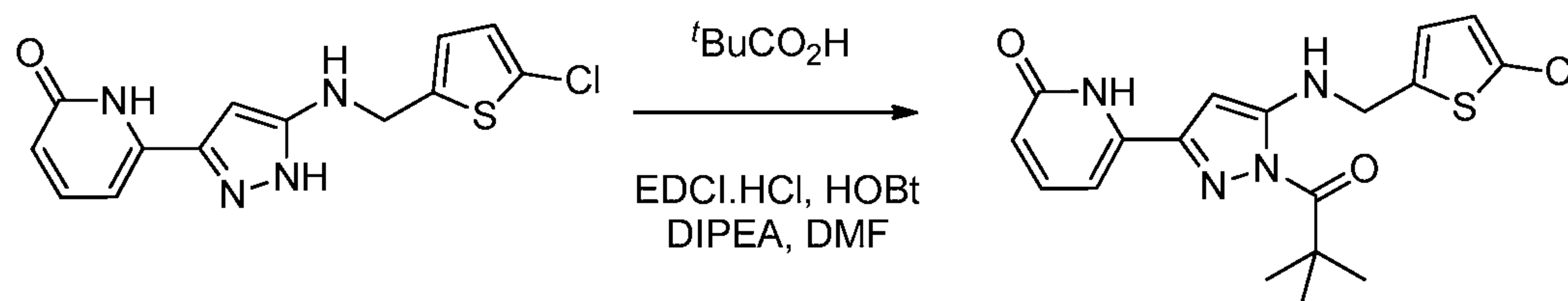
Compound 74
