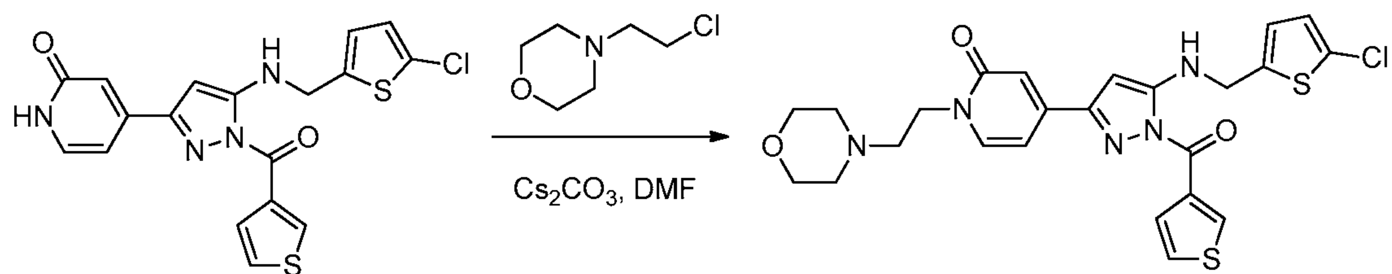
Compound 17
