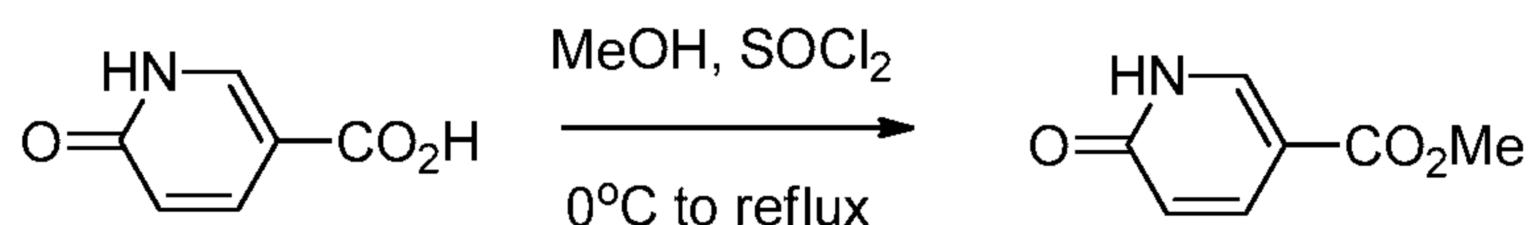
Intermediate 31
