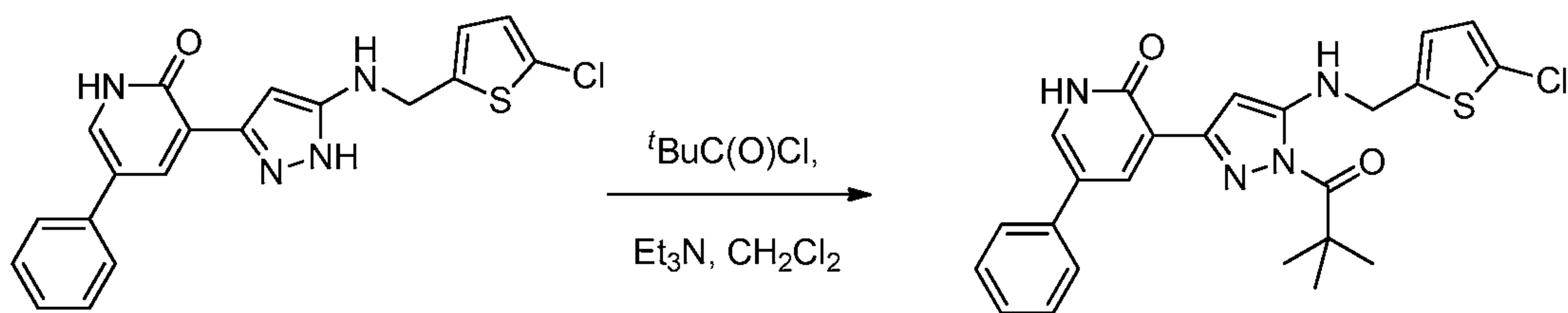
Compound 32
