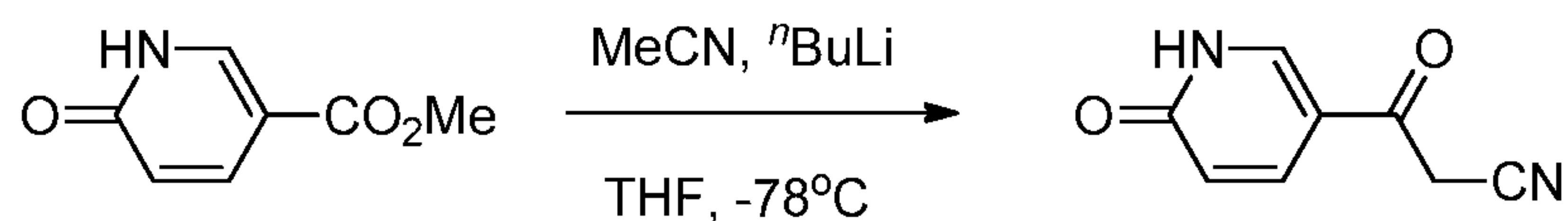
Intermediate 31
