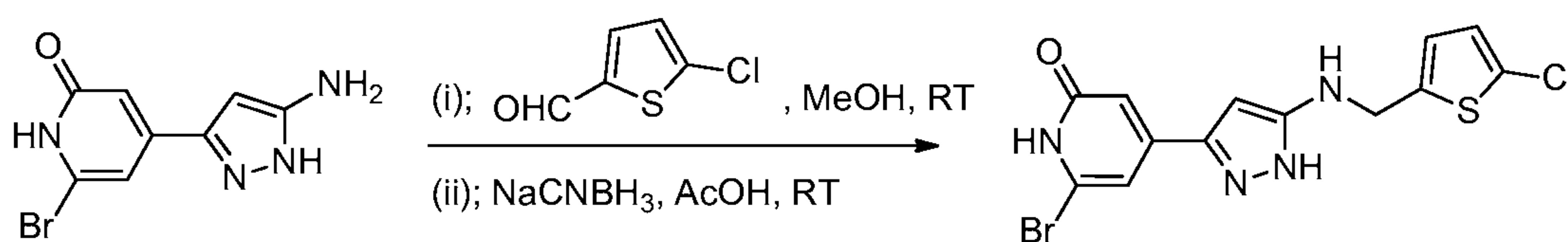
Compound 57
