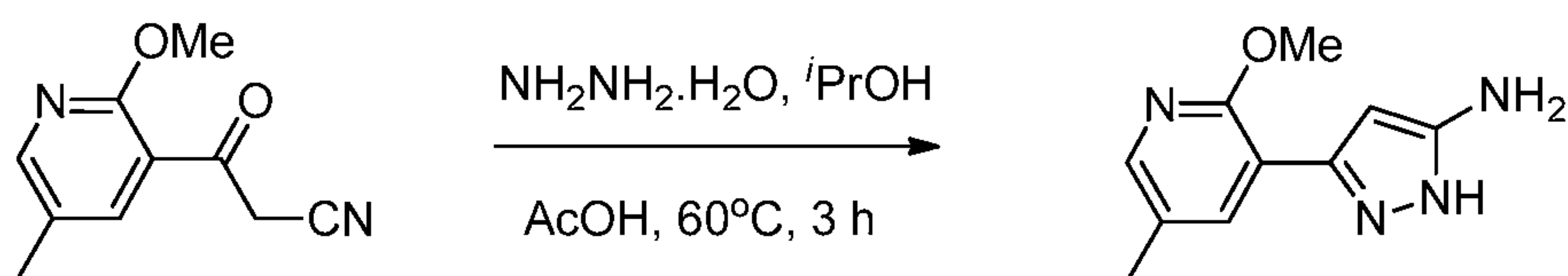
Intermediate 18
