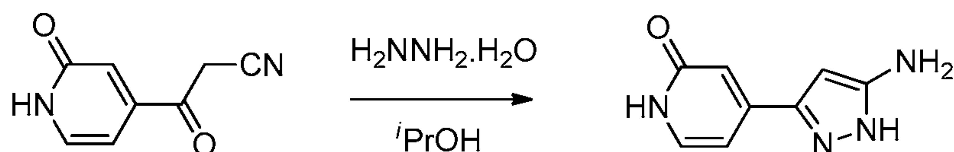
Intermediate 4
