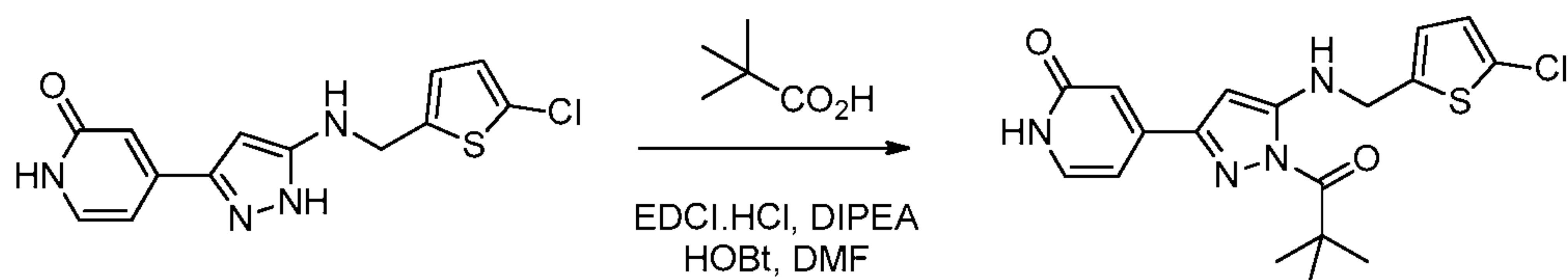
Compound 9
