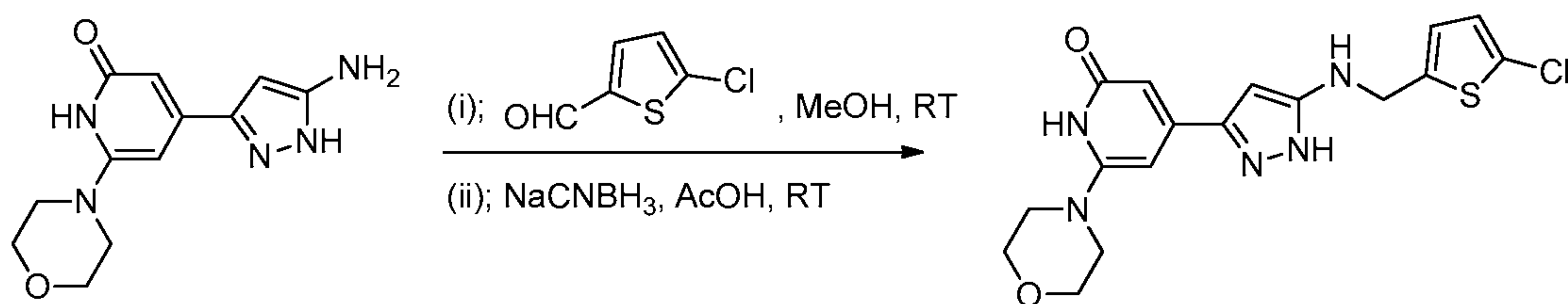
Compound 42
