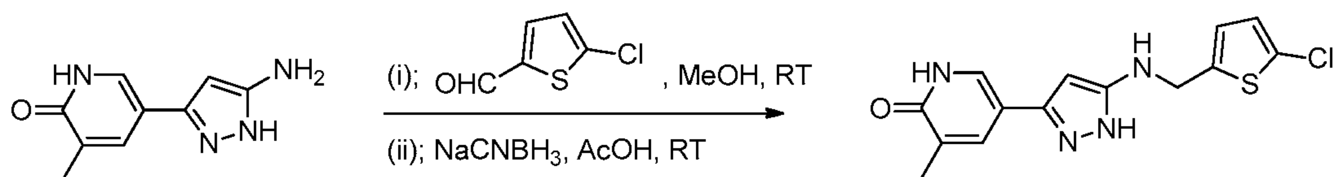
Compound 46
