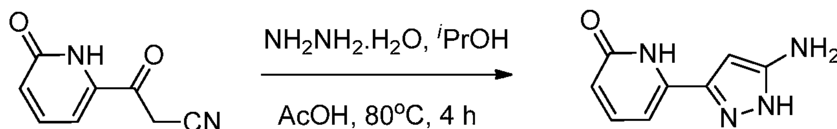
Intermediate 34
