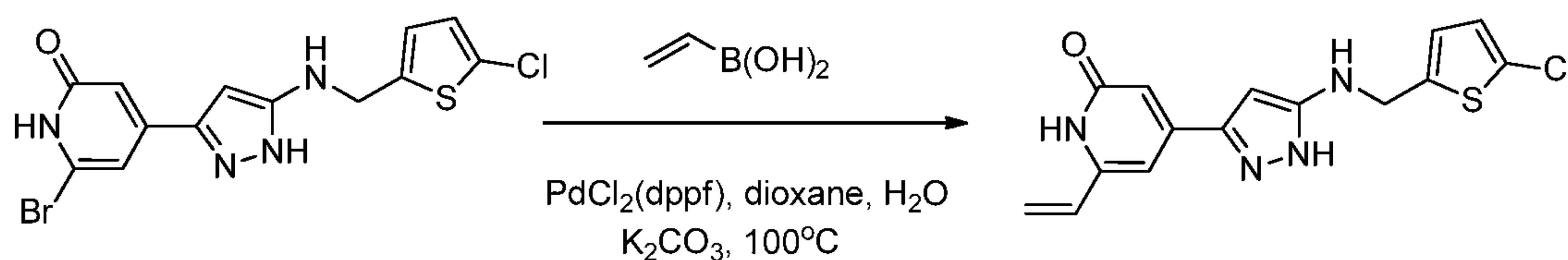
Compound 58
