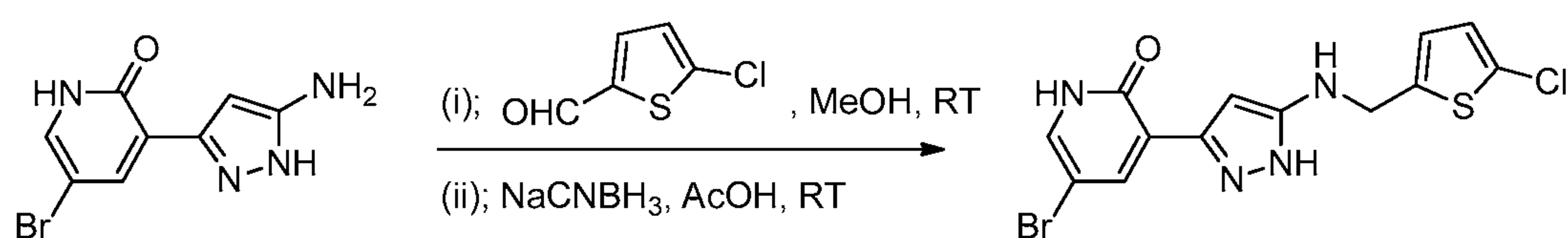
Compound 22
