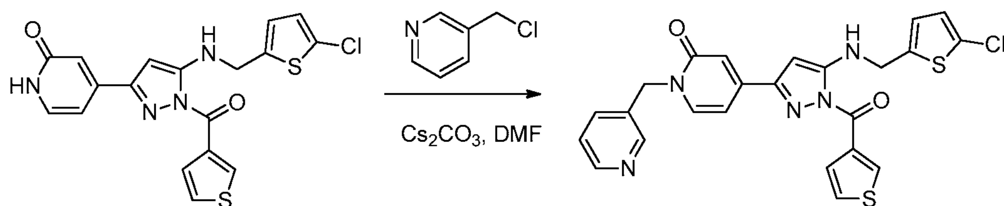
Compound 17
