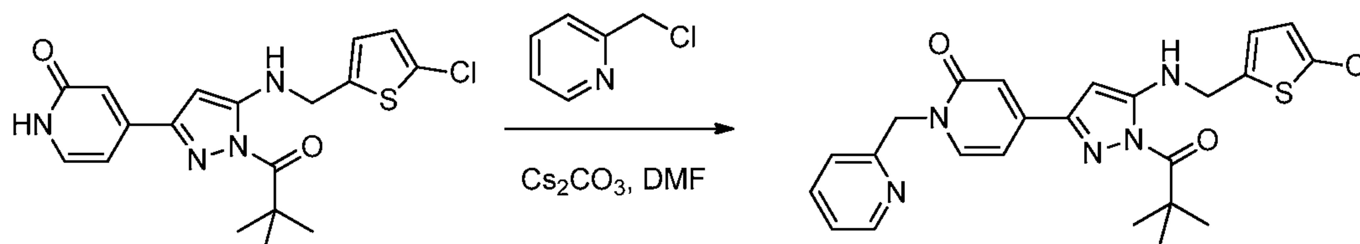
Compound 13
