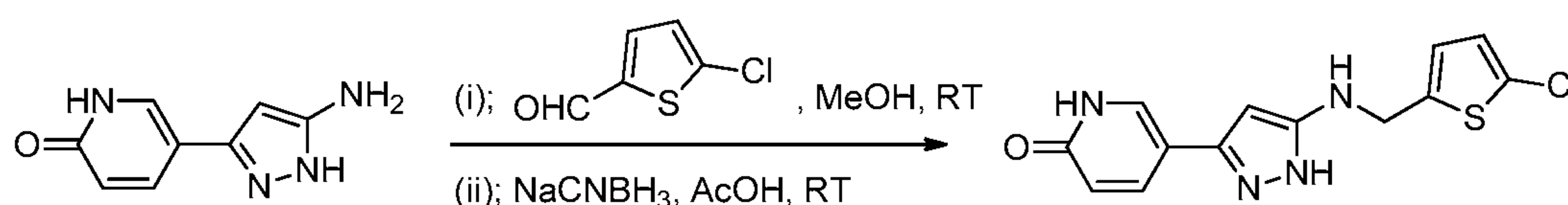
Compound 68
