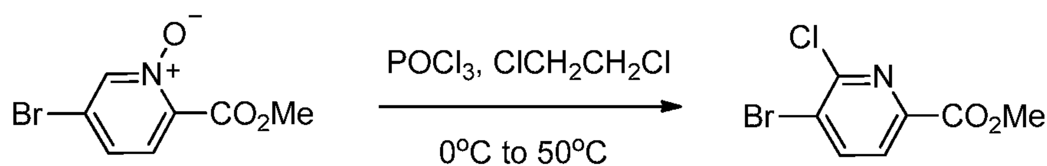
Intermediate 26
