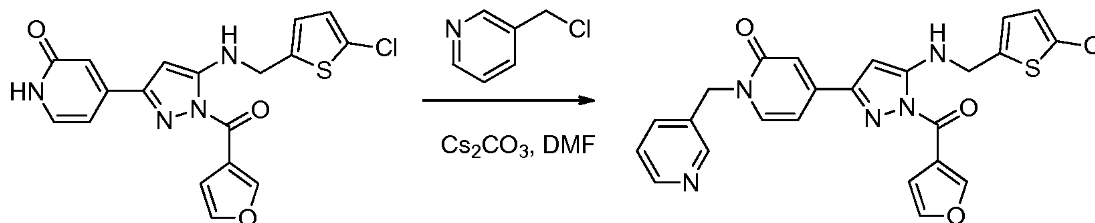
Compound 9
