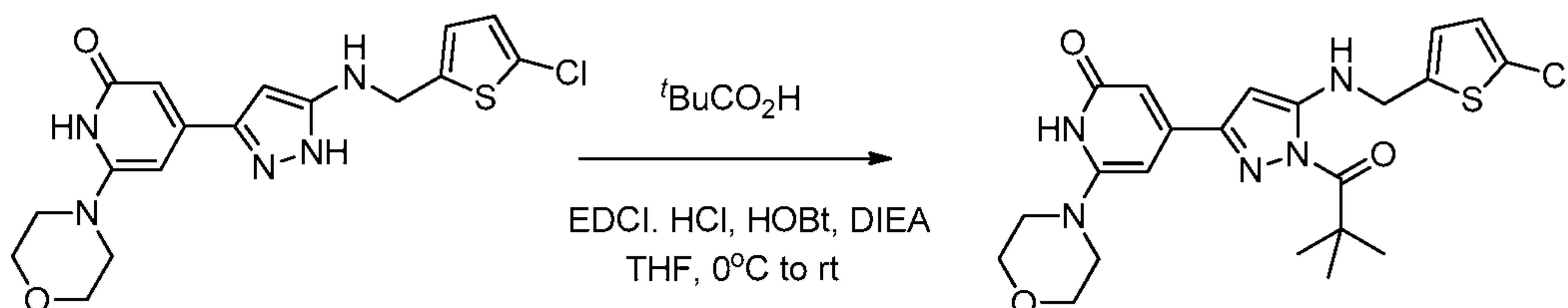
Compound 43
