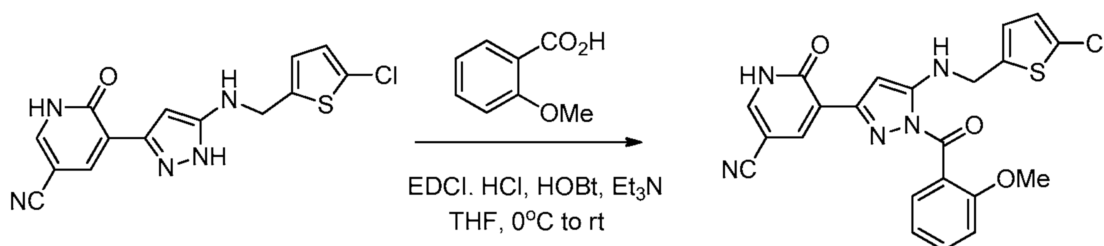
Compound 35
