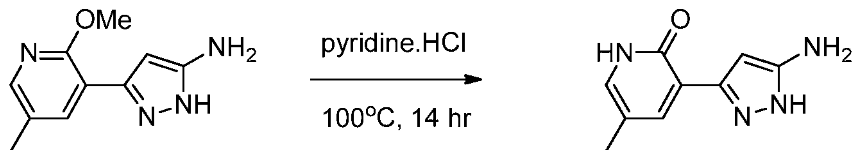
Compound 37
