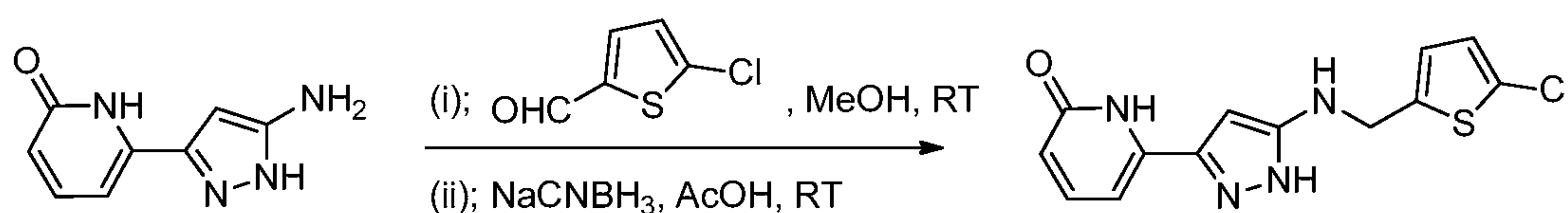
Compound 73
