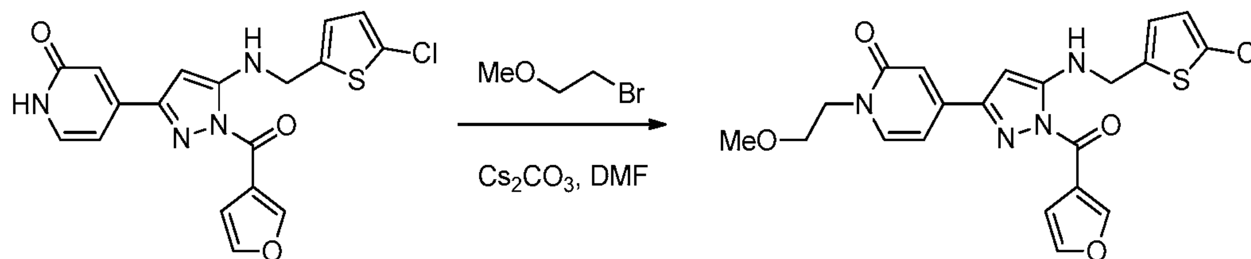
Compound 9
