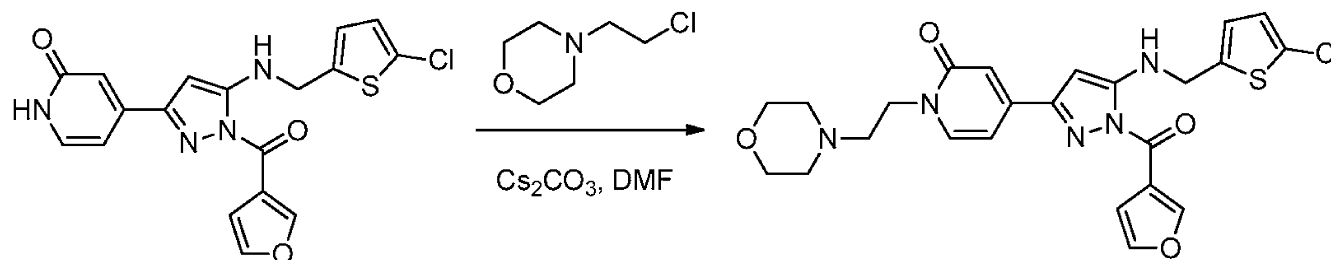
Compound 9
