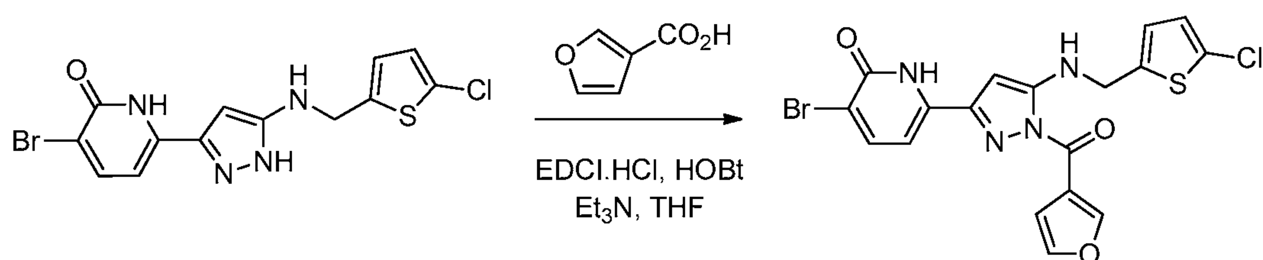
Compound 66
