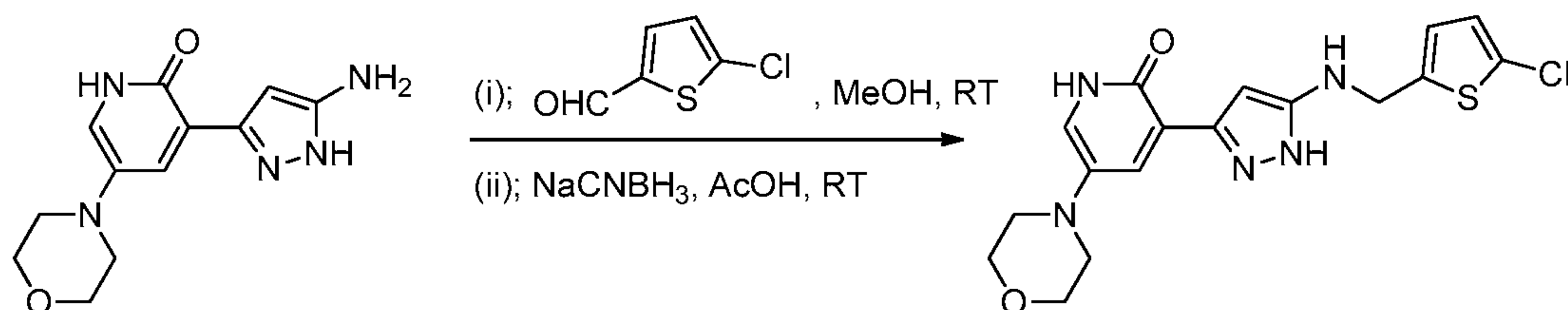
Compound 29
