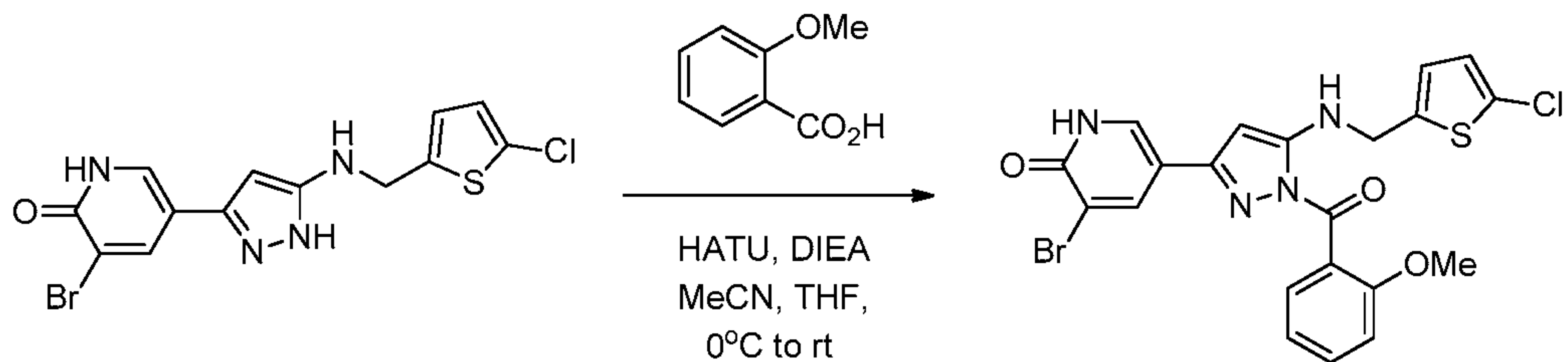
Compound 49
