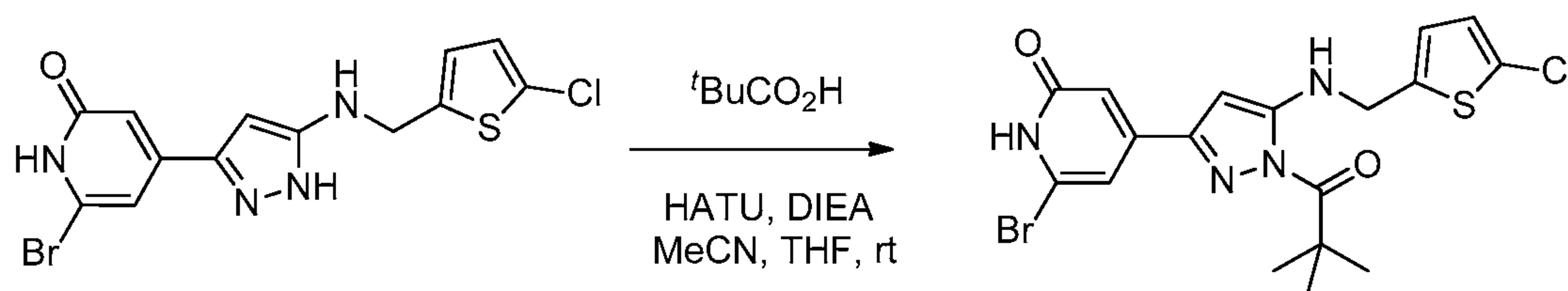
Compound 58
