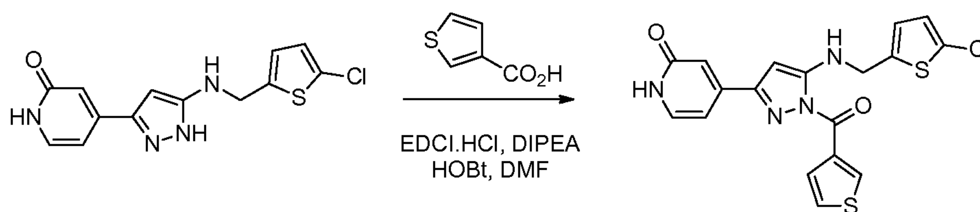
Compound 8
