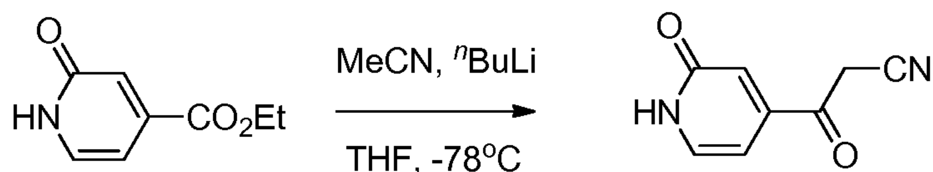
Intermediate 3
