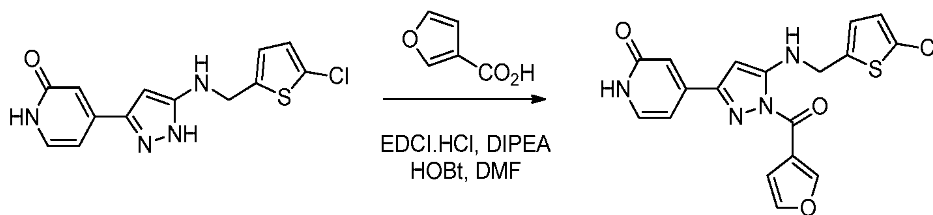
Compound 8
