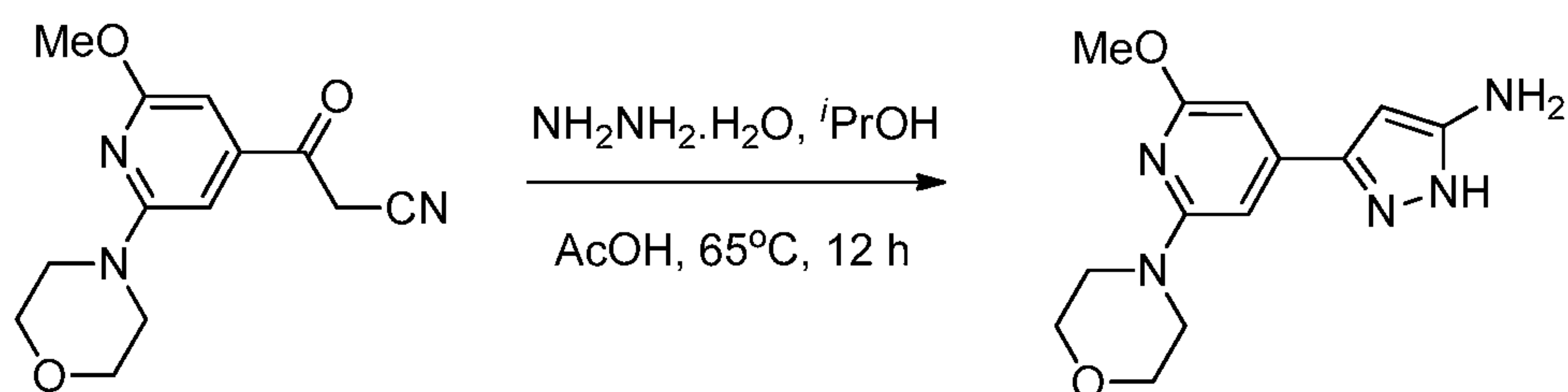
Intermediate 20
