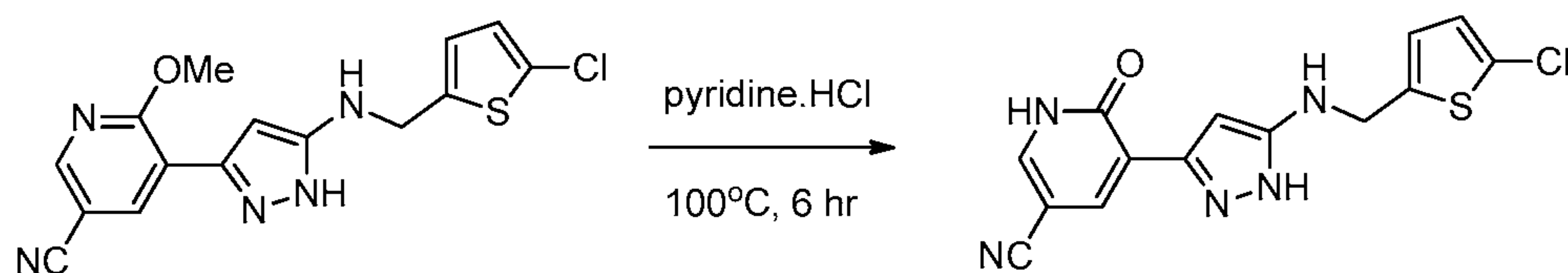
Compound 34
