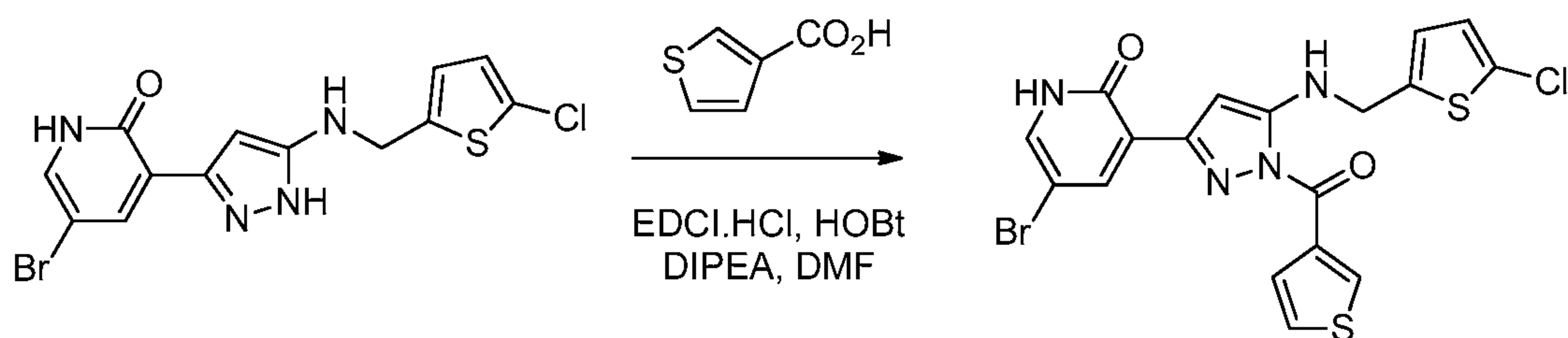
Compound 23
