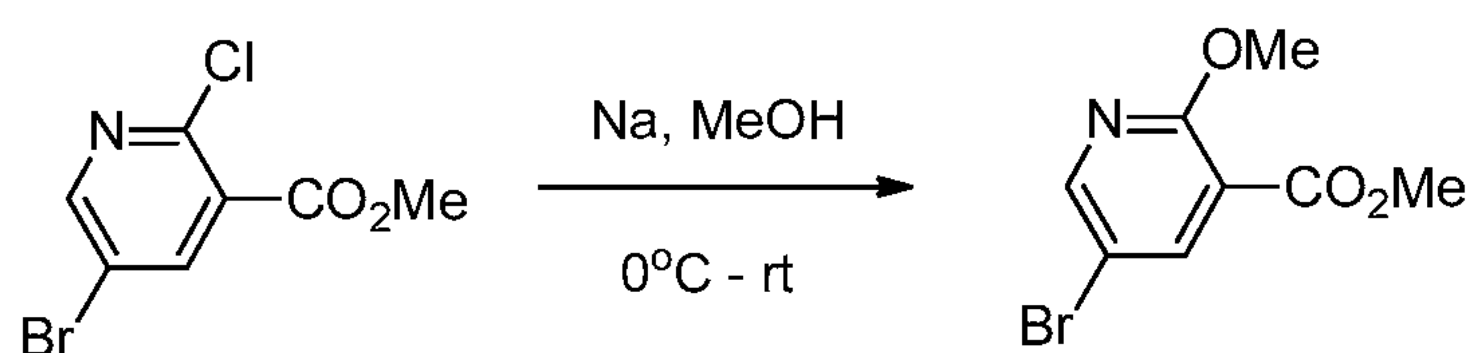
Intermediate 7
