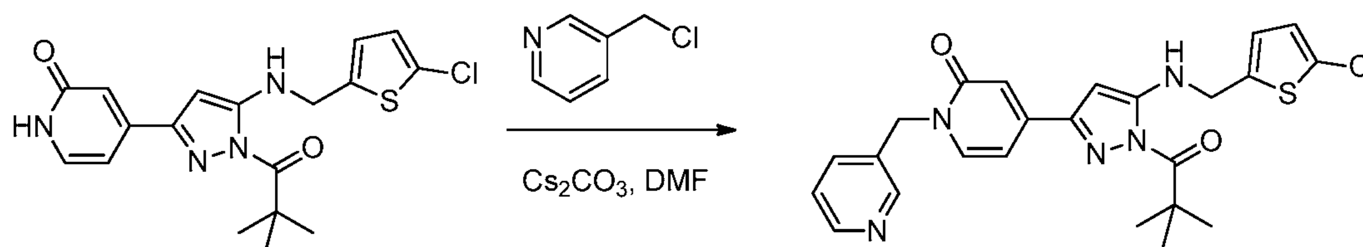
Compound 13
