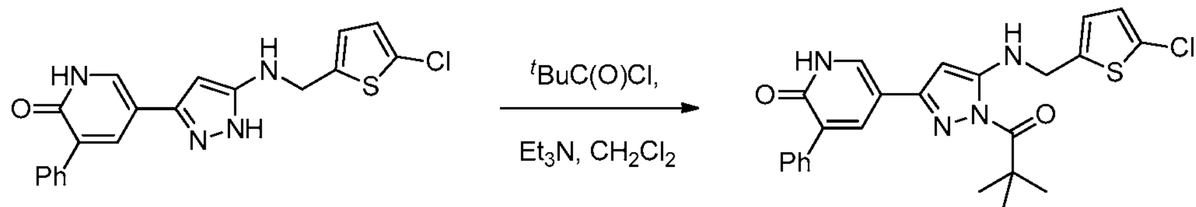
Compound 50
