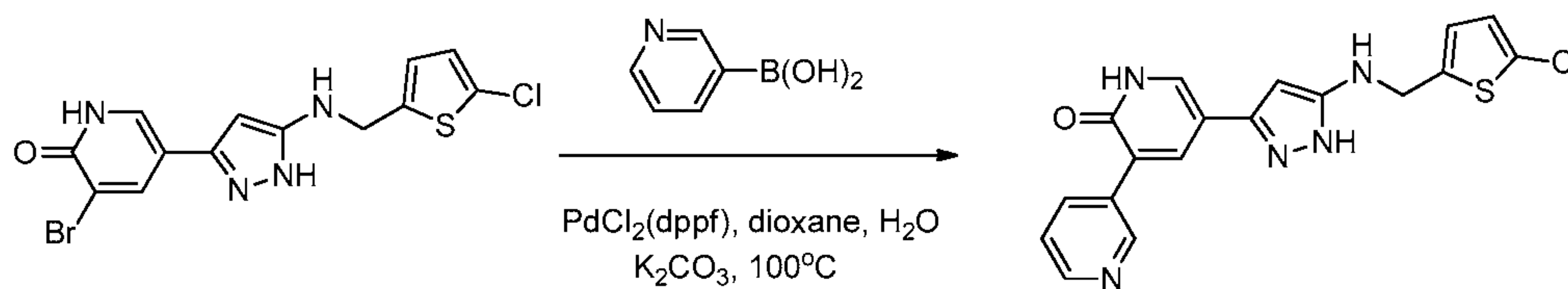
Compound 49
