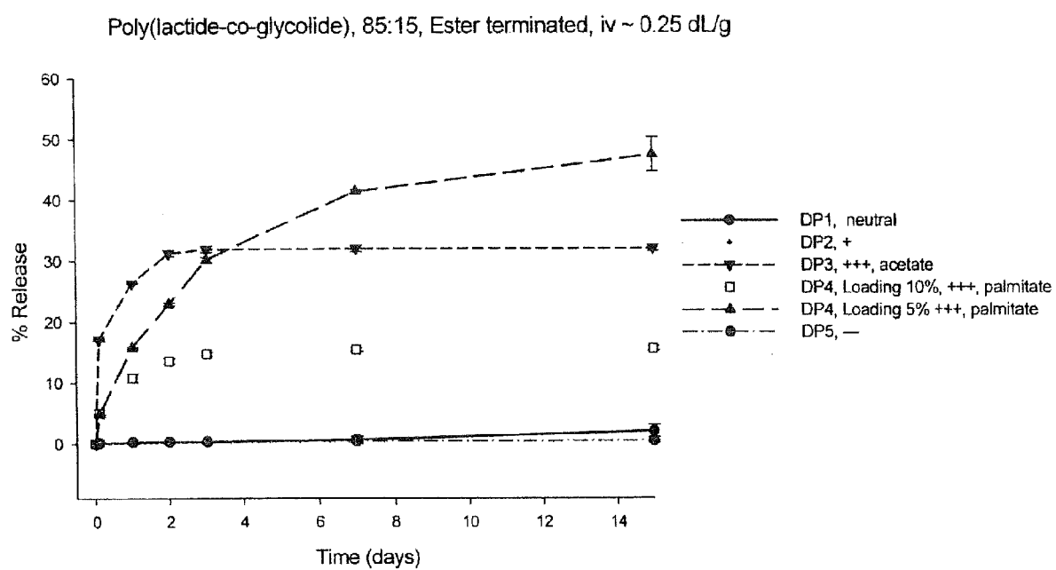
Figure 10: In vitro release rate, PLG 85:15 2E through 15 days
