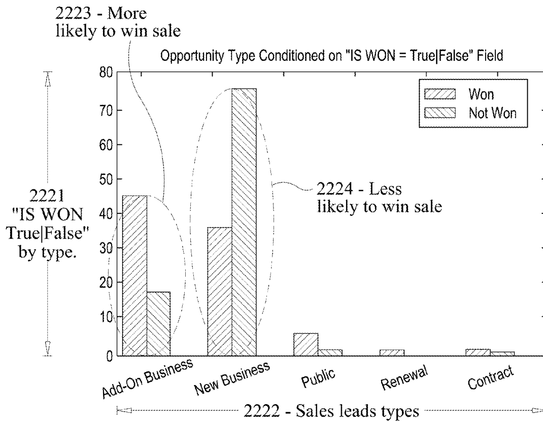
FIG. 22B Predictive Relationships for Opportunity Scoring
