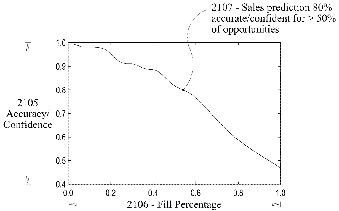
FIG. 21A Completeness vs. Accuracy
