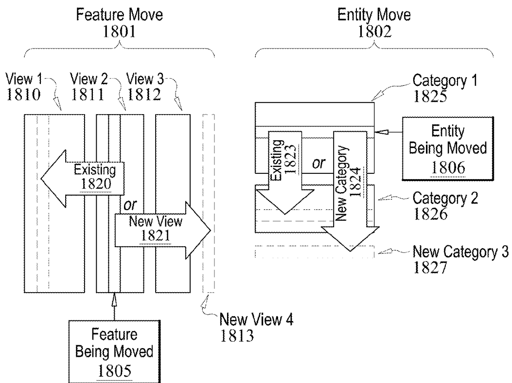
FIG. 18 Feature and Entity Moves Method
