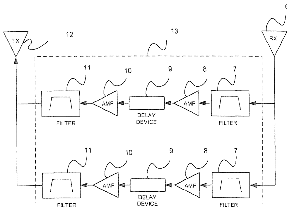
PRESENT INVENTION – DUAL BAND
