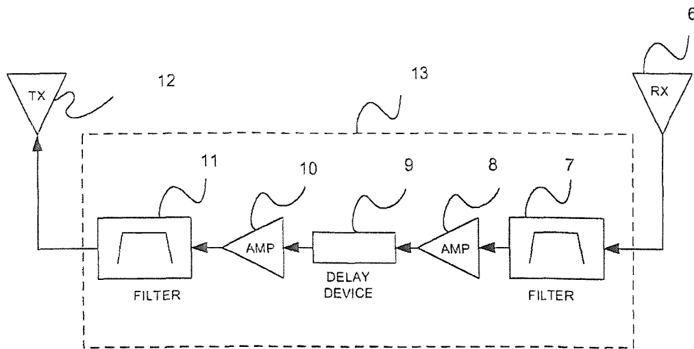
PRESENT INVENTION – SINGLE BAND
