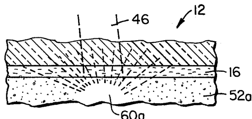
FIG. 4. PRIOR ART
