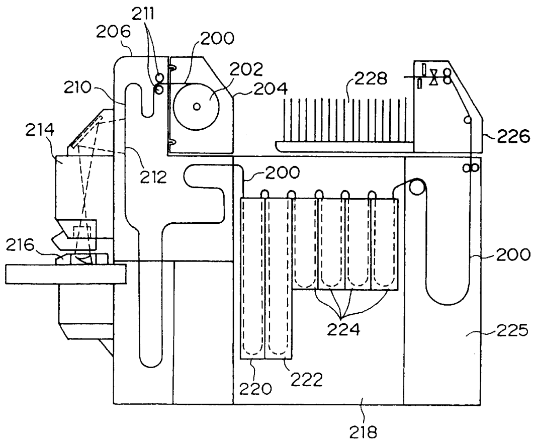
FIG. 7 PRIOR ART
