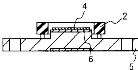
Fig. 2C PRIOR ART
