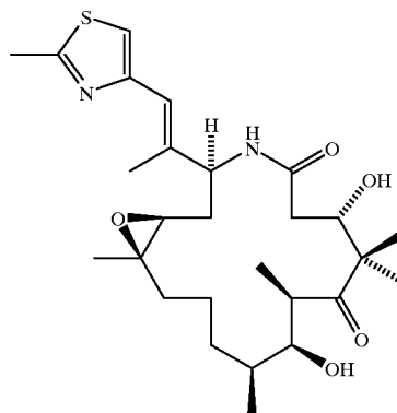
Preparation of 2
