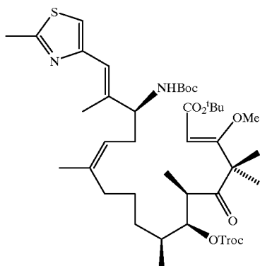
Preparation of 18
