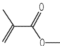
METHYLMETHACRYLATE
