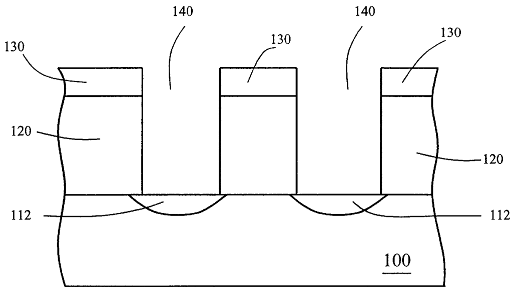
FIG. 1C (PRIOR ART)
