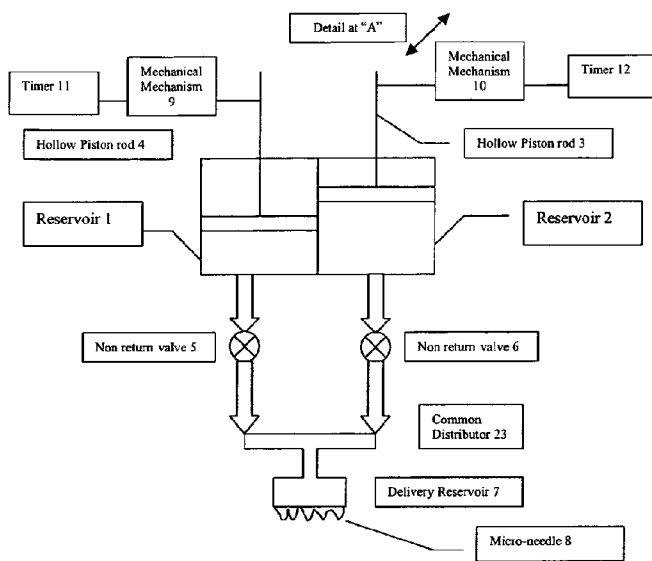
FIGURE 1 MECHANISM FOR PROGRAMMED DELIVERY OF BIOLOGICAL MATERIAL
