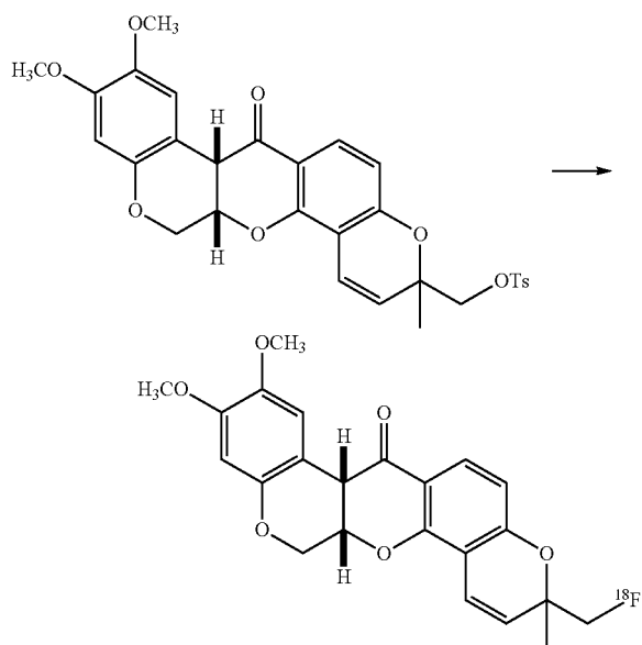
Synthesis of (6aS,12aS)-7'-[ 18 F]fluorodeguelin
