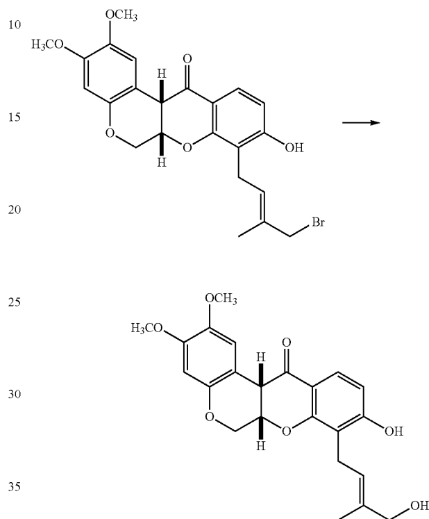
Synthesis of 4'-hydroxy-rot-2'-enonic acid
