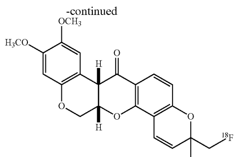
Synthesis of (6aS,12aS)-7'-[ 18 F]fluorodeguelin
