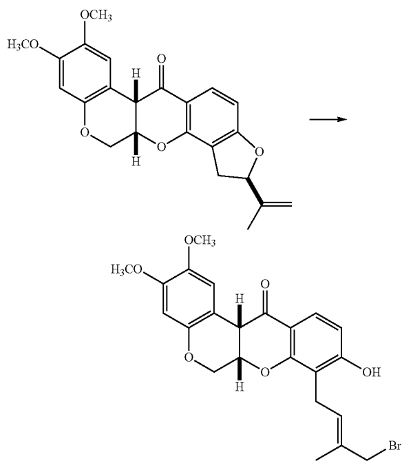
Synthesis of 4'-bromo-rot-2'-enonic acid
